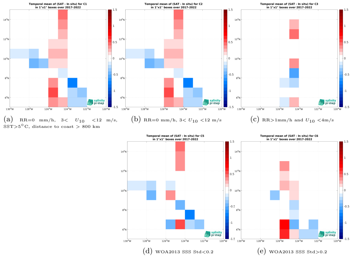
Figure 12: Temporal mean gridded over spatial boxes of size 1^\circ \times 1^\circ of \Delta SSS (SMAP SSS L3 v5 - 8-Day running (RSS) - Sairdrone) for 5 different subdatasets corresponding to:RR=0 mm/h, 3 < U_{10} < 12 m/s, SST >5^\circ\text{C} , distance to coast > 800 km (a), RR=0 mm/h, 3 < U_{10} < 12 m/s (b), RR >1 mm/h and U_{10} < 4 m/s (c), WOA2013 SSS Std <0.2 (d), WOA2013 SSS Std >0.2 (e).
