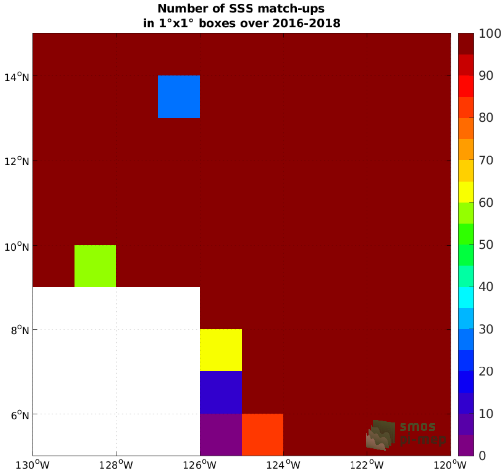
Figure 3: Number of SSS match-ups between Surface drifters SSS and the SMAP SSS L3 v5 - 8-Day running (RSS) SSS product for the SPURS 2 Pi-MEP region over 1°x1° boxes and for the full satellite product period.
