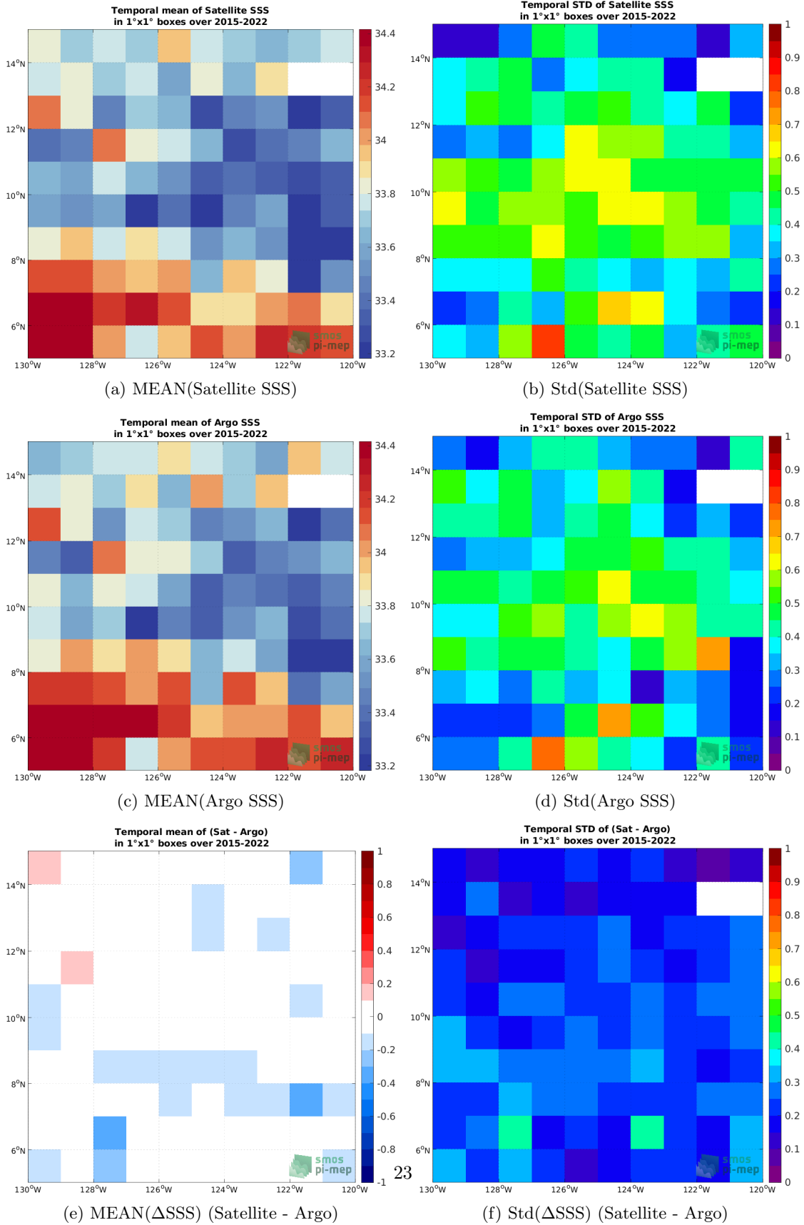
Figure 6: Temporal mean (left) and Std (right) of SSS from SMAP SSS L3 v5 - 8-Day running (RSS) (top), Argo (middle), and of \Delta SSS (Satellite - Argo). Only match-up pairs are used to generate these maps.
