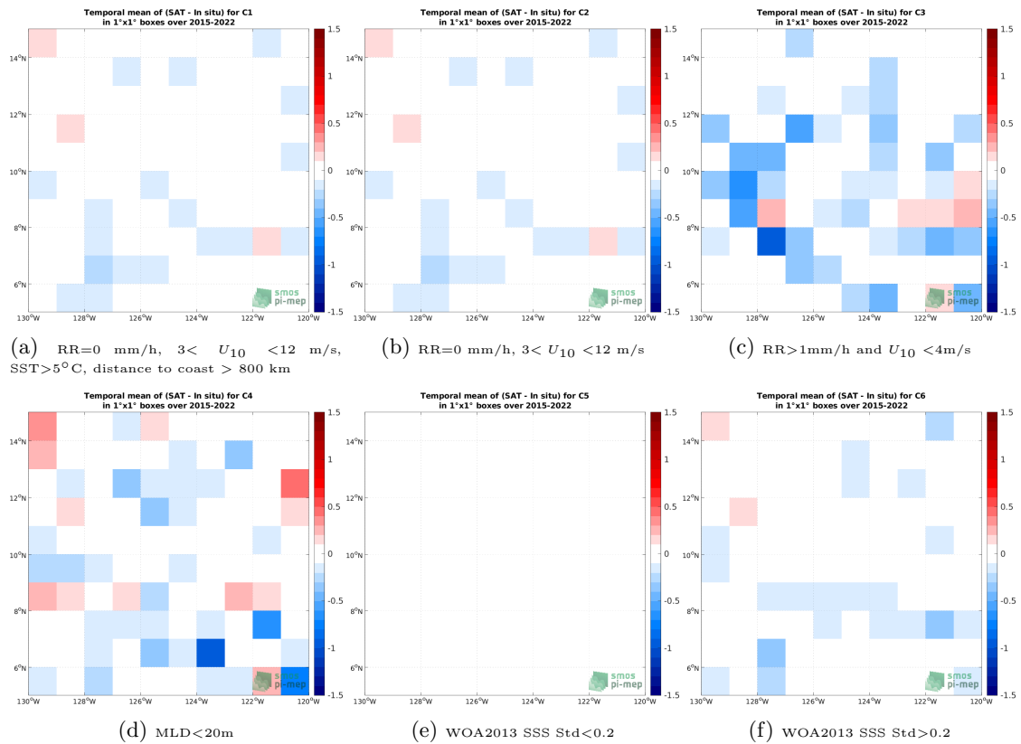
Figure 12: Temporal mean gridded over spatial boxes of size 1^\circ \times 1^\circ of \Delta SSS (SMAP SSS L3 v5 - 8-Day running (RSS) - Argo) for 6 different subdatasets corresponding to:RR=0 mm/h, 3 < U_{10} < 12 m/s, SST >5^\circ C, distance to coast > 800 km (a), RR=0 mm/h, 3 < U_{10} < 12 m/s (b), RR >1 mm/h and U_{10} < 4 m/s (c),MLD <20 m (d),WOA2013 SSS Std <0.2 (e),WOA2013 SSS Std >0.2 (f).
