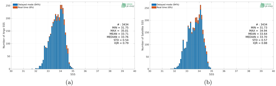
Figure 2: Histograms of SSS from Argo (a) and SMAP SSS L3 v5 - 8-Day running (RSS) (b) considering all match-up pairs per bins of 0.1 over the SPURS 2 Pi-MEP region and for the full satellite product period.
