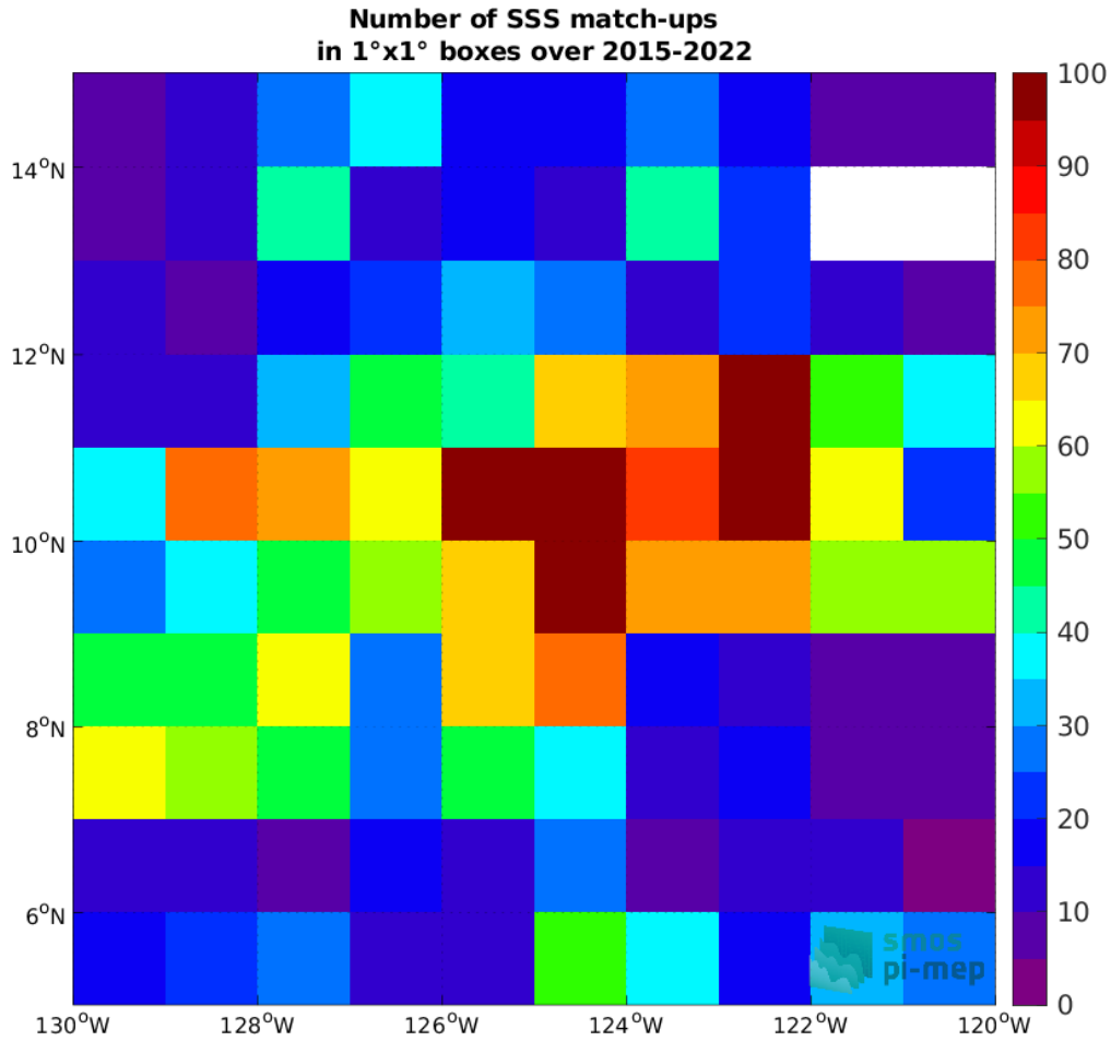
Figure 4: Number of SSS match-ups between Argo SSS and the SMAP SSS L3 v5 - 8-Day running (RSS) SSS product for the SPURS 2 Pi-MEP region over 1°x1° boxes and for the full satellite product period.
