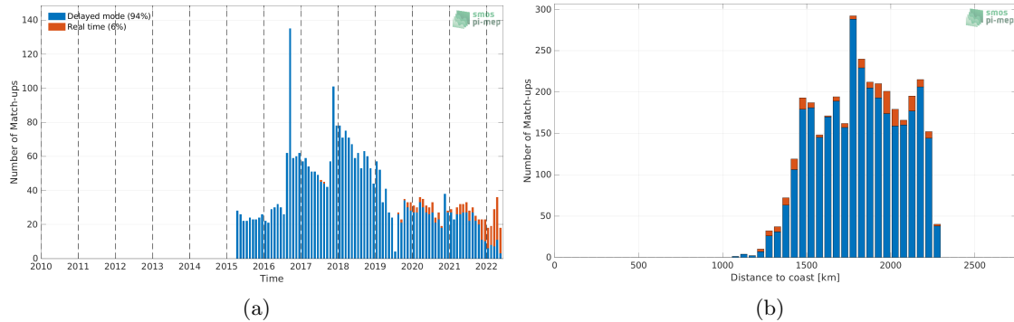
Figure 1: Number of match-ups between Argo and SMAP SSS L3 v5 - 8-Day running (RSS) SSS as a function of time (a) and as function of the distance to coast (b) over the SPURS 2 Pi-MEP region and for the full satellite product period.
