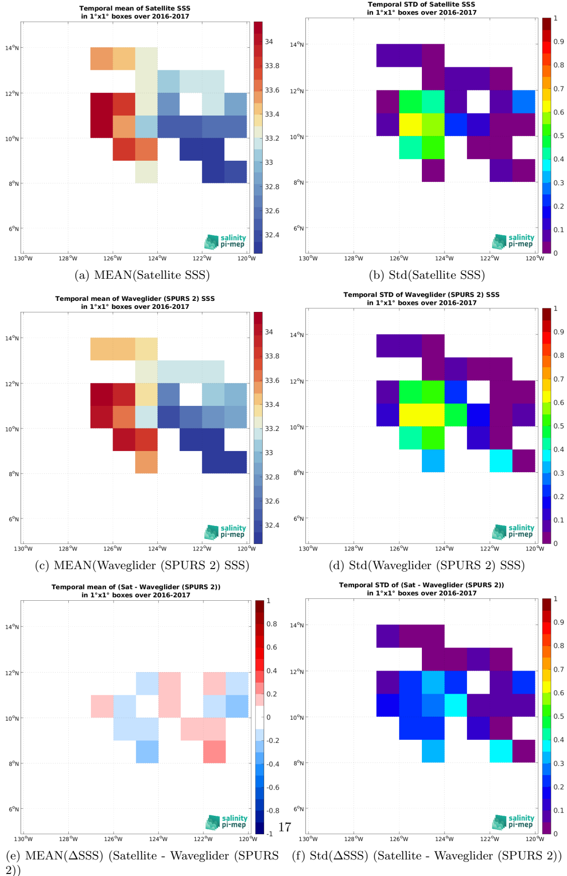
Figure 6: Temporal mean (left) and Std (right) of SSS from SMAP SSS L3 v5 - Monthly (RSS) (top), Waveglider (SPURS 2) (middle), and of \Delta SSS (Satellite - Waveglider (SPURS 2)). Only match-up pairs are used to generate these maps.
