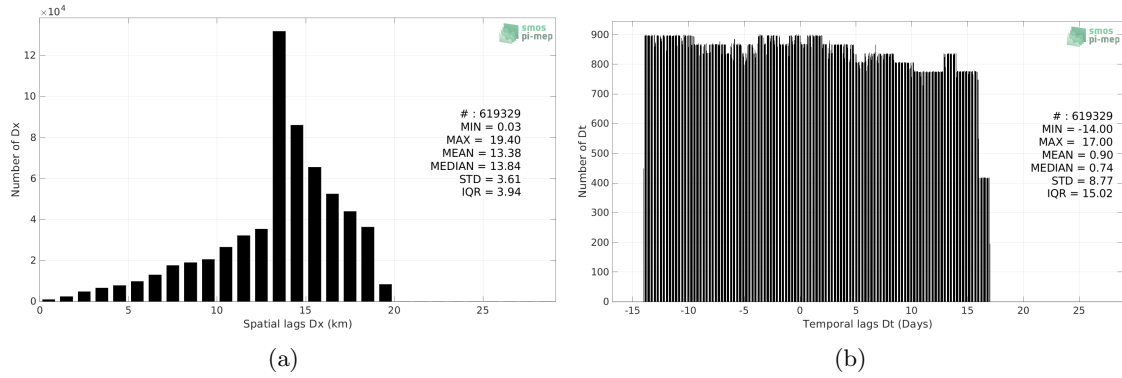
Figure 5: Histograms of the spatial (a) and temporal (b) lags between the location/time of the Waveglider (SPURS 2) measurement and the date of the corresponding SMAP SSS L3 v5 - Monthly (RSS) SSS pixel.
