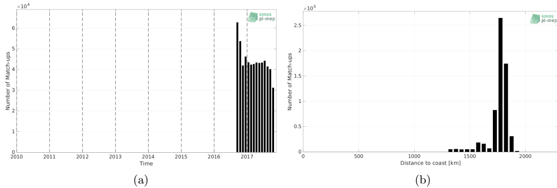
Figure 1: Number of match-ups between Waveglider (SPURS 2) and SMAP SSS L3 v5 - Monthly (RSS) SSS as a function of time (a) and as function of the distance to coast (b) over the SPURS 2 Pi-MEP region and for the full satellite product period.
