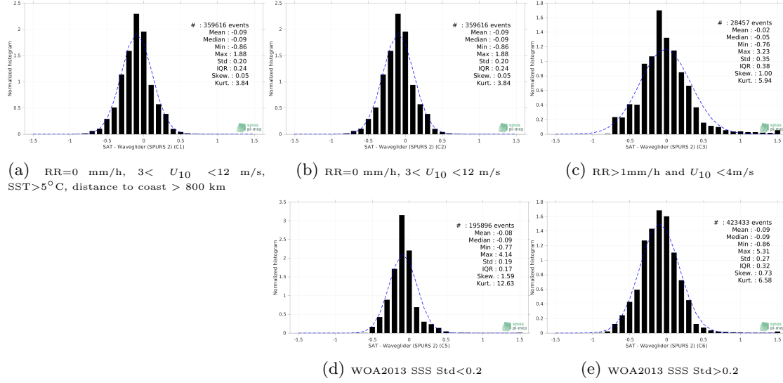
Figure 13: Normalized histogram of \Delta SSS (SMAP SSS L3 v5 - Monthly (RSS) - Waveglider (SPURS 2)) for 5 different subdatasets corresponding to: RR=0 mm/h, 3 < U_{10} < 12 m/s, SST>5°C, distance to coast > 800 km (a), RR=0 mm/h, 3 < U_{10} < 12 m/s (b), RR>1mm/h and U_{10} < 4 m/s (c), WOA2013 SSS Std<0.2 (d), WOA2013 SSS Std>0.2 (e).
