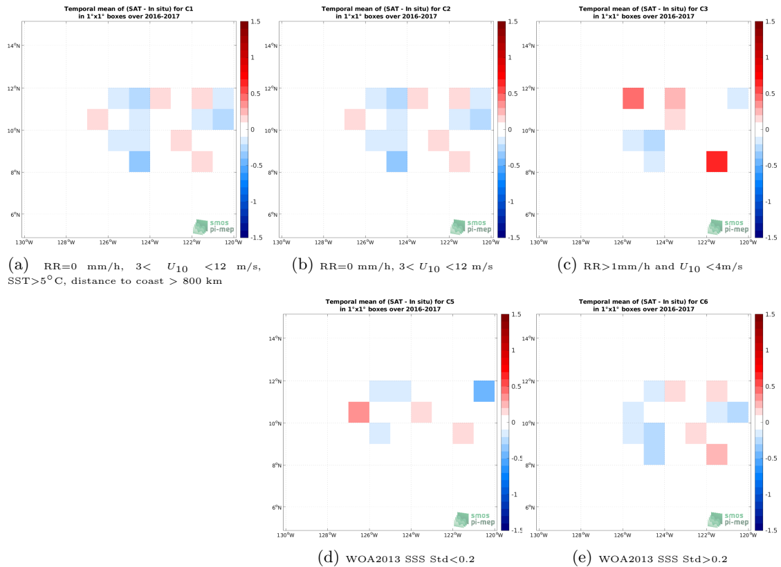
Figure 12: Temporal mean gridded over spatial boxes of size 1^\circ \times 1^\circ of \Delta SSS (SMAP SSS L3 v5 - Monthly (RSS) - Waveglider (SPURS 2)) for 5 different subdatasets corresponding to:RR=0 mm/h, 3 < U_{10} < 12 m/s, SST >5^\circ\text{C} , distance to coast > 800 km (a), RR=0 mm/h, 3 < U_{10} < 12 m/s (b), RR >1 mm/h and U_{10} < 4 m/s (c), WOA2013 SSS Std <0.2 (d), WOA2013 SSS Std >0.2 (e).
