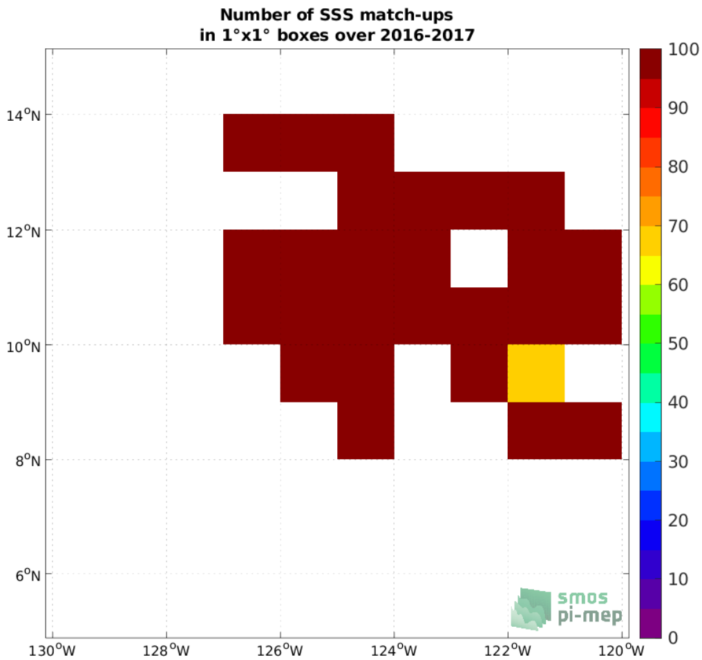
Figure 4: Number of SSS match-ups between Waveglider (SPURS 2) SSS and the SMAP SSS L3 v5 - Monthly (RSS) SSS product for the SPURS 2 Pi-MEP region over 1°x1° boxes and for the full satellite product period.
