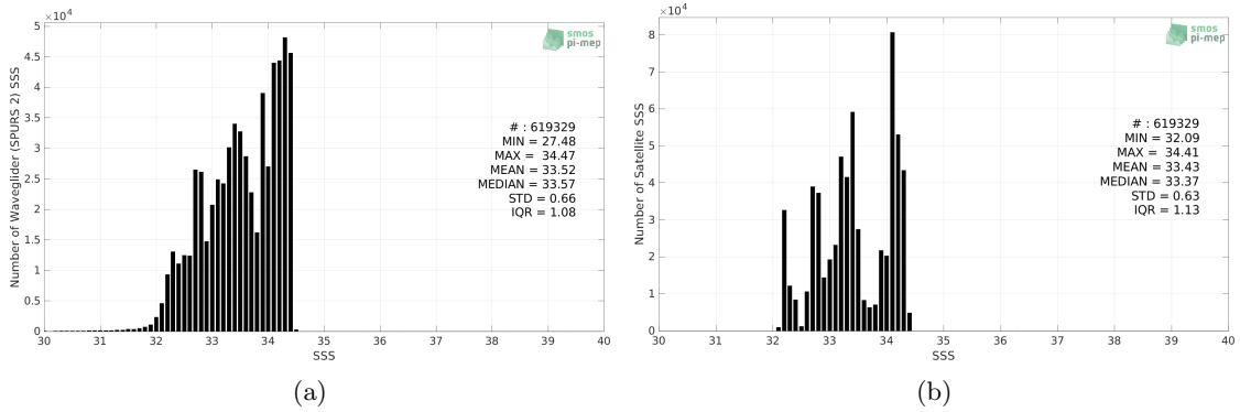
Figure 2: Histograms of SSS from Waveglider (SPURS 2) (a) and SMAP SSS L3 v5 - Monthly (RSS) (b) considering all match-up pairs per bins of 0.1 over the SPURS 2 Pi-MEP region and for the full satellite product period.
