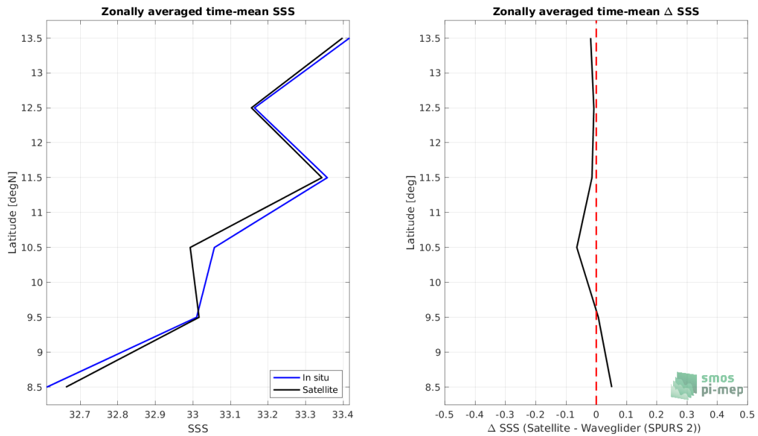
Figure 8: Left panel: Zonal mean SSS from SMAP SSS L3 v5 - Monthly (RSS) satellite product (black) and from Waveglider (SPURS 2) (blue). Right panel: Zonal mean of \Delta SSS (Satellite - Waveglider (SPURS 2)) for all the collected Pi-MEP match-up pairs estimated over the full satellite product period.
