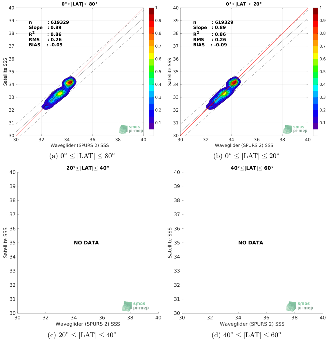
Figure 9: Contour maps of the concentration of SMAP SSS L3 v5 - Monthly (RSS) SSS (y-axis) versus Waveglider (SPURS 2) SSS (x-axis) at match-up pairs for different latitude bands. For each plot, the red line shows x=y . The black thin and dashed lines indicate a linear fit through the data cloud and the \pm 95\% confidence levels, respectively. The number match-up pairs n , the slope and R^2 coefficient of the linear fit, the root mean square (RMS) and the mean bias between satellite and in situ data are indicated for each latitude band in each plots.
