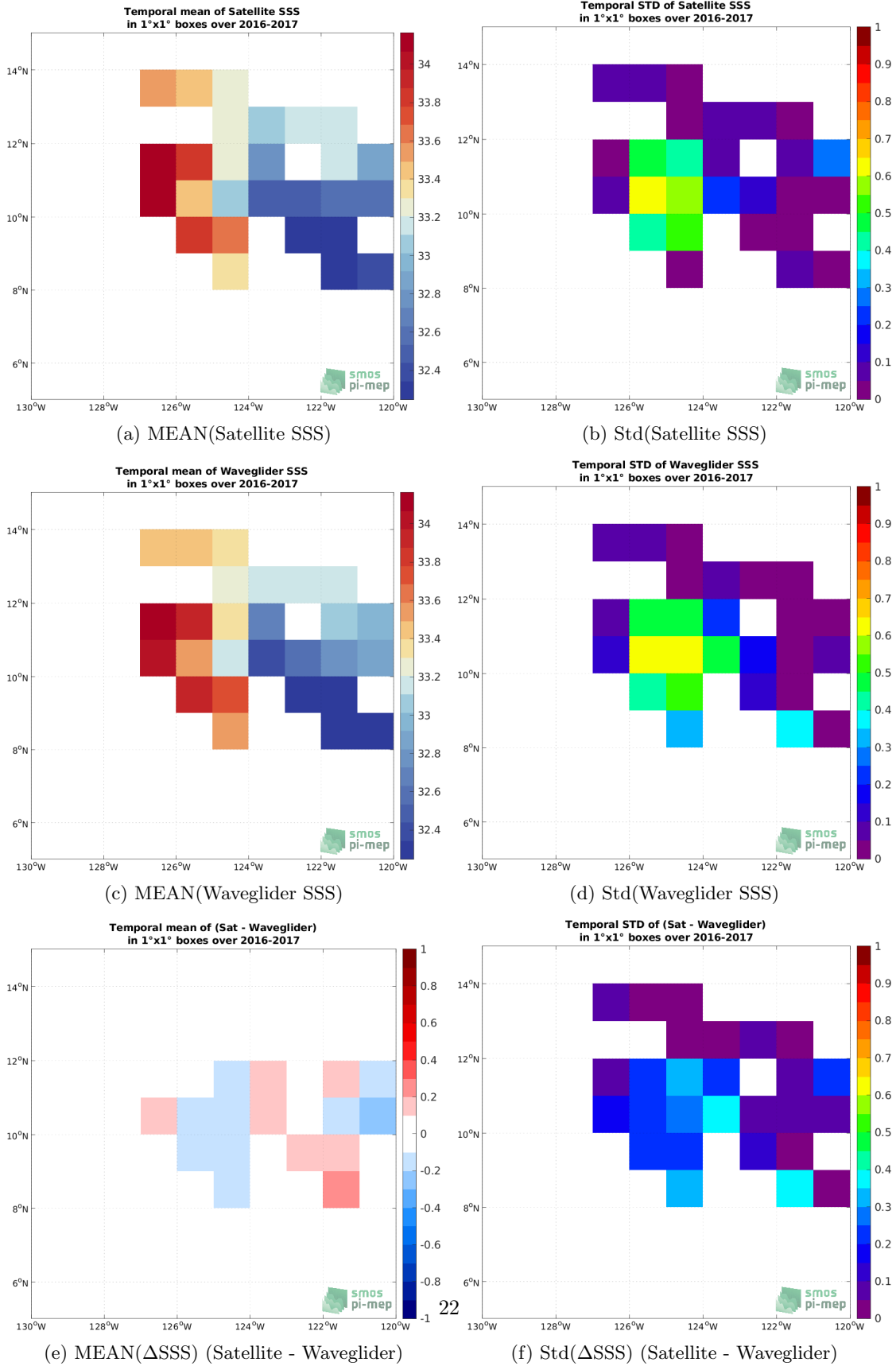
Figure 5: Temporal mean (left) and Std (right) of SSS from SMAP SSS L3 v5 - Monthly (RSS) (top), Waveglider (middle), and of \Delta SSS (Satellite - Waveglider). Only match-up pairs are used to generate these maps.
