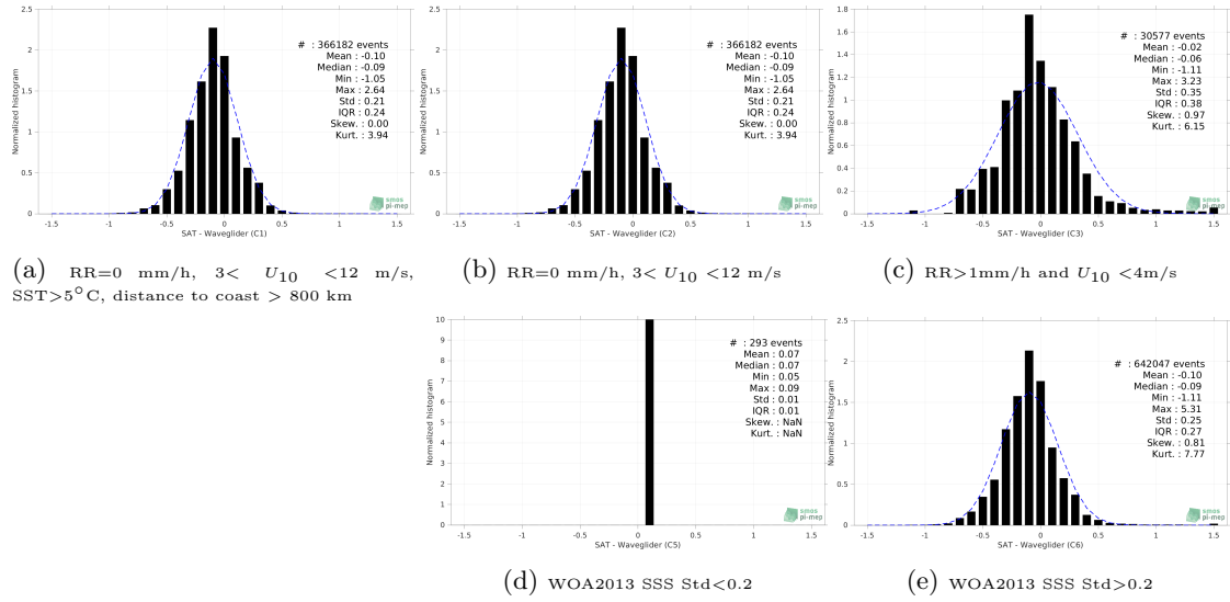
Figure 12: Normalized histogram of \Delta SSS (SMAP SSS L3 v5 - Monthly (RSS) - Waveglider) for 5 different subdatasets corresponding to: RR=0 mm/h, 3 < U_{10} < 12 m/s, SST > 5°C, distance to coast > 800 km (a), RR=0 mm/h, 3 < U_{10} < 12 m/s (b), RR > 1mm/h and U_{10} < 4 m/s (c), WOA2013 SSS Std < 0.2 (d), WOA2013 SSS Std > 0.2 (e).
