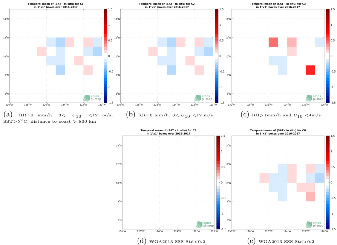
Figure 11: Temporal mean gridded over spatial boxes of size 1^\circ \times 1^\circ of \Delta SSS (SMAP SSS L3 v5 - Monthly (RSS) - Waveglider) for 5 different subdatasets corresponding to:RR=0 mm/h, 3 < U_{10} < 12 m/s, SST > 5^\circ\text{C} , distance to coast > 800 km (a), RR=0 mm/h, 3 < U_{10} < 12 m/s (b), RR > 1 mm/h and U_{10} < 4 m/s (c), WOA2013 SSS Std < 0.2 (d), WOA2013 SSS Std > 0.2 (e).
