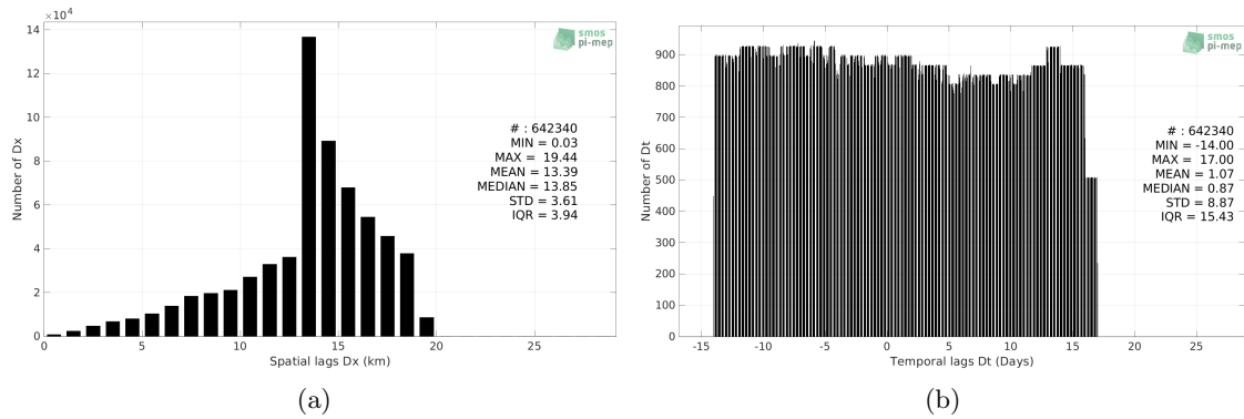
Figure 4: Histograms of the spatial (a) and temporal (b) lags between the location/time of the Waveglider measurement and the date of the corresponding SMAP SSS L3 v5 - Monthly (RSS) SSS pixel.
