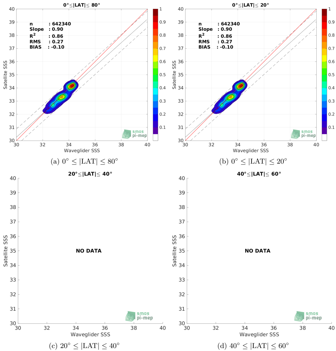
Figure 8: Contour maps of the concentration of SMAP SSS L3 v5 - Monthly (RSS) SSS (y-axis) versus Waveglider SSS (x-axis) at match-up pairs for different latitude bands. For each plot, the red line shows x=y . The black thin and dashed lines indicate a linear fit through the data cloud and the \pm 95\% confidence levels, respectively. The number match-up pairs n , the slope and R^2 coefficient of the linear fit, the root mean square (RMS) and the mean bias between satellite and in situ data are indicated for each latitude band in each plots.
