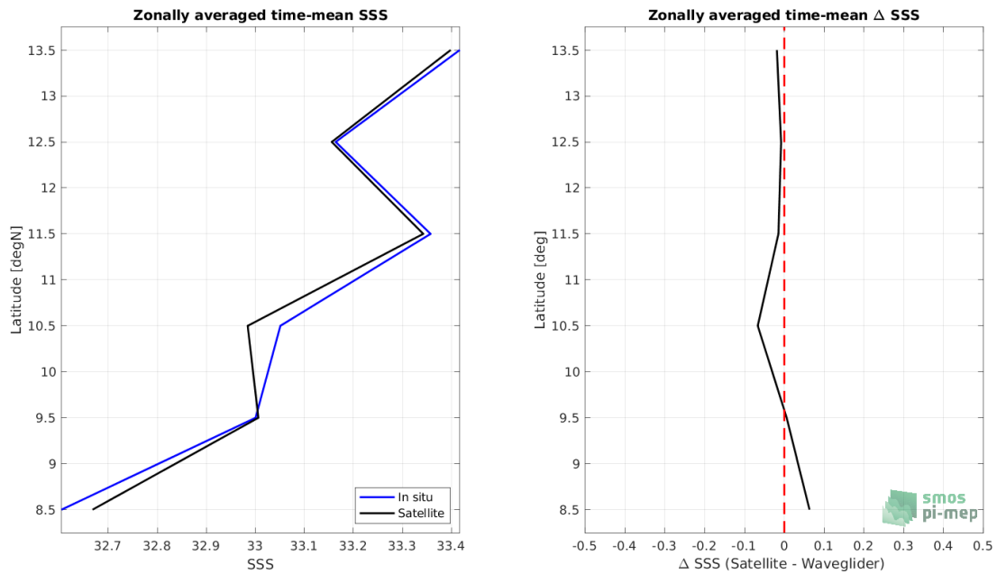
Figure 7: Left panel: Zonal mean SSS from SMAP SSS L3 v5 - Monthly (RSS) satellite product (black) and from Waveglider (blue). Right panel: Zonal mean of \Delta SSS (Satellite - Waveglider) for all the collected Pi-MEP match-up pairs estimated over the full satellite product period.
