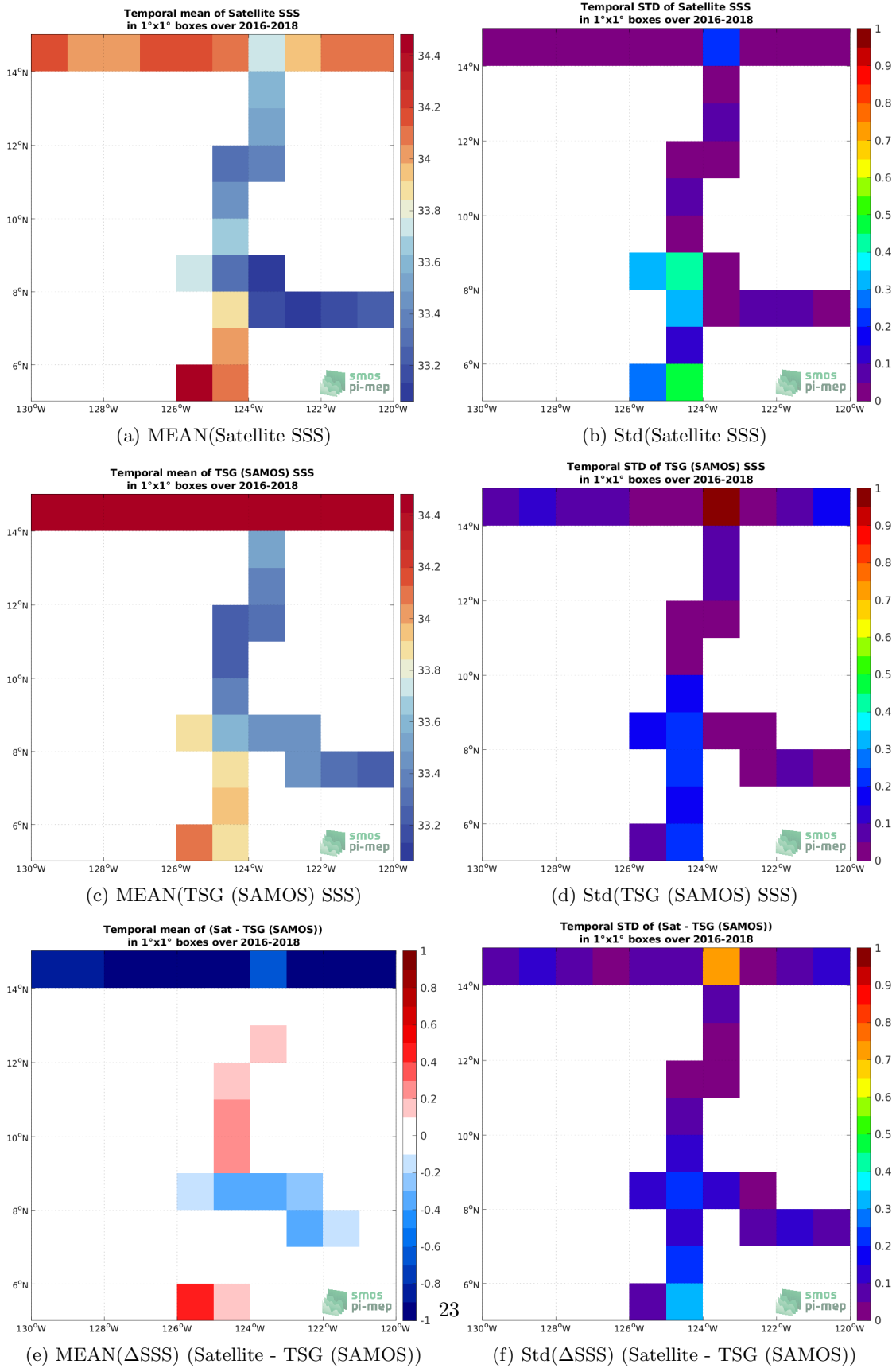
Figure 6: Temporal mean (left) and Std (right) of SSS from SMAP SSS L3 v5 - Monthly (RSS) (top), TSG (SAMOS) (middle), and of \Delta SSS (Satellite - TSG (SAMOS)). Only match-up pairs are used to generate these maps.
