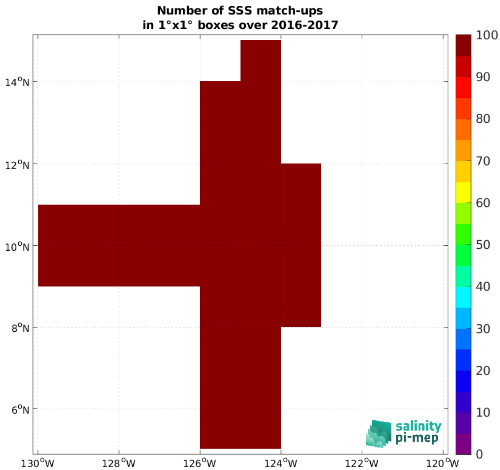
Figure 4: Number of SSS match-ups between Salinity Snake (SPURS 2) SSS and the SMAP SSS L3 v5 - Monthly (RSS) SSS product for the SPURS 2 Pi-MEP region over 1^\circ \times 1^\circ boxes and for the full satellite product period.
