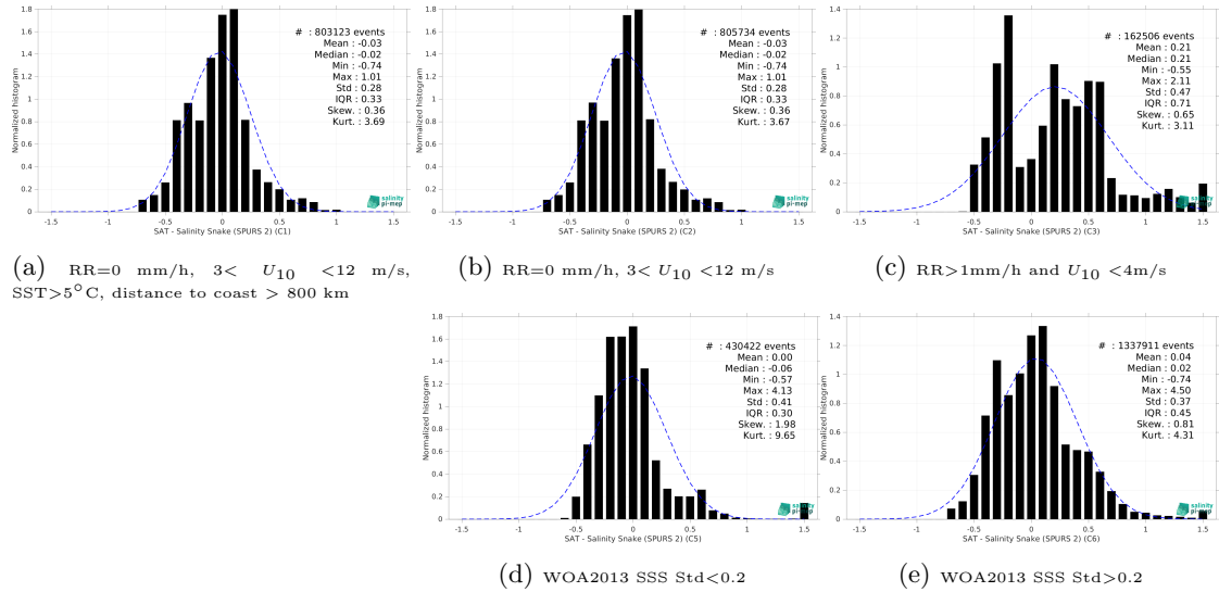
Figure 13: Normalized histogram of \Delta SSS (SMAP SSS L3 v5 - Monthly (RSS) - Salinity Snake (SPURS 2)) for 5 different subdatasets corresponding to: RR=0 mm/h, 3 < U_{10} < 12 m/s, SST > 5°C, distance to coast > 800 km (a), RR=0 mm/h, 3 < U_{10} < 12 m/s (b), RR > 1mm/h and U_{10} < 4 m/s (c), WOA2013 SSS Std < 0.2 (d), WOA2013 SSS Std > 0.2 (e).
