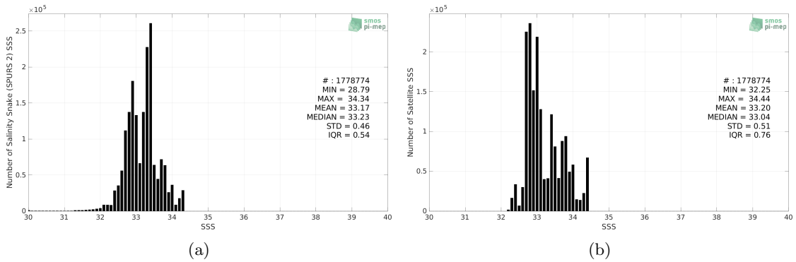
Figure 2: Histograms of SSS from Salinity Snake (SPURS 2) (a) and SMAP SSS L3 v5 - Monthly (RSS) (b) considering all match-up pairs per bins of 0.1 over the SPURS 2 Pi-MEP region and for the full satellite product period.
