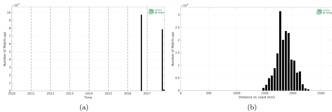
Figure 1: Number of match-ups between Salinity Snake (SPURS 2) and SMAP SSS L3 v5 - Monthly (RSS) SSS as a function of time (a) and as function of the distance to coast (b) over the SPURS 2 Pi-MEP region and for the full satellite product period.
