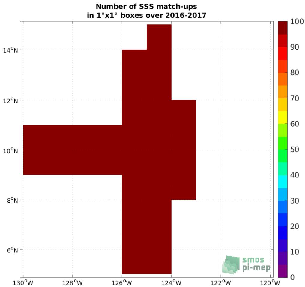
Figure 4: Number of SSS match-ups between Salinity Snake (SPURS 2) SSS and the SMAP SSS L3 v5 - Monthly (RSS) SSS product for the SPURS 2 Pi-MEP region over 1°x1° boxes and for the full satellite product period.
