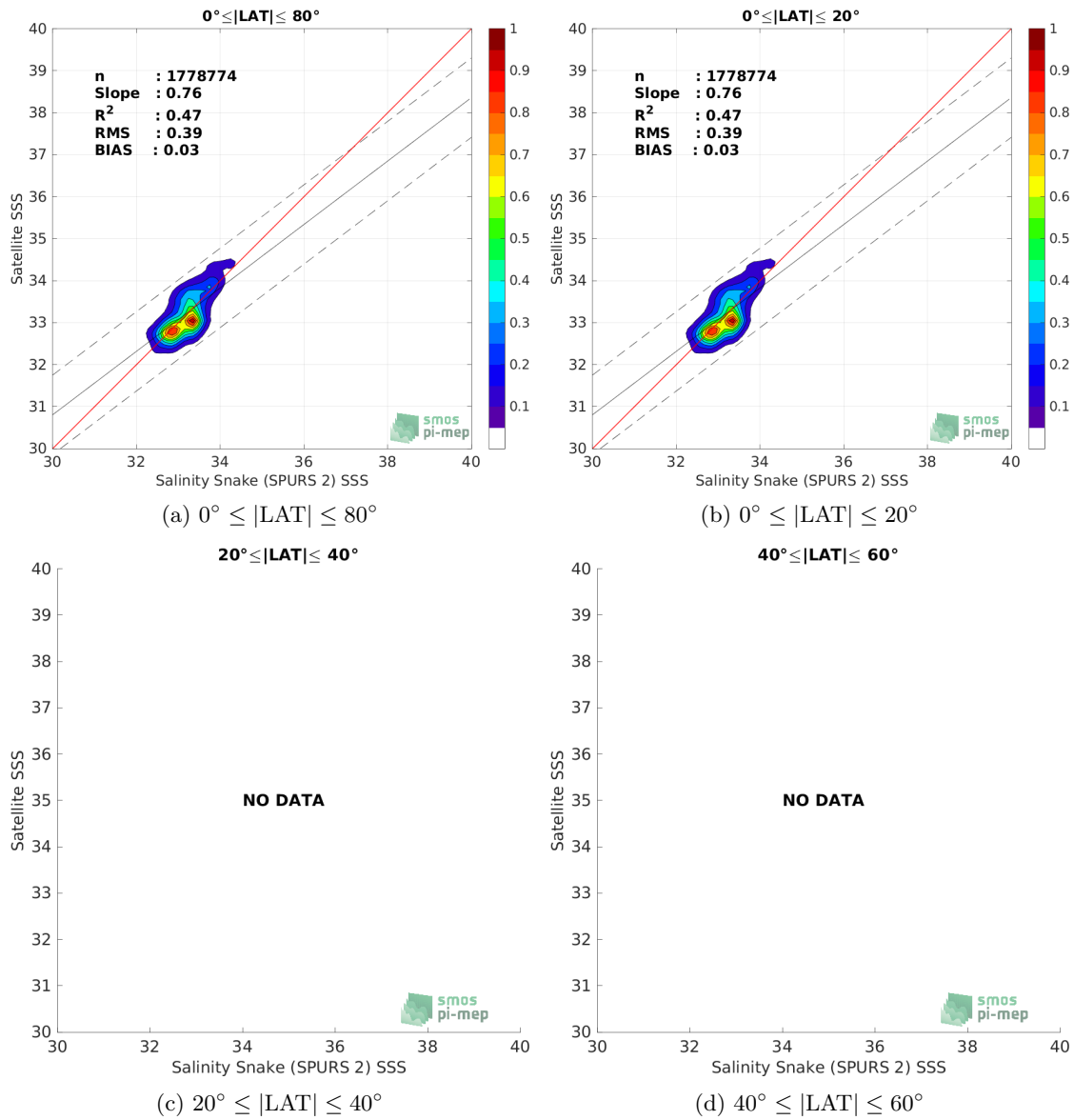
Figure 9: Contour maps of the concentration of SMAP SSS L3 v5 - Monthly (RSS) SSS (y-axis) versus Salinity Snake (SPURS 2) SSS (x-axis) at match-up pairs for different latitude bands. For each plot, the red line shows x=y . The black thin and dashed lines indicate a linear fit through the data cloud and the \pm 95\% confidence levels, respectively. The number match-up pairs n , the slope and R^2 coefficient of the linear fit, the root mean square (RMS) and the mean bias between satellite and in situ data are indicated for each latitude band in each plots.
