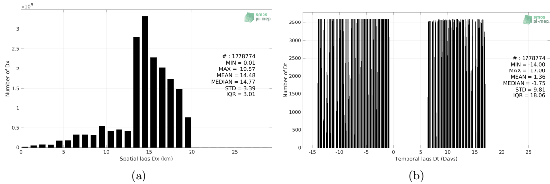
Figure 5: Histograms of the spatial (a) and temporal (b) lags between the location/time of the Salinity Snake (SPURS 2) measurement and the date of the corresponding SMAP SSS L3 v5 - Monthly (RSS) SSS pixel.
