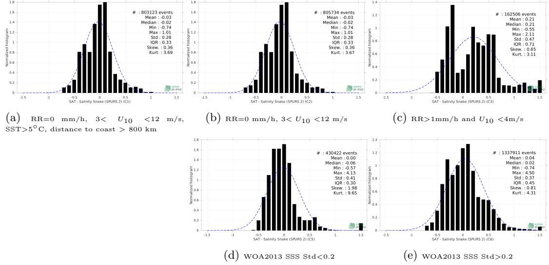
Figure 13: Normalized histogram of \Delta SSS (SMAP SSS L3 v5 - Monthly (RSS) - Salinity Snake (SPURS 2)) for 5 different subdatasets corresponding to: RR=0 mm/h, 3 < U_{10} < 12 m/s, SST > 5°C, distance to coast > 800 km (a), RR=0 mm/h, 3 < U_{10} < 12 m/s (b), RR > 1mm/h and U_{10} < 4 m/s (c), WOA2013 SSS Std < 0.2 (d), WOA2013 SSS Std > 0.2 (e).
