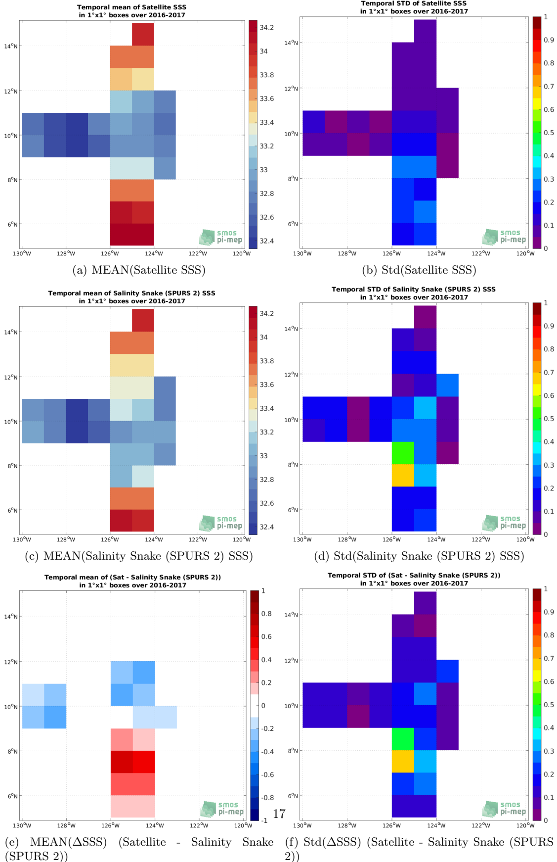
Figure 6: Temporal mean (left) and Std (right) of SSS from SMAP SSS L3 v5 - Monthly (RSS) (top), Salinity Snake (SPURS 2) (middle), and of \Delta SSS (Satellite - Salinity Snake (SPURS 2)). Only match-up pairs are used to generate these maps.
