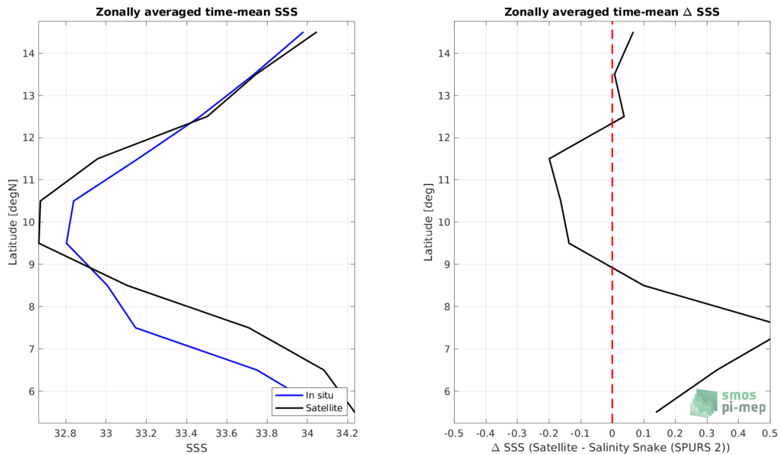
Figure 8: Left panel: Zonal mean SSS from SMAP SSS L3 v5 - Monthly (RSS) satellite product (black) and from Salinity Snake (SPURS 2) (blue). Right panel: Zonal mean of \Delta SSS (Satellite - Salinity Snake (SPURS 2)) for all the collected Pi-MEP match-up pairs estimated over the full satellite product period.
