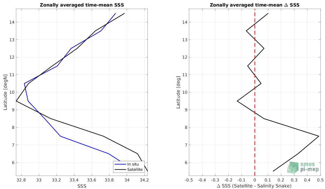
Figure 8: Left panel: Zonal mean SSS from SMAP SSS L3 v5 - Monthly (RSS) satellite product (black) and from Salinity Snake (blue). Right panel: Zonal mean of \Delta SSS (Satellite - Salinity Snake) for all the collected Pi-MEP match-up pairs estimated over the full satellite product period.
