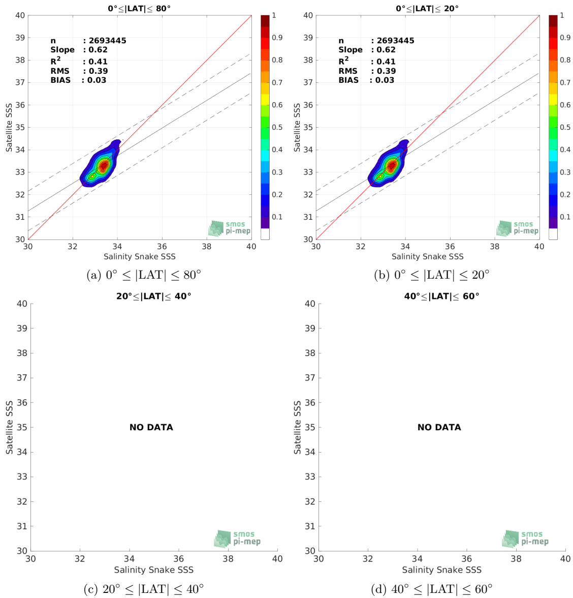
Figure 9: Contour maps of the concentration of SMAP SSS L3 v5 - Monthly (RSS) SSS (y-axis) versus Salinity Snake SSS (x-axis) at match-up pairs for different latitude bands. For each plot, the red line shows x=y . The black thin and dashed lines indicate a linear fit through the data cloud and the \pm 95\% confidence levels, respectively. The number match-up pairs n , the slope and R^2 coefficient of the linear fit, the root mean square (RMS) and the mean bias between satellite and in situ data are indicated for each latitude band in each plots.
