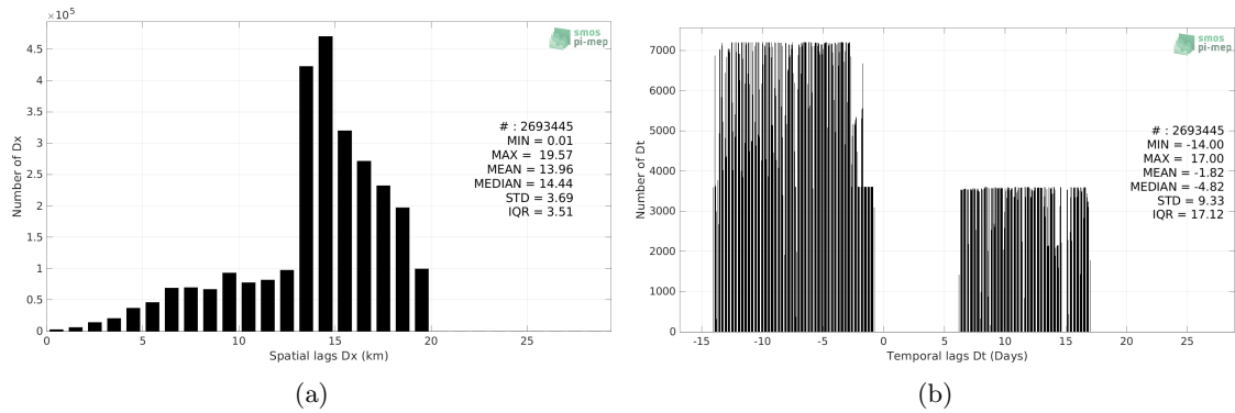
Figure 5: Histograms of the spatial (a) and temporal (b) lags between the location/time of the Salinity Snake measurement and the date of the corresponding SMAP SSS L3 v5 - Monthly (RSS) SSS pixel.
