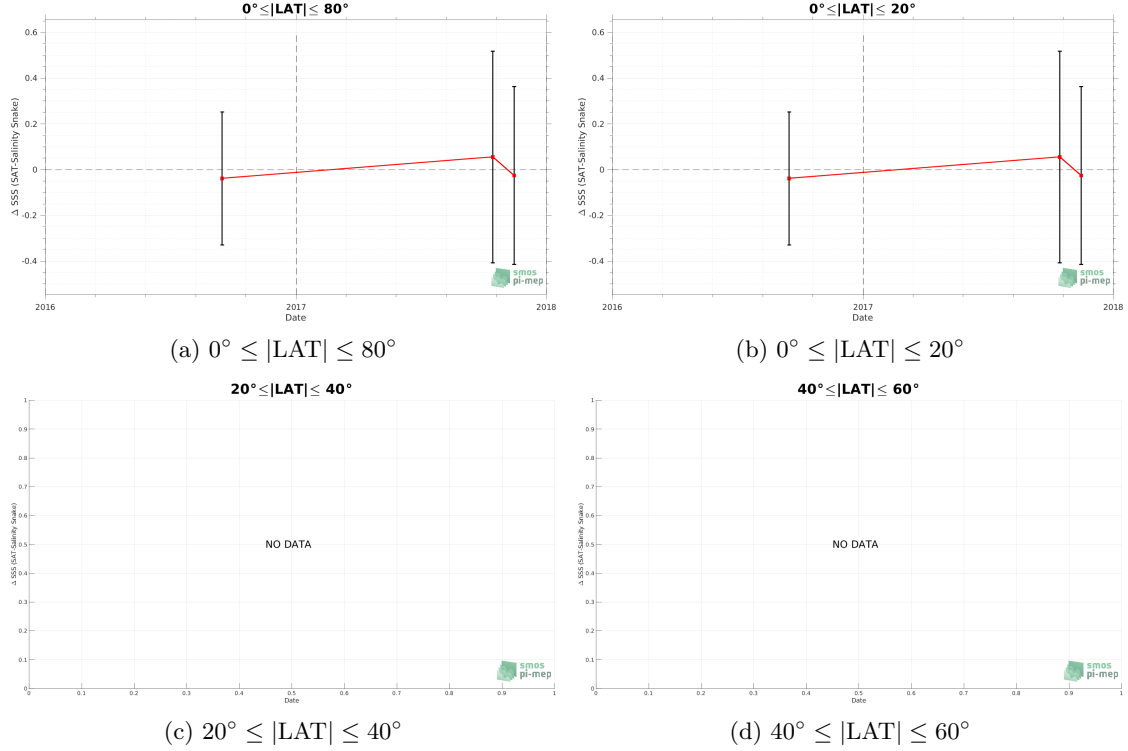
Figure 10: Monthly median (red curves) of \Delta SSS (Satellite - Salinity Snake) and \pm 1 Std (black vertical thick bars) as function of time for all the collected Pi-MEP match-up pairs estimated over the SPURS 2 Pi-MEP region and for the full satellite product period are shown for different latitude bands: (a) 80°S-80°N, (b) 20°S-20°N, (c) 40°S-20°S and 20°N-40°N and (d) 60°S-40°S and 40°N-60°N.
