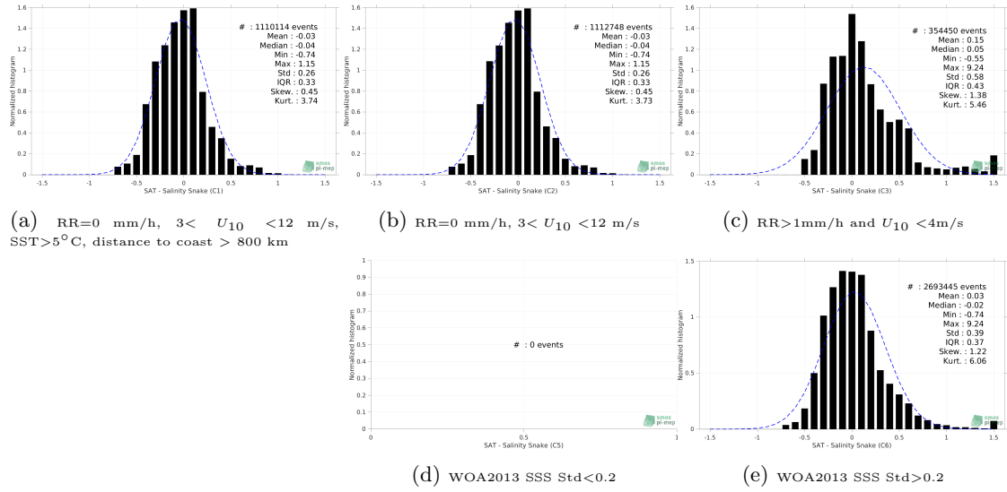
Figure 13: Normalized histogram of \Delta SSS (SMAP SSS L3 v5 - Monthly (RSS) - Salinity Snake) for 5 different subdatasets corresponding to: RR=0 mm/h, 3 < U_{10} < 12 m/s, SST > 5°C, distance to coast > 800 km (a), RR=0 mm/h, 3 < U_{10} < 12 m/s (b), RR > 1mm/h and U_{10} < 4 m/s (c), WOA2013 SSS Std < 0.2 (d), WOA2013 SSS Std > 0.2 (e).
