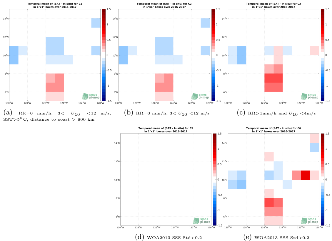
Figure 12: Temporal mean gridded over spatial boxes of size 1^\circ \times 1^\circ of \Delta SSS (SMAP SSS L3 v5 - Monthly (RSS) - Salinity Snake) for 5 different subdatasets corresponding to:RR=0 mm/h, 3 < U_{10} < 12 m/s, SST >5^\circ C, distance to coast > 800 km (a), RR=0 mm/h, 3 < U_{10} < 12 m/s (b), RR >1 mm/h and U_{10} < 4 m/s (c), WOA2013 SSS Std <0.2 (d), WOA2013 SSS Std >0.2 (e).
