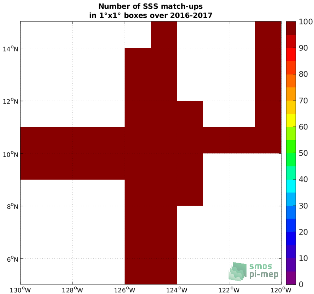
Figure 4: Number of SSS match-ups between Salinity Snake SSS and the SMAP SSS L3 v5 - Monthly (RSS) SSS product for the SPURS 2 Pi-MEP region over 1°x1° boxes and for the full satellite product period.
