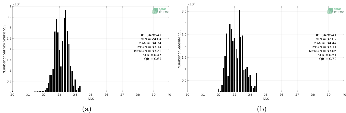
Figure 2: Histograms of SSS from Salinity Snake (a) and SMAP SSS L3 v5 - Monthly (RSS) (b) considering all match-up pairs per bins of 0.1 over the SPURS 2 Pi-MEP region and for the full satellite product period.
