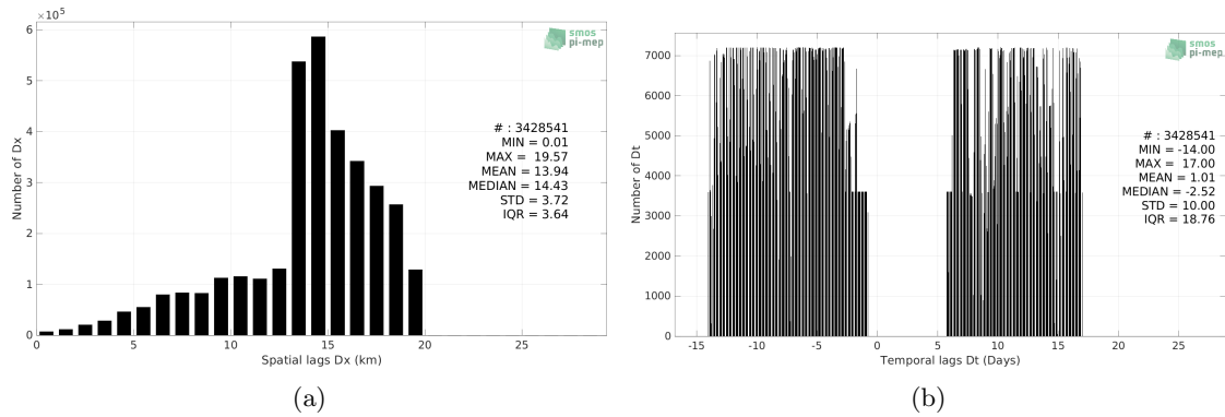
Figure 4: Histograms of the spatial (a) and temporal (b) lags between the location/time of the Salinity Snake measurement and the date of the corresponding SMAP SSS L3 v5 - Monthly (RSS) SSS pixel.
