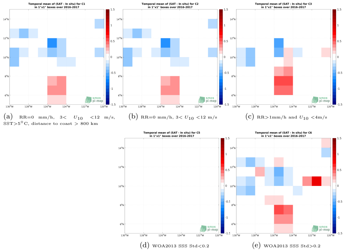
Figure 11: Temporal mean gridded over spatial boxes of size 1^\circ \times 1^\circ of \Delta SSS (SMAP SSS L3 v5 - Monthly (RSS) - Salinity Snake) for 5 different subdatasets corresponding to:RR=0 mm/h, 3 < U_{10} < 12 m/s, SST >5^\circ\text{C} , distance to coast > 800 km (a), RR=0 mm/h, 3 < U_{10} < 12 m/s (b), RR >1 mm/h and U_{10} < 4 m/s (c), WOA2013 SSS Std <0.2 (d), WOA2013 SSS Std >0.2 (e).
