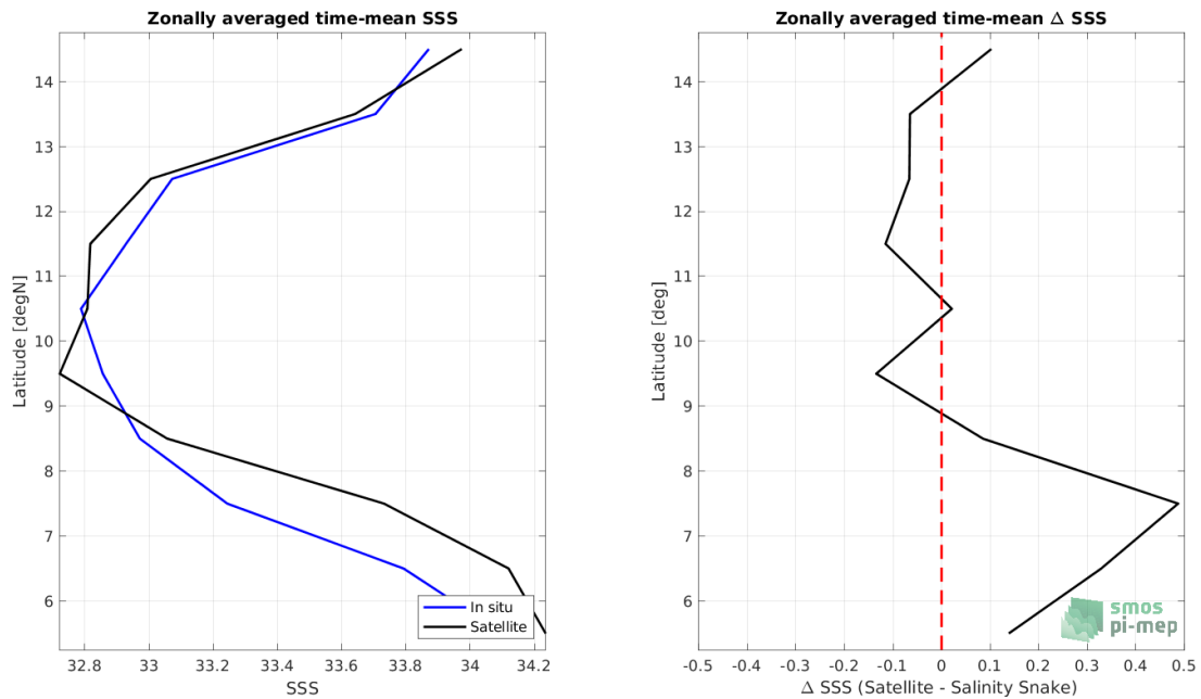
Figure 7: Left panel: Zonal mean SSS from SMAP SSS L3 v5 - Monthly (RSS) satellite product (black) and from Salinity Snake (blue). Right panel: Zonal mean of \Delta SSS (Satellite - Salinity Snake) for all the collected Pi-MEP match-up pairs estimated over the full satellite product period.
