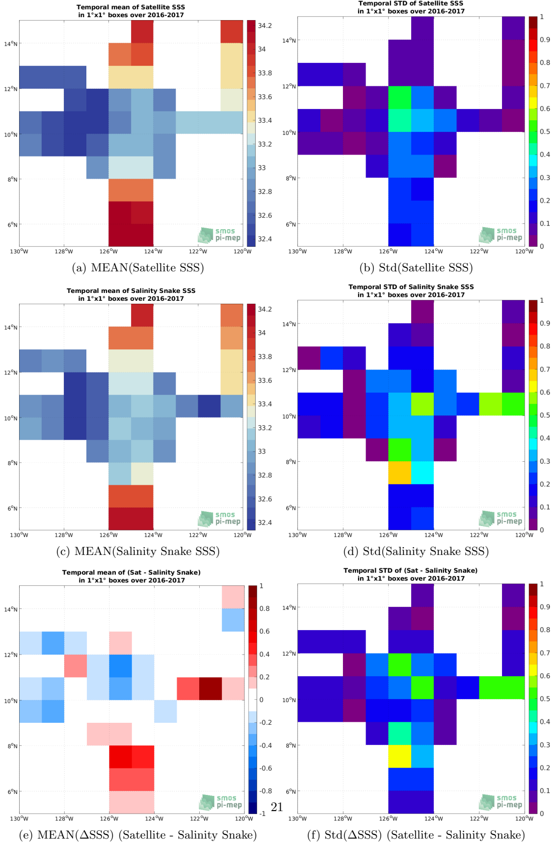
Figure 5: Temporal mean (left) and Std (right) of SSS from SMAP SSS L3 v5 - Monthly (RSS) (top), Salinity Snake (middle), and of \Delta SSS (Satellite - Salinity Snake). Only match-up pairs are used to generate these maps.
