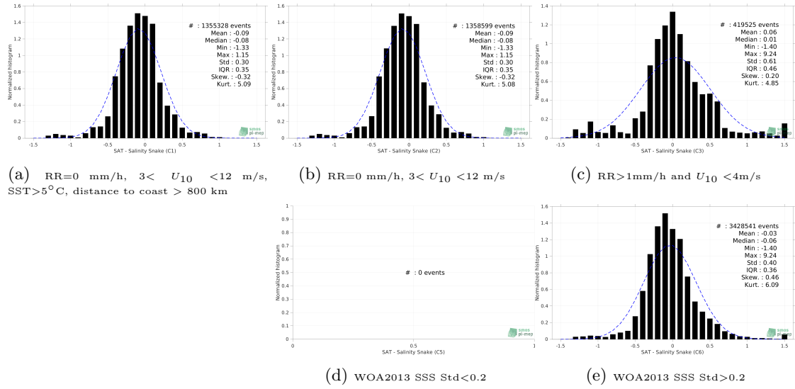
Figure 12: Normalized histogram of \Delta SSS (SMAP SSS L3 v5 - Monthly (RSS) - Salinity Snake) for 5 different subdatasets corresponding to: RR=0 mm/h, 3 < U_{10} < 12 m/s, SST>5°C, distance to coast > 800 km (a), RR=0 mm/h, 3 < U_{10} < 12 m/s (b), RR>1mm/h and U_{10} < 4 m/s (c), WOA2013 SSS Std<0.2 (d), WOA2013 SSS Std>0.2 (e).
