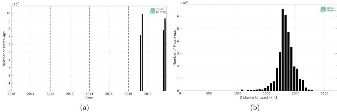
Figure 1: Number of match-ups between Salinity Snake and SMAP SSS L3 v5 - Monthly (RSS) SSS as a function of time (a) and as function of the distance to coast (b) over the SPURS 2 Pi-MEP region and for the full satellite product period.
