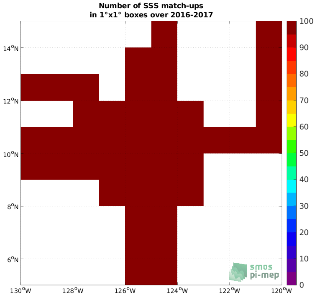
Figure 3: Number of SSS match-ups between Salinity Snake SSS and the SMAP SSS L3 v5 - Monthly (RSS) SSS product for the SPURS 2 Pi-MEP region over 1^\circ \times 1^\circ boxes and for the full satellite product period.
