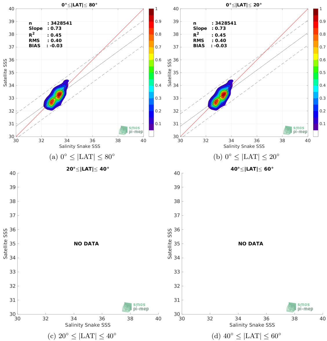
Figure 8: Contour maps of the concentration of SMAP SSS L3 v5 - Monthly (RSS) SSS (y-axis) versus Salinity Snake SSS (x-axis) at match-up pairs for different latitude bands. For each plot, the red line shows x=y . The black thin and dashed lines indicate a linear fit through the data cloud and the \pm 95\% confidence levels, respectively. The number match-up pairs n , the slope and R^2 coefficient of the linear fit, the root mean square (RMS) and the mean bias between satellite and in situ data are indicated for each latitude band in each plots.
