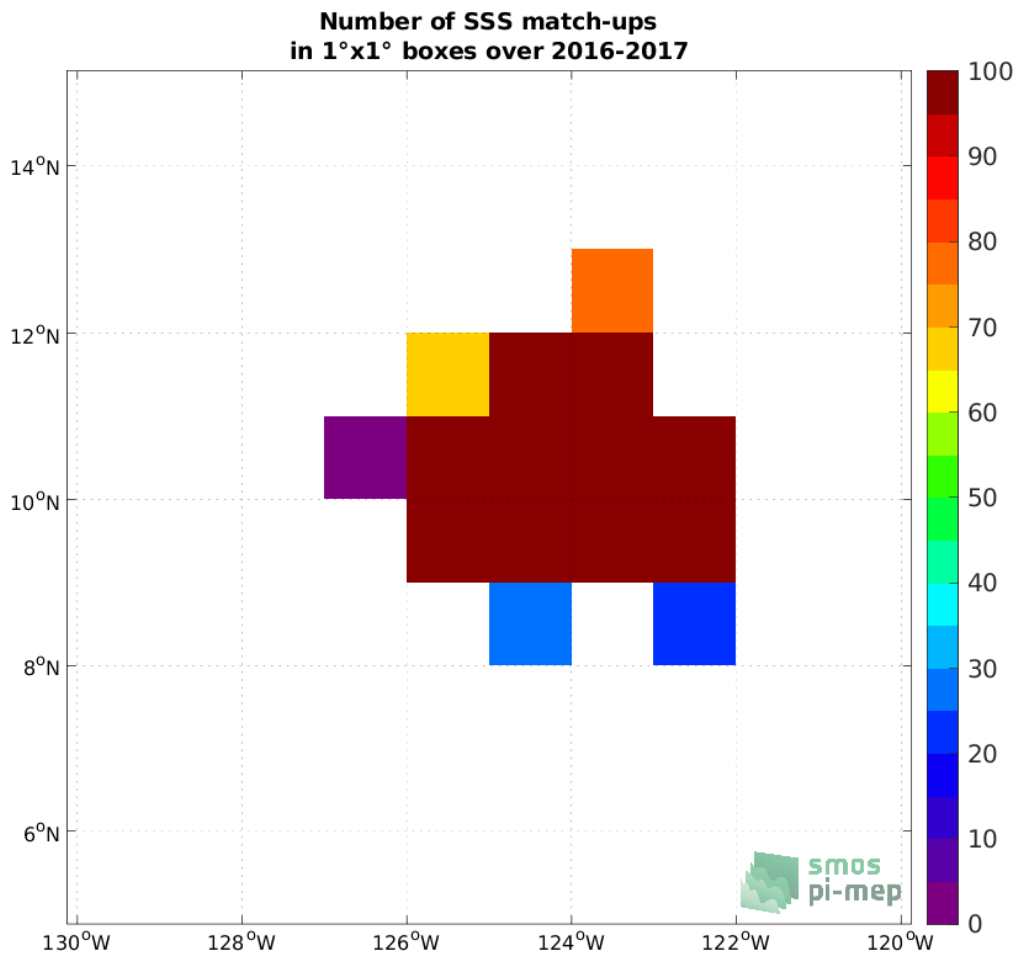
Figure 4: Number of SSS match-ups between Seaglider (SPURS 2) SSS and the SMAP SSS L3 v5 - Monthly (RSS) SSS product for the SPURS 2 Pi-MEP region over 1^\circ \times 1^\circ boxes and for the full satellite product period.
