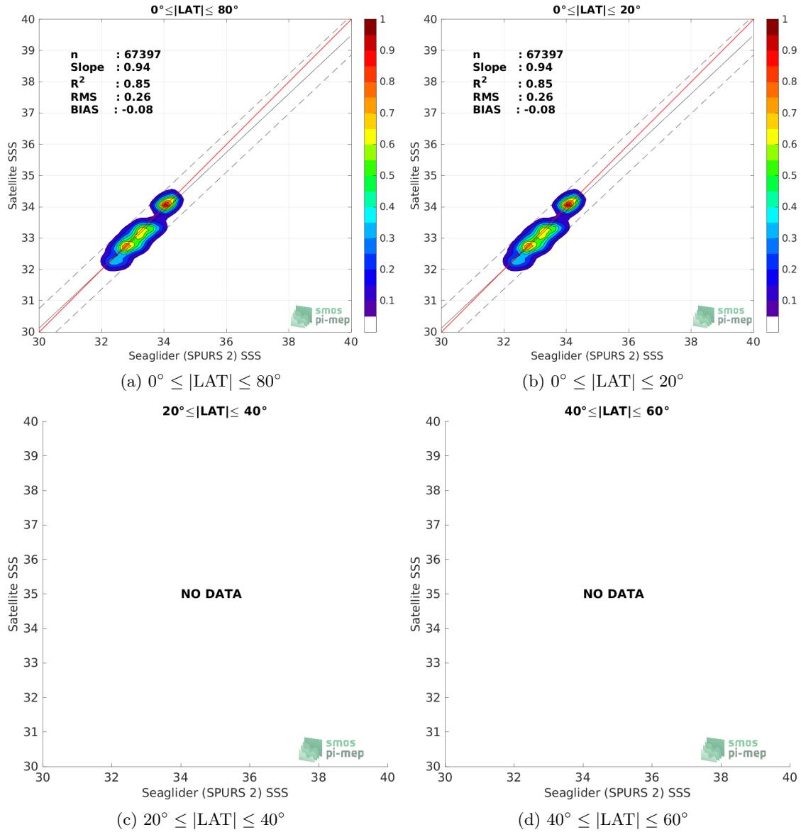
Figure 9: Contour maps of the concentration of SMAP SSS L3 v5 - Monthly (RSS) SSS (y-axis) versus Seaglider (SPURS 2) SSS (x-axis) at match-up pairs for different latitude bands. For each plot, the red line shows x=y . The black thin and dashed lines indicate a linear fit through the data cloud and the \pm 95\% confidence levels, respectively. The number match-up pairs n , the slope and R^2 coefficient of the linear fit, the root mean square (RMS) and the mean bias between satellite and in situ data are indicated for each latitude band in each plots.
