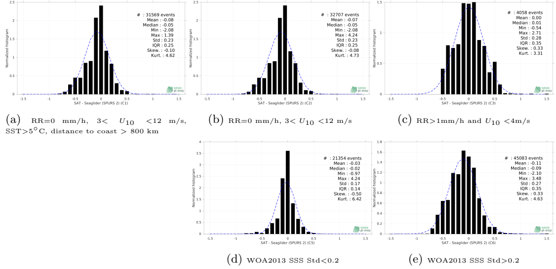
Figure 13: Normalized histogram of \Delta SSS (SMAP SSS L3 v5 - Monthly (RSS) - Seaglider (SPURS 2)) for 5 different subdatasets corresponding to: RR=0 mm/h, 3 < U_{10} < 12 m/s, SST>5°C, distance to coast > 800 km (a), RR=0 mm/h, 3 < U_{10} < 12 m/s (b), RR>1mm/h and U_{10} < 4 m/s (c), WOA2013 SSS Std<0.2 (d), WOA2013 SSS Std>0.2 (e).
