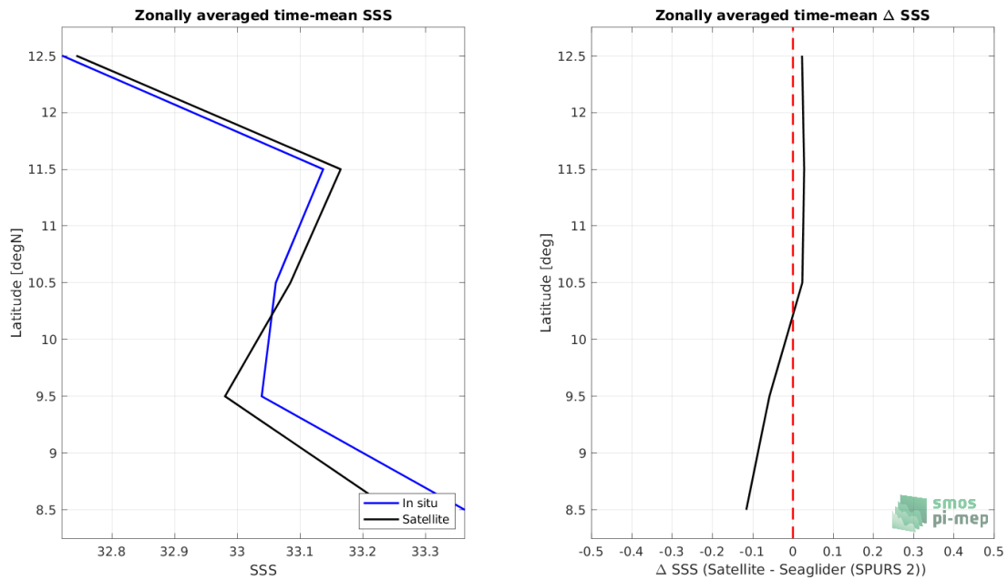
Figure 8: Left panel: Zonal mean SSS from SMAP SSS L3 v5 - Monthly (RSS) satellite product (black) and from Seaglider (SPURS 2) (blue). Right panel: Zonal mean of \Delta SSS (Satellite - Seaglider (SPURS 2)) for all the collected Pi-MEP match-up pairs estimated over the full satellite product period.
