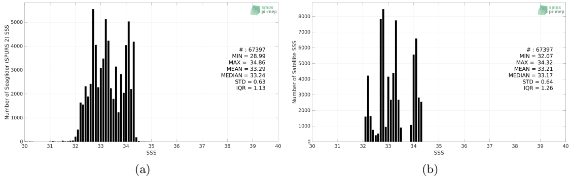
Figure 2: Histograms of SSS from Seaglider (SPURS 2) (a) and SMAP SSS L3 v5 - Monthly (RSS) (b) considering all match-up pairs per bins of 0.1 over the SPURS 2 Pi-MEP region and for the full satellite product period.
