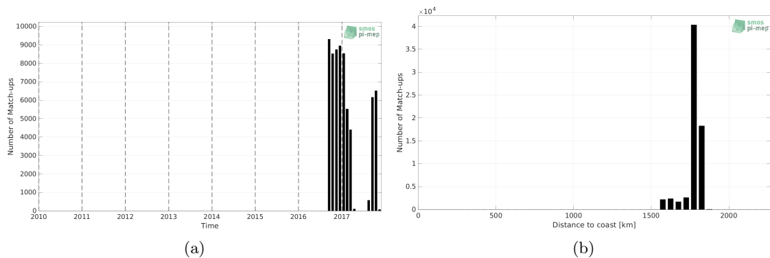
Figure 1: Number of match-ups between Seaglider (SPURS 2) and SMAP SSS L3 v5 - Monthly (RSS) SSS as a function of time (a) and as function of the distance to coast (b) over the SPURS 2 Pi-MEP region and for the full satellite product period.
