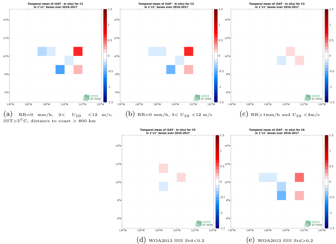
Figure 12: Temporal mean gridded over spatial boxes of size 1^\circ \times 1^\circ of \Delta SSS (SMAP SSS L3 v5 - Monthly (RSS) - Seaglider (SPURS 2)) for 5 different subdatasets corresponding to:RR=0 mm/h, 3 < U_{10} < 12 m/s, SST >5^\circ C, distance to coast > 800 km (a), RR=0 mm/h, 3 < U_{10} < 12 m/s (b), RR >1 mm/h and U_{10} < 4 m/s (c), WOA2013 SSS Std <0.2 (d), WOA2013 SSS Std >0.2 (e).
