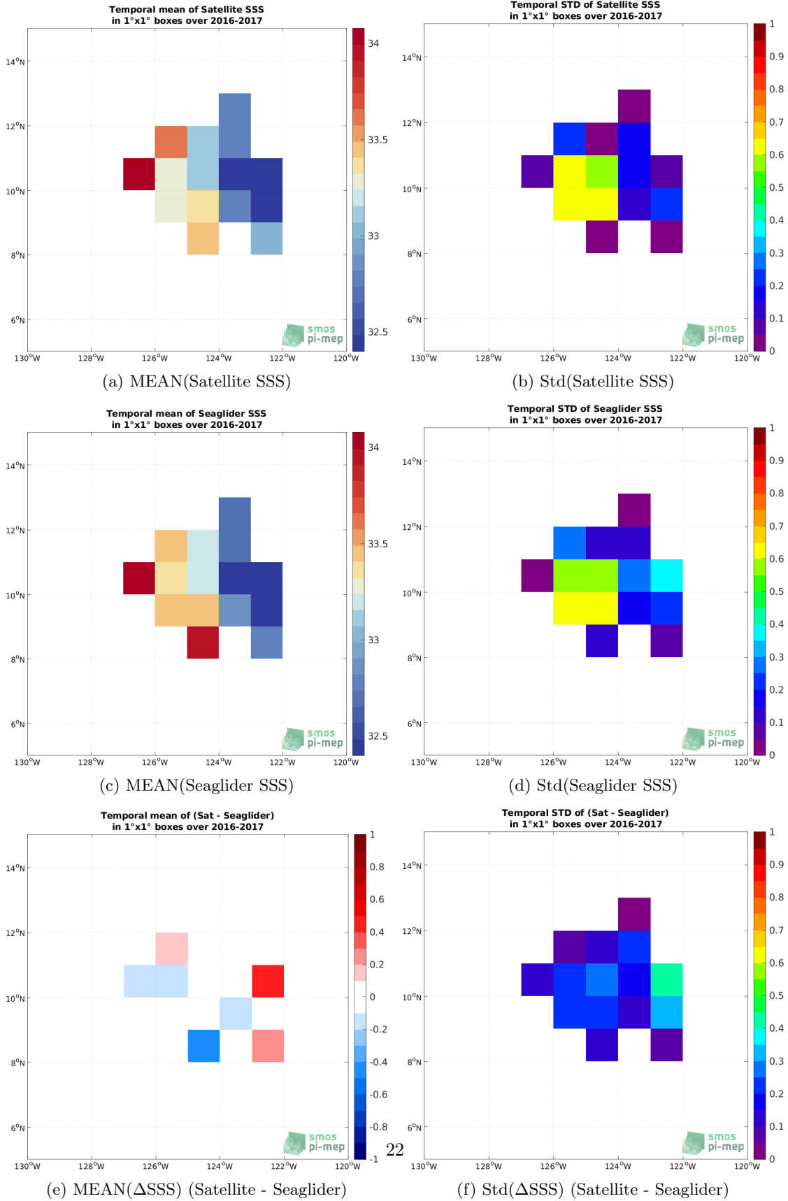
Figure 6: Temporal mean (left) and Std (right) of SSS from SMAP SSS L3 v5 - Monthly (RSS) (top), Seaglider (middle), and of \Delta SSS (Satellite - Seaglider). Only match-up pairs are used to generate these maps.
