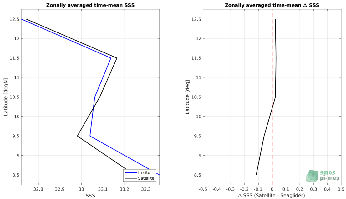
Figure 8: Left panel: Zonal mean SSS from SMAP SSS L3 v5 - Monthly (RSS) satellite product (black) and from Seaglider (blue). Right panel: Zonal mean of \Delta SSS (Satellite - Seaglider) for all the collected Pi-MEP match-up pairs estimated over the full satellite product period.
