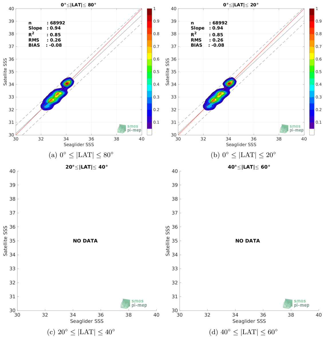
Figure 9: Contour maps of the concentration of SMAP SSS L3 v5 - Monthly (RSS) SSS (y-axis) versus Seaglider SSS (x-axis) at match-up pairs for different latitude bands. For each plot, the red line shows x=y . The black thin and dashed lines indicate a linear fit through the data cloud and the \pm 95\% confidence levels, respectively. The number match-up pairs n , the slope and R^2 coefficient of the linear fit, the root mean square (RMS) and the mean bias between satellite and in situ data are indicated for each latitude band in each plots.
