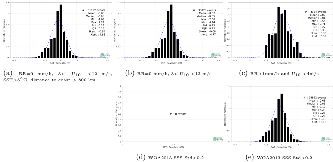
Figure 13: Normalized histogram of \Delta SSS (SMAP SSS L3 v5 - Monthly (RSS) - Seaglider) for 5 different subdatasets corresponding to: RR=0 mm/h, 3 < U_{10} < 12 m/s, SST > 5°C, distance to coast > 800 km (a), RR=0 mm/h, 3 < U_{10} < 12 m/s (b), RR > 1mm/h and U_{10} < 4 m/s (c), WOA2013 SSS Std < 0.2 (d), WOA2013 SSS Std > 0.2 (e).
