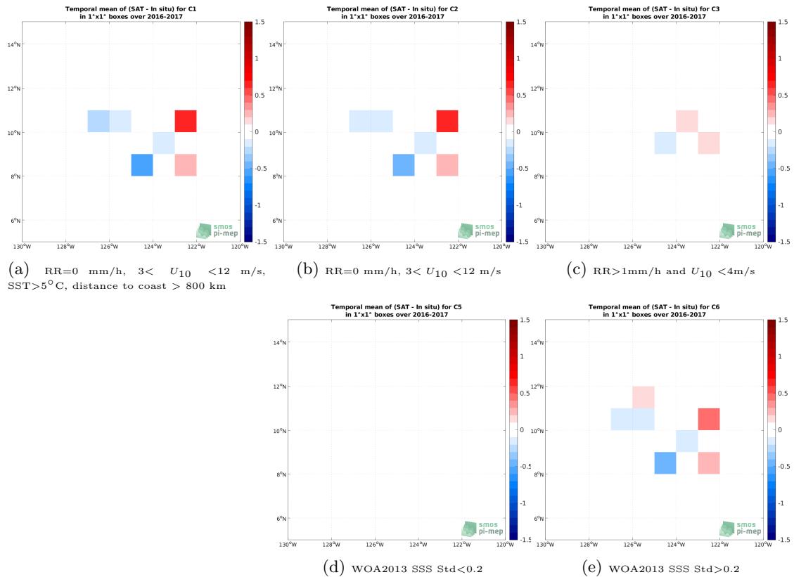
Figure 12: Temporal mean gridded over spatial boxes of size 1^\circ \times 1^\circ of \Delta SSS (SMAP SSS L3 v5 - Monthly (RSS) - Seaglider) for 5 different subdatasets corresponding to:RR=0 mm/h, 3 < U_{10} < 12 m/s, SST >5^\circ C, distance to coast > 800 km (a), RR=0 mm/h, 3 < U_{10} < 12 m/s (b), RR >1 mm/h and U_{10} < 4 m/s (c), WOA2013 SSS Std <0.2 (d), WOA2013 SSS Std >0.2 (e).
