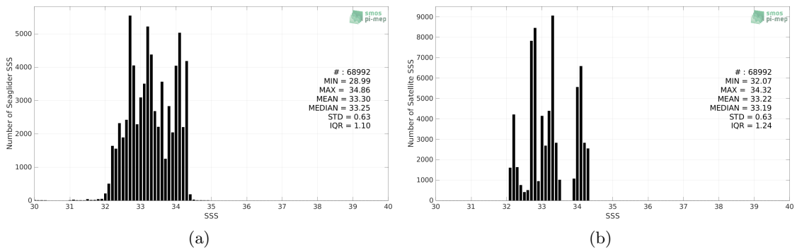
Figure 2: Histograms of SSS from Seaglider (a) and SMAP SSS L3 v5 - Monthly (RSS) (b) considering all match-up pairs per bins of 0.1 over the SPURS 2 Pi-MEP region and for the full satellite product period.
