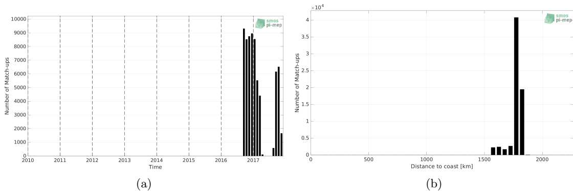
Figure 1: Number of match-ups between Seaglider and SMAP SSS L3 v5 - Monthly (RSS) SSS as a function of time (a) and as function of the distance to coast (b) over the SPURS 2 Pi-MEP region and for the full satellite product period.
