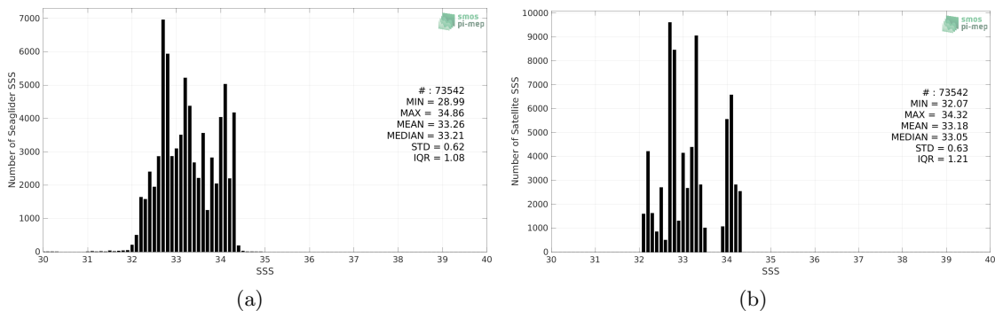
Figure 2: Histograms of SSS from Seagliders (a) and SMAP SSS L3 v5 - Monthly (RSS) (b) considering all match-up pairs per bins of 0.1 over the SPURS 2 Pi-MEP region and for the full satellite product period.
