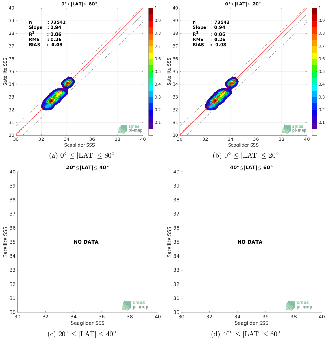
Figure 8: Contour maps of the concentration of SMAP SSS L3 v5 - Monthly (RSS) SSS (y-axis) versus Seaglider SSS (x-axis) at match-up pairs for different latitude bands. For each plot, the red line shows x=y . The black thin and dashed lines indicate a linear fit through the data cloud and the \pm 95\% confidence levels, respectively. The number match-up pairs n , the slope and R^2 coefficient of the linear fit, the root mean square (RMS) and the mean bias between satellite and in situ data are indicated for each latitude band in each plots.
