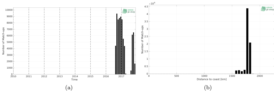
Figure 1: Number of match-ups between Seagliders and SMAP SSS L3 v5 - Monthly (RSS) SSS as a function of time (a) and as function of the distance to coast (b) over the SPURS 2 Pi-MEP region and for the full satellite product period.
