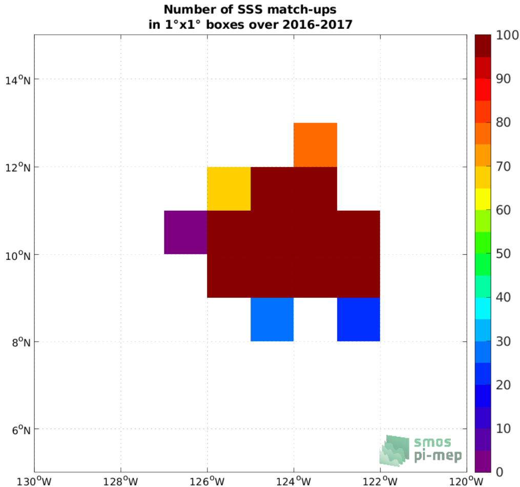
Figure 3: Number of SSS match-ups between Seaglider SSS and the SMAP SSS L3 v5 - Monthly (RSS) SSS product for the SPURS 2 Pi-MEP region over 1^\circ \times 1^\circ boxes and for the full satellite product period.
