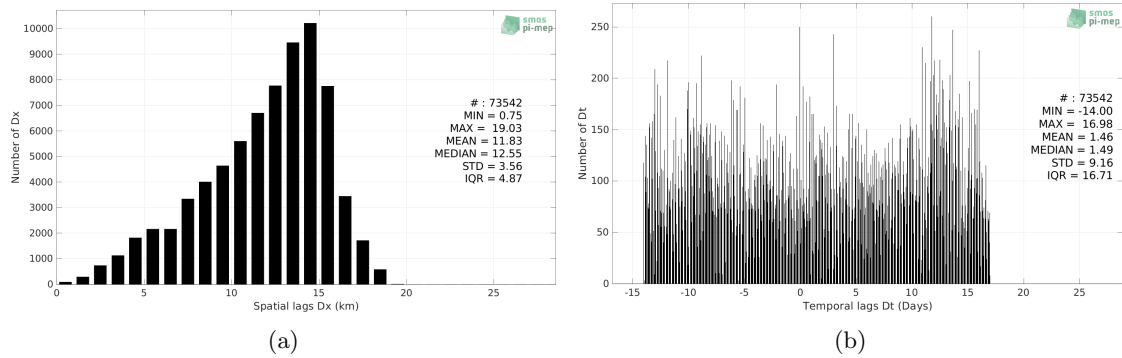
Figure 4: Histograms of the spatial (a) and temporal (b) lags between the location/time of the Seaglider measurement and the date of the corresponding SMAP SSS L3 v5 - Monthly (RSS) SSS pixel.
