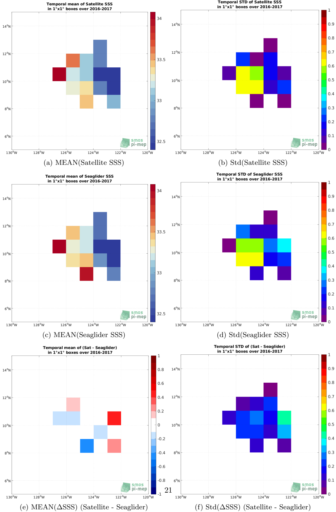
Figure 5: Temporal mean (left) and Std (right) of SSS from SMAP SSS L3 v5 - Monthly (RSS) (top), Seaglider (middle), and of \Delta SSS (Satellite - Seaglider). Only match-up pairs are used to generate these maps.
