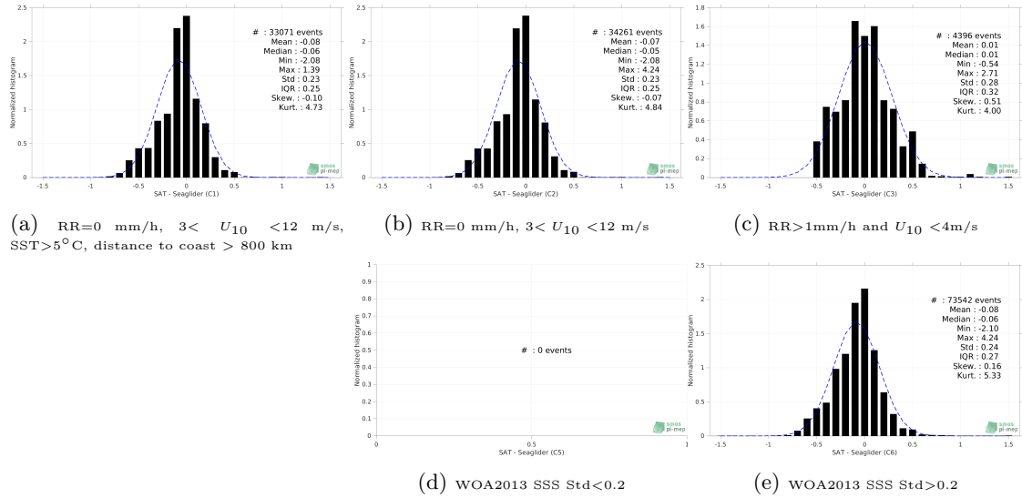
Figure 12: Normalized histogram of \Delta SSS (SMAP SSS L3 v5 - Monthly (RSS) - Seaglider) for 5 different subdatasets corresponding to: RR=0 mm/h, 3 < U_{10} < 12 m/s, SST > 5°C, distance to coast > 800 km (a), RR=0 mm/h, 3 < U_{10} < 12 m/s (b), RR > 1mm/h and U_{10} < 4 m/s (c), WOA2013 SSS Std < 0.2 (d), WOA2013 SSS Std > 0.2 (e).
