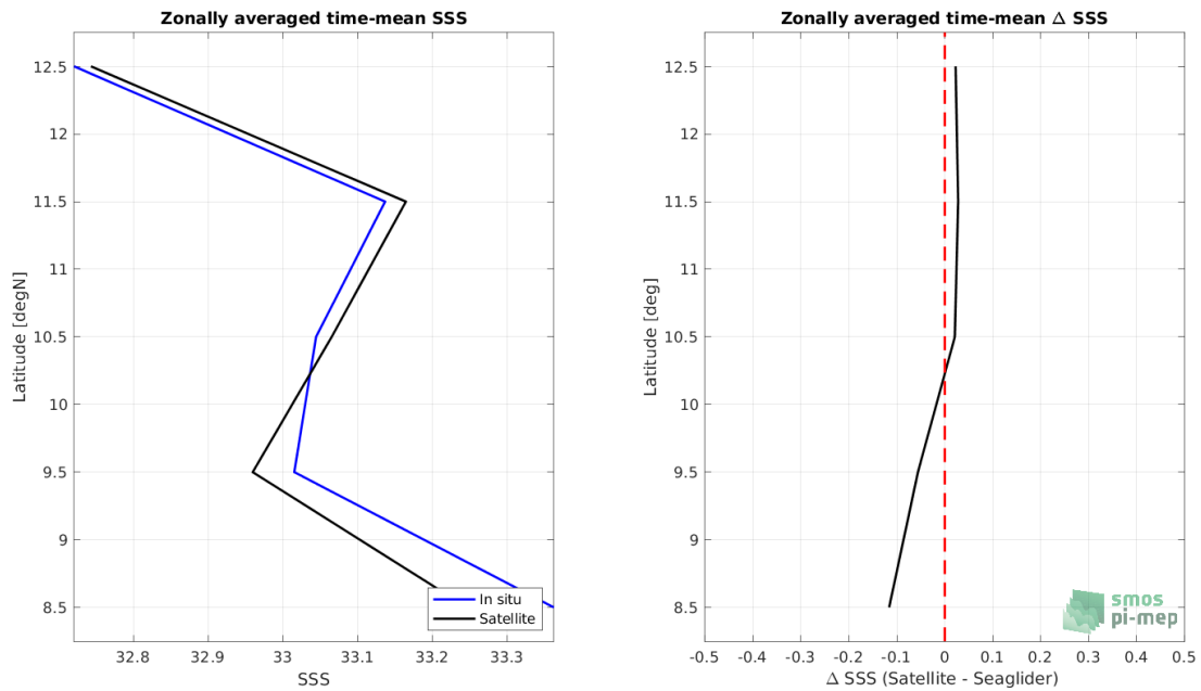
Figure 7: Left panel: Zonal mean SSS from SMAP SSS L3 v5 - Monthly (RSS) satellite product (black) and from Seaglider (blue). Right panel: Zonal mean of \Delta SSS (Satellite - Seaglider) for all the collected Pi-MEP match-up pairs estimated over the full satellite product period.
