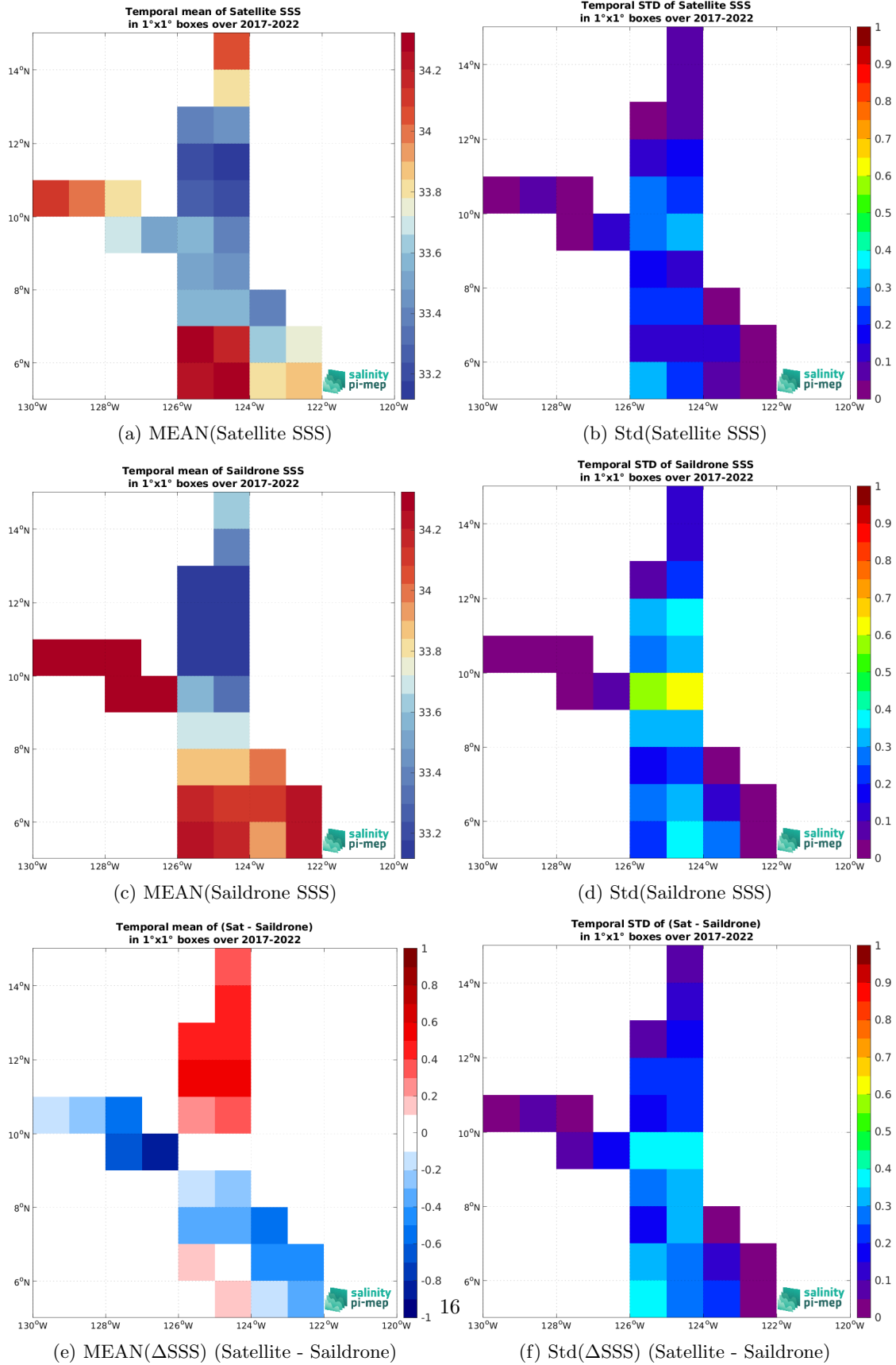
Figure 6: Temporal mean (left) and Std (right) of SSS from SMAP SSS L3 v5 - Monthly (RSS) (top), Saildrone (middle), and of \Delta SSS (Satellite - Saildrone). Only match-up pairs are used to generate these maps.
