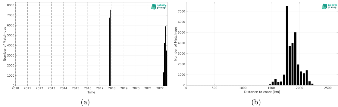
Figure 1: Number of match-ups between Sairdron and SMAP SSS L3 v5 - Monthly (RSS) SSS as a function of time (a) and as function of the distance to coast (b) over the SPURS 2 Pi-MEP region and for the full satellite product period.
