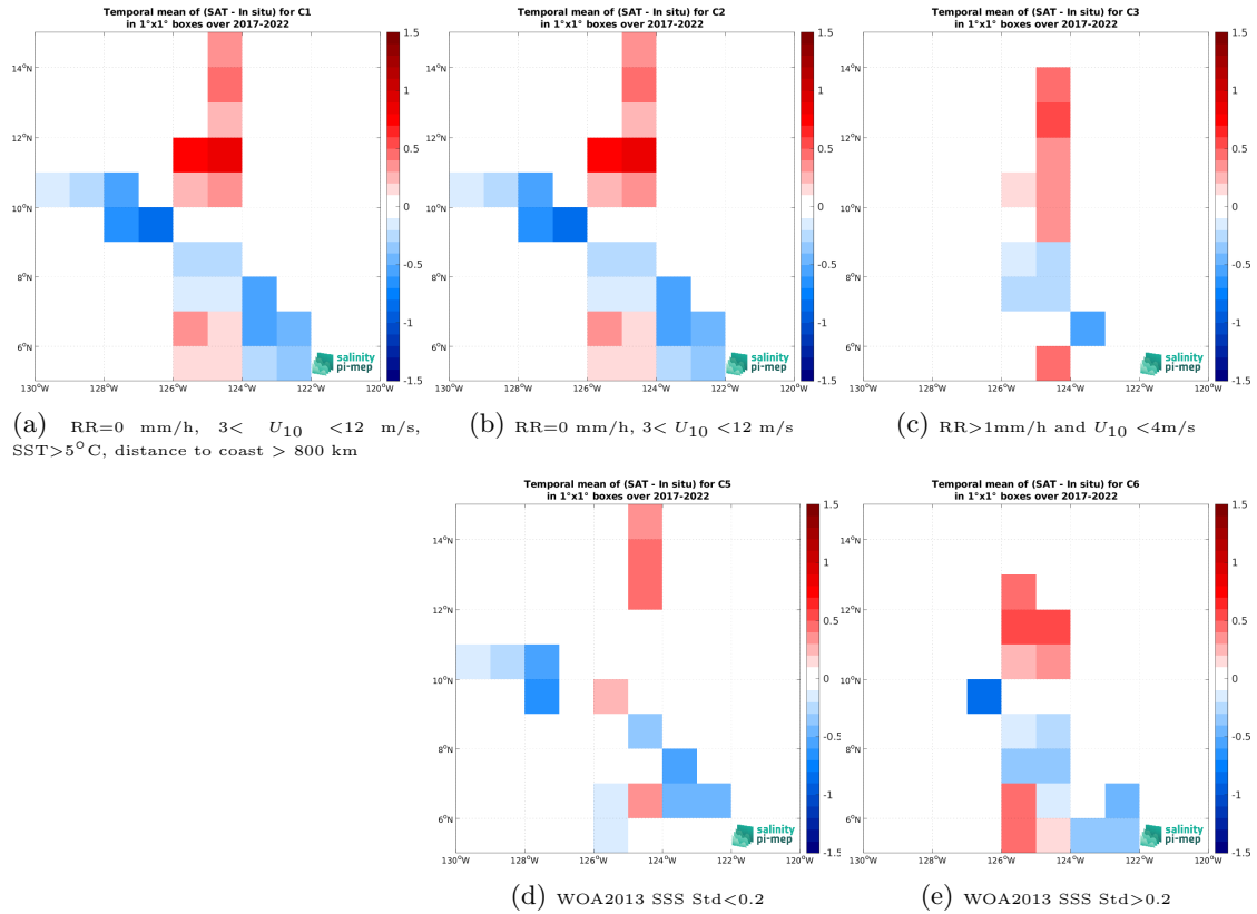
Figure 12: Temporal mean gridded over spatial boxes of size 1^\circ \times 1^\circ of \Delta SSS (SMAP SSS L3 v5 - Monthly (RSS) - Sairdrone) for 5 different subdatasets corresponding to:RR=0 mm/h, 3 < U_{10} < 12 m/s, SST >5^\circ\text{C} , distance to coast > 800 km (a), RR=0 mm/h, 3 < U_{10} < 12 m/s (b), RR >1 mm/h and U_{10} < 4 m/s (c), WOA2013 SSS Std <0.2 (d), WOA2013 SSS Std >0.2 (e).
