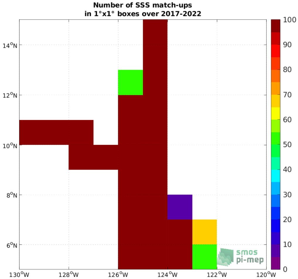
Figure 4: Number of SSS match-ups between Saildrone SSS and the SMAP SSS L3 v5 - Monthly (RSS) SSS product for the SPURS 2 Pi-MEP region over 1^\circ \times 1^\circ boxes and for the full satellite product period.
