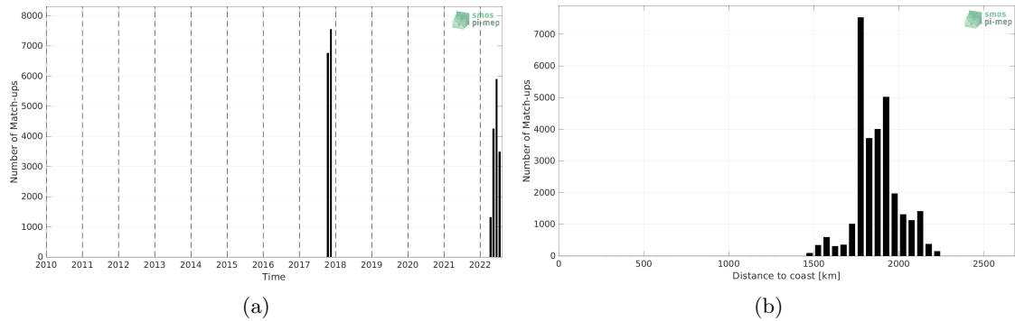
Figure 1: Number of match-ups between Sairdrone and SMAP SSS L3 v5 - Monthly (RSS) SSS as a function of time (a) and as function of the distance to coast (b) over the SPURS 2 Pi-MEP region and for the full satellite product period.
