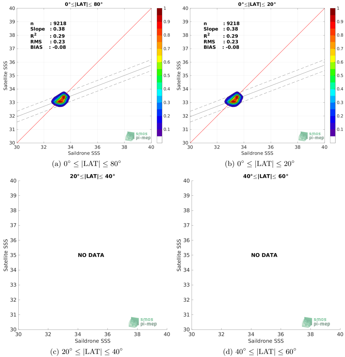
Figure 8: Contour maps of the concentration of SMAP SSS L3 v5 - Monthly (RSS) SSS (y-axis) versus Sailability SSS (x-axis) at match-up pairs for different latitude bands. For each plot, the red line shows x=y . The black thin and dashed lines indicate a linear fit through the data cloud and the \pm 95\% confidence levels, respectively. The number match-up pairs n , the slope and R^2 coefficient of the linear fit, the root mean square (RMS) and the mean bias between satellite and in situ data are indicated for each latitude band in each plots.
