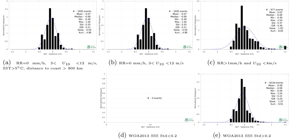
Figure 12: Normalized histogram of \Delta SSS (SMAP SSS L3 v5 - Monthly (RSS) - Saildrone) for 5 different subdatasets corresponding to: RR=0 mm/h, 3 < U_{10} < 12 m/s, SST > 5°C, distance to coast > 800 km (a), RR=0 mm/h, 3 < U_{10} < 12 m/s (b), RR > 1mm/h and U_{10} < 4 m/s (c), WOA2013 SSS Std < 0.2 (d), WOA2013 SSS Std > 0.2 (e).
