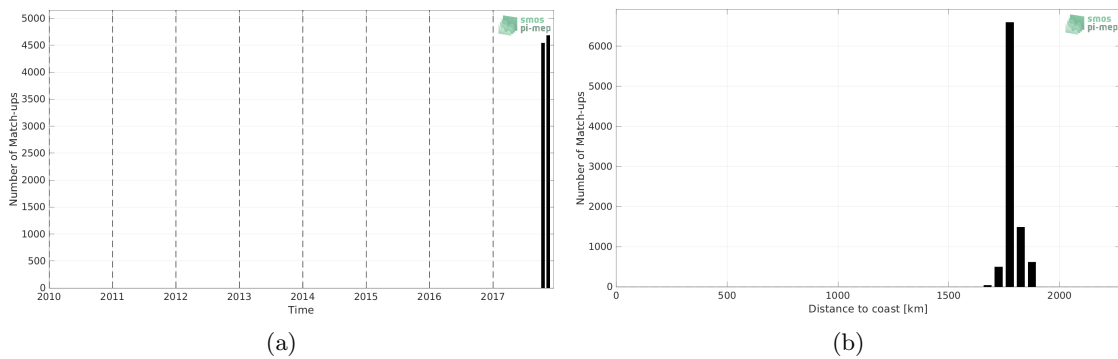
Figure 1: Number of match-ups between Saildrone and SMAP SSS L3 v5 - Monthly (RSS) SSS as a function of time (a) and as function of the distance to coast (b) over the SPURS 2 Pi-MEP region and for the full satellite product period.
