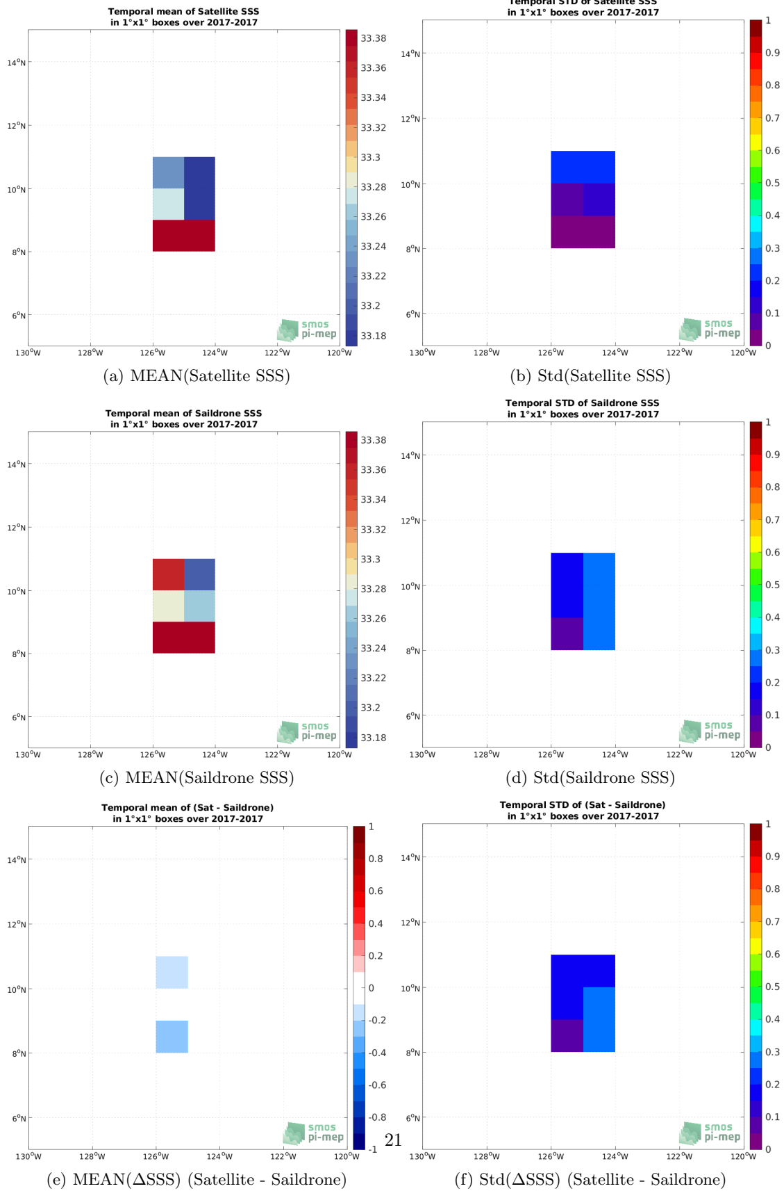
Figure 5: Temporal mean (left) and Std (right) of SSS from SMAP SSS L3 v5 - Monthly (RSS) (top), Saildrone (middle), and of \Delta SSS (Satellite - Saildrone). Only match-up pairs are used to generate these maps.
