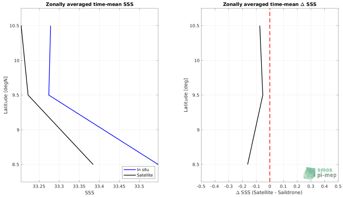
Figure 7: Left panel: Zonal mean SSS from SMAP SSS L3 v5 - Monthly (RSS) satellite product (black) and from Sairdrone (blue). Right panel: Zonal mean of \Delta SSS (Satellite - Sairdrone) for all the collected Pi-MEP match-up pairs estimated over the full satellite product period.
