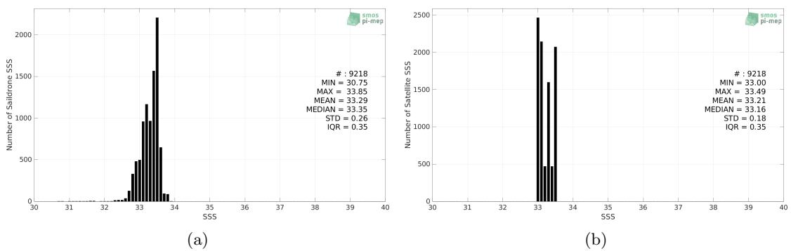
Figure 2: Histograms of SSS from Saildrone (a) and SMAP SSS L3 v5 - Monthly (RSS) (b) considering all match-up pairs per bins of 0.1 over the SPURS 2 Pi-MEP region and for the full satellite product period.
