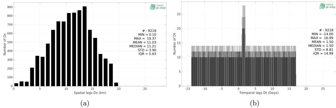
Figure 4: Histograms of the spatial (a) and temporal (b) lags between the location/time of the Sailldrone measurement and the date of the corresponding SMAP SSS L3 v5 - Monthly (RSS) SSS pixel.
