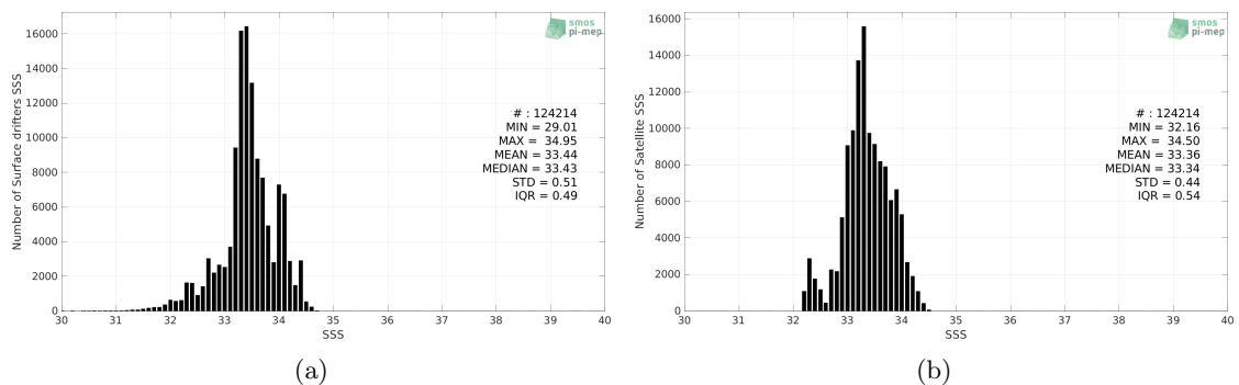
Figure 2: Histograms of SSS from Surface drifters (a) and SMAP SSS L3 v5 - Monthly (RSS) (b) considering all match-up pairs per bins of 0.1 over the SPURS 2 Pi-MEP region and for the full satellite product period.
