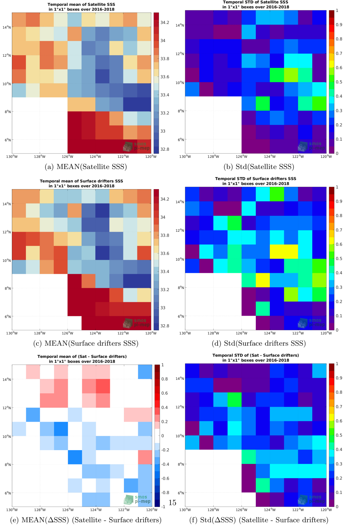
Figure 5: Temporal mean (left) and Std (right) of SSS from SMAP SSS L3 v5 - Monthly (RSS) (top), Surface drifters (middle), and of \Delta SSS (Satellite - Surface drifters). Only match-up pairs are used to generate these maps.
