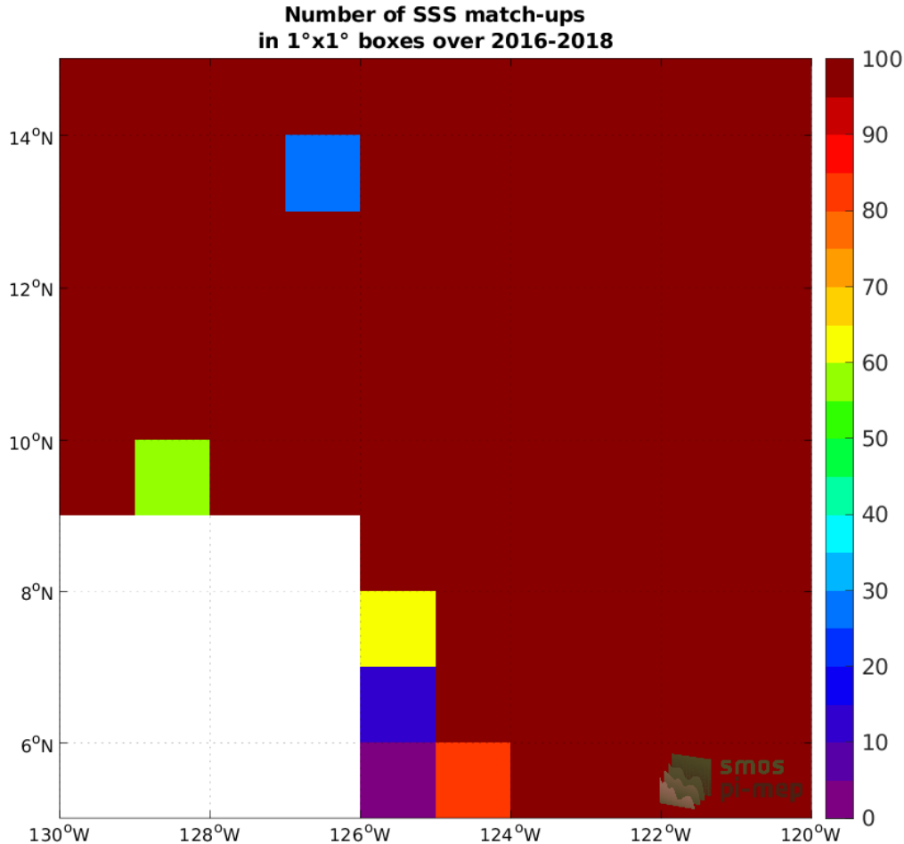
Figure 3: Number of SSS match-ups between Surface drifters SSS and the SMAP SSS L3 v5 - Monthly (RSS) SSS product for the SPURS 2 Pi-MEP region over 1^\circ \times 1^\circ boxes and for the full satellite product period.
