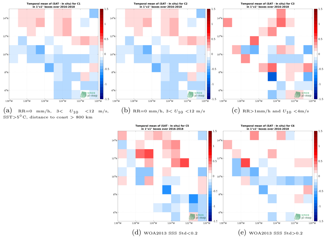
Figure 11: Temporal mean gridded over spatial boxes of size 1^\circ \times 1^\circ of \Delta SSS (SMAP SSS L3 v5 - Monthly (RSS) - Surface drifters) for 5 different subdatasets corresponding to:RR=0 mm/h, 3 < U_{10} < 12 m/s, SST > 5^\circ\text{C} , distance to coast > 800 km (a), RR=0 mm/h, 3 < U_{10} < 12 m/s (b), RR > 1 mm/h and U_{10} < 4 m/s (c), WOA2013 SSS Std < 0.2 (d), WOA2013 SSS Std > 0.2 (e).
