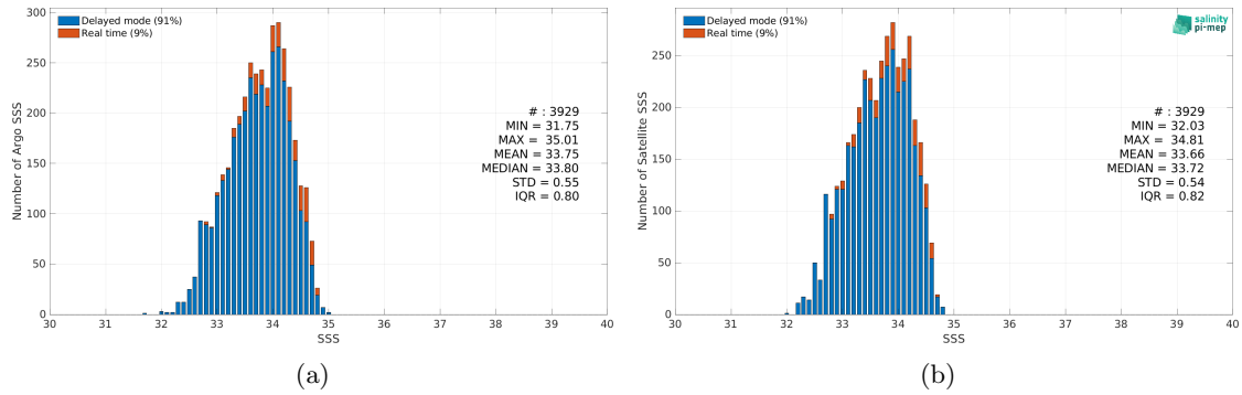
Figure 2: Histograms of SSS from Argo (a) and SMAP SSS L3 v5 - Monthly (RSS) (b) considering all match-up pairs per bins of 0.1 over the SPURS 2 Pi-MEP region and for the full satellite product period.
