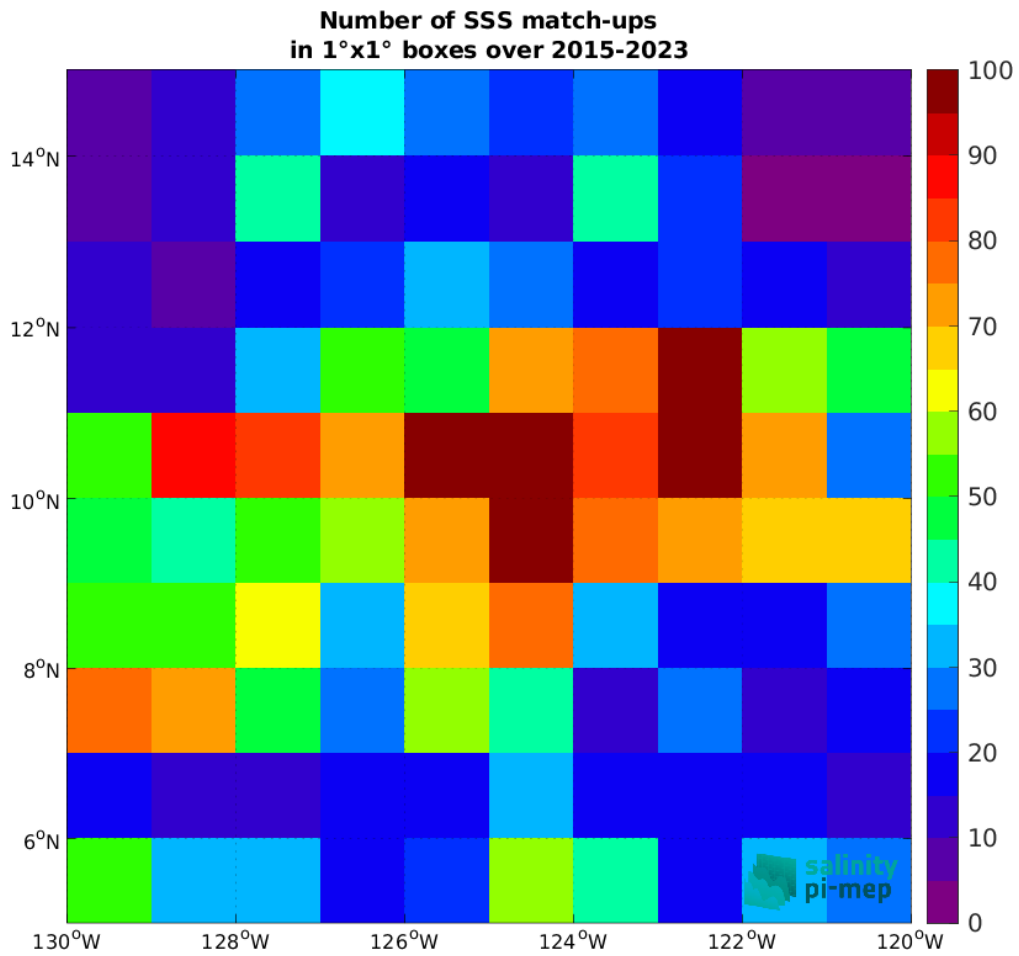
Figure 4: Number of SSS match-ups between Argo SSS and the SMAP SSS L3 v5 - Monthly (RSS) SSS product for the SPURS 2 Pi-MEP region over 1°x1° boxes and for the full satellite product period.
