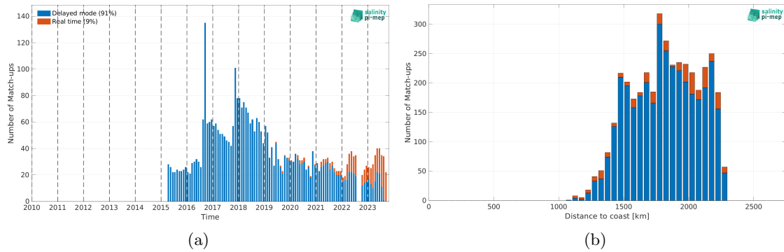
Figure 1: Number of match-ups between Argo and SMAP SSS L3 v5 - Monthly (RSS) SSS as a function of time (a) and as function of the distance to coast (b) over the SPURS 2 Pi-MEP region and for the full satellite product period.
