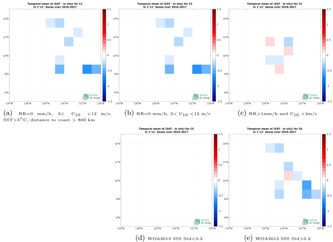
Figure 11: Temporal mean gridded over spatial boxes of size 1^\circ \times 1^\circ of \Delta\text{SSS} (SMAP SSS L3 v4 - 8-Day running (RSS) - Waveglider) for 5 different subdatasets corresponding to:RR=0 mm/h, 3 < U_{10} < 12 m/s, SST >5^\circ\text{C} , distance to coast > 800 km (a), RR=0 mm/h, 3 < U_{10} < 12 m/s (b), RR >1 mm/h and U_{10} < 4 m/s (c), WOA2013 SSS Std <0.2 (d), WOA2013 SSS Std >0.2 (e).
