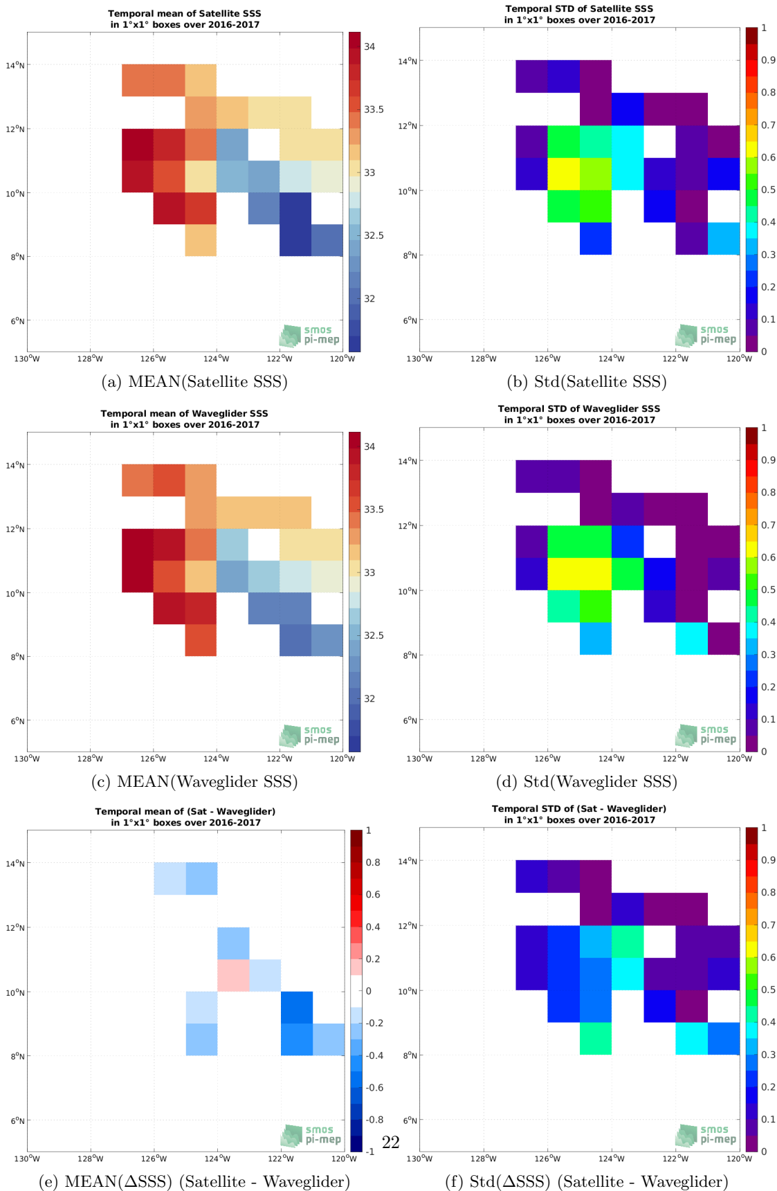
Figure 5: Temporal mean (left) and Std (right) of SSS from SMAP SSS L3 v4 - 8-Day running (RSS) (top), Waveglider (middle), and of \Delta SSS (Satellite - Waveglider). Only match-up pairs are used to generate these maps.
