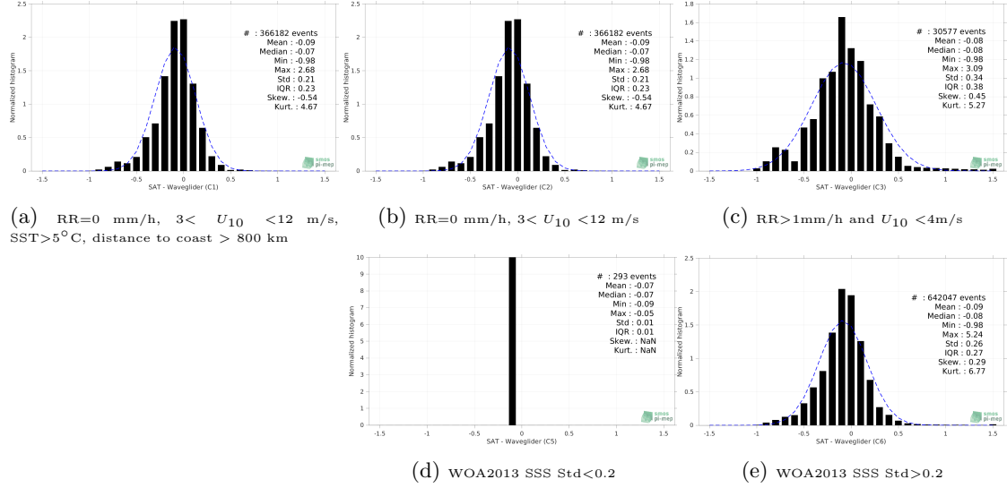
Figure 12: Normalized histogram of \Delta SSS (SMAP SSS L3 v4 - 8-Day running (RSS) - Waveglider) for 5 different subdatasets corresponding to: RR=0 mm/h, 3 < U_{10} < 12 m/s, SST > 5°C, distance to coast > 800 km (a), RR=0 mm/h, 3 < U_{10} < 12 m/s (b), RR > 1mm/h and U_{10} < 4 m/s (c), WOA2013 SSS Std < 0.2 (d), WOA2013 SSS Std > 0.2 (e).
