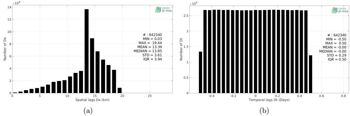
Figure 4: Histograms of the spatial (a) and temporal (b) lags between the location/time of the Waveglider measurement and the date of the corresponding SMAP SSS L3 v4 - 8-Day running (RSS) SSS pixel.
