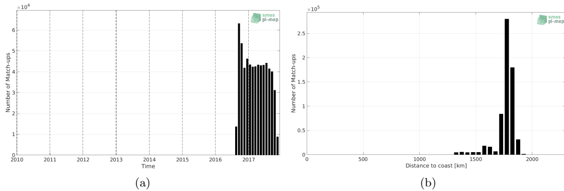
Figure 1: Number of match-ups between Waveglider and SMAP SSS L3 v4 - 8-Day running (RSS) SSS as a function of time (a) and as function of the distance to coast (b) over the SPURS 2 Pi-MEP region and for the full satellite product period.
