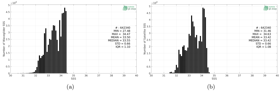
Figure 2: Histograms of SSS from Waveglider (a) and SMAP SSS L3 v4 - 8-Day running (RSS) (b) considering all match-up pairs per bins of 0.1 over the SPURS 2 Pi-MEP region and for the full satellite product period.
