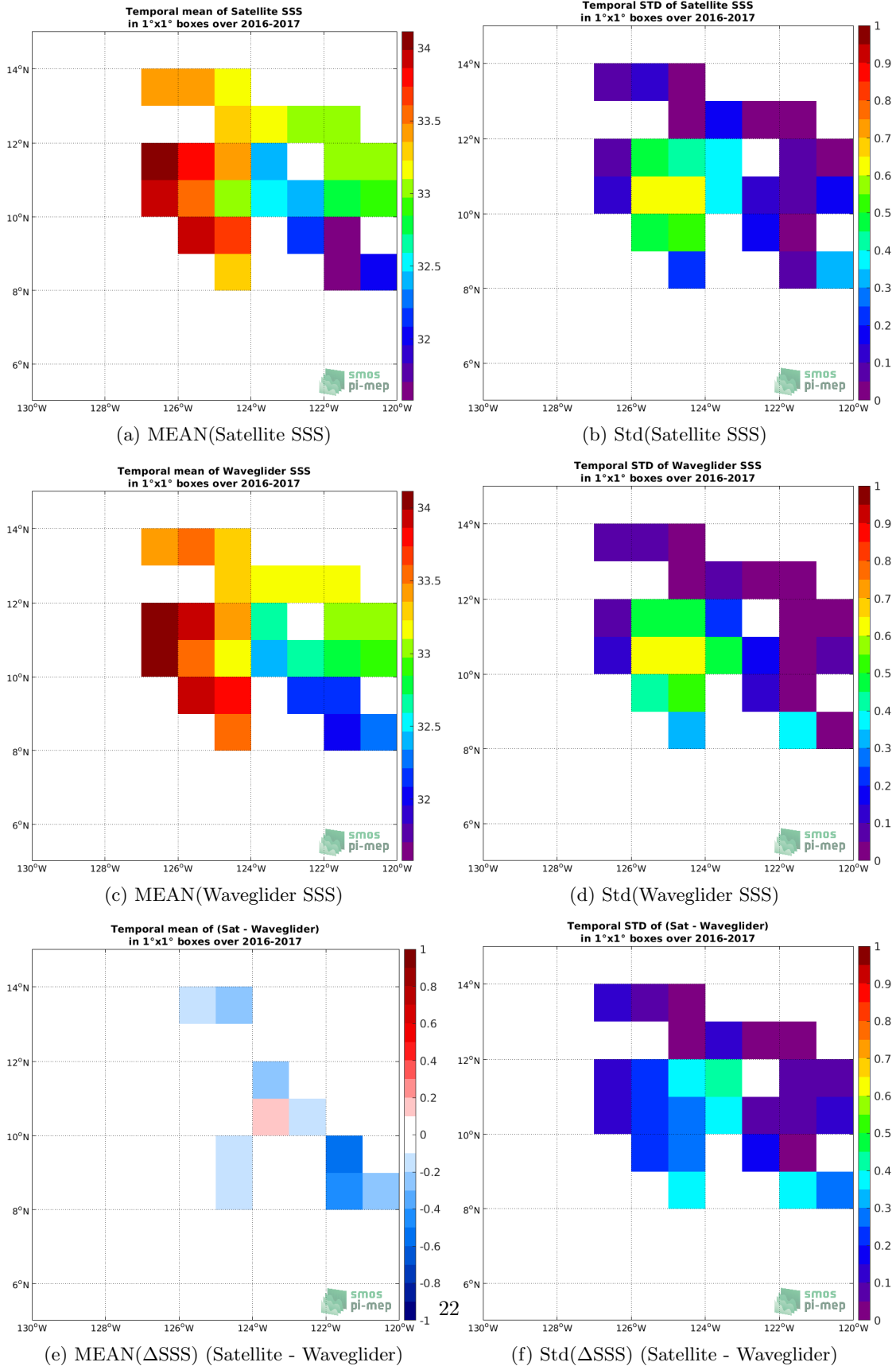
Figure 5: Temporal mean (left) and Std (right) of SSS from SMAP SSS L3 v4 - 8-Day running (RSS) (top), Waveglider (middle), and of \Delta SSS (Satellite - Waveglider). Only match-up pairs are used to generate these maps.
