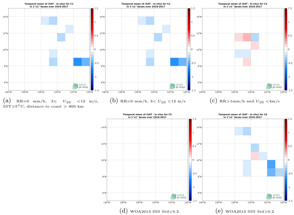
Figure 11: Temporal mean gridded over spatial boxes of size 1^\circ \times 1^\circ of \Delta SSS (SMAP SSS L3 v4 - 8-Day running (RSS) - Waveglider) for 5 different subdatasets corresponding to:RR=0 mm/h, 3 < U_{10} < 12 m/s, SST >5^\circ\text{C} , distance to coast > 800 km (a), RR=0 mm/h, 3 < U_{10} < 12 m/s (b), RR >1 mm/h and U_{10} < 4 m/s (c), WOA2013 SSS Std <0.2 (d), WOA2013 SSS Std >0.2 (e).
