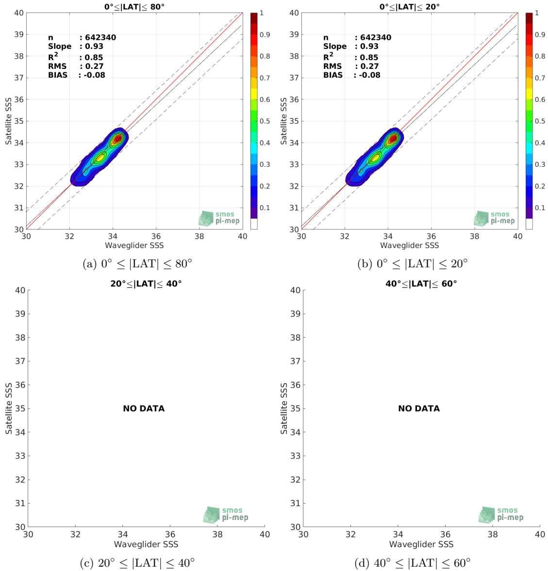
Figure 8: Contour maps of the concentration of SMAP SSS L3 v4 - 8-Day running (RSS) SSS (y-axis) versus Waveglider SSS (x-axis) at match-up pairs for different latitude bands. For each plot, the red line shows x=y . The black thin and dashed lines indicate a linear fit through the data cloud and the \pm 95\% confidence levels, respectively. The number match-up pairs n , the slope and R^2 coefficient of the linear fit, the root mean square (RMS) and the mean bias between satellite and in situ data are indicated for each latitude band in each plots.
