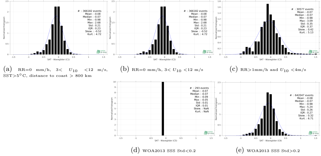
Figure 12: Normalized histogram of \Delta\text{SSS} (SMAP SSS L3 v4 - 8-Day running (RSS) - Waveglider) for 5 different subdatasets corresponding to: RR=0 mm/h, 3 < U_{10} < 12 m/s, SST > 5^\circ\text{C} , distance to coast > 800 km (a), RR=0 mm/h, 3 < U_{10} < 12 m/s (b), RR > 1\text{mm/h} and U_{10} < 4\text{m/s} (c), WOA2013 SSS \text{Std} < 0.2 (d), WOA2013 SSS \text{Std} > 0.2 (e).
