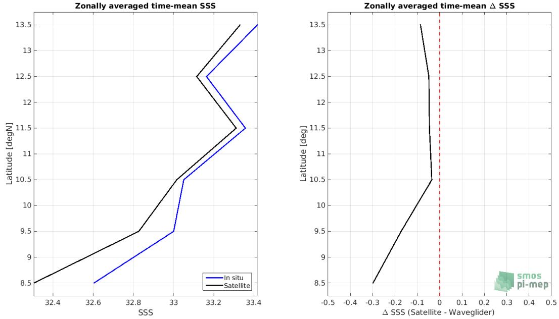
Figure 8: Left panel: Zonal mean SSS from SMAP SSS L3 v4 - 8-Day running (RSS) satellite product (black) and from Waveglider (blue). Right panel: Zonal mean of \Delta SSS (Satellite - Waveglider) for all the collected Pi-MEP match-up pairs estimated over the full satellite product period.
