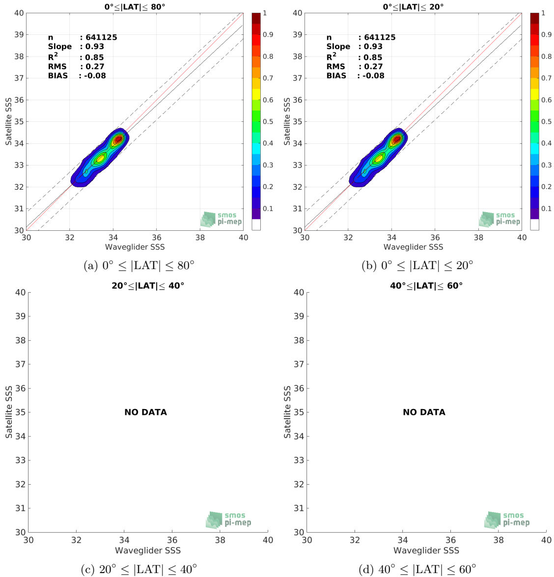
Figure 9: Contour maps of the concentration of SMAP SSS L3 v4 - 8-Day running (RSS) SSS (y-axis) versus Waveglider SSS (x-axis) at match-up pairs for different latitude bands. For each plot, the red line shows x=y . The black thin and dashed lines indicate a linear fit through the data cloud and the \pm 95\% confidence levels, respectively. The number match-up pairs n , the slope and R^2 coefficient of the linear fit, the root mean square (RMS) and the mean bias between satellite and in situ data are indicated for each latitude band in each plots.
