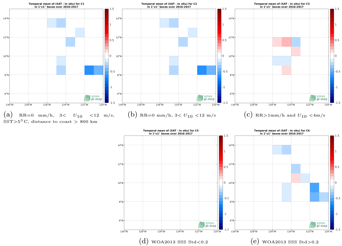
Figure 12: Temporal mean gridded over spatial boxes of size 1^\circ \times 1^\circ of \Delta SSS (SMAP SSS L3 v4 - 8-Day running (RSS) - Waveglider) for 5 different subdatasets corresponding to:RR=0 mm/h, 3 < U_{10} < 12 m/s, SST >5^\circ\text{C} , distance to coast > 800 km (a), RR=0 mm/h, 3 < U_{10} < 12 m/s (b), RR >1 mm/h and U_{10} < 4 m/s (c), WOA2013 SSS Std <0.2 (d), WOA2013 SSS Std >0.2 (e).
