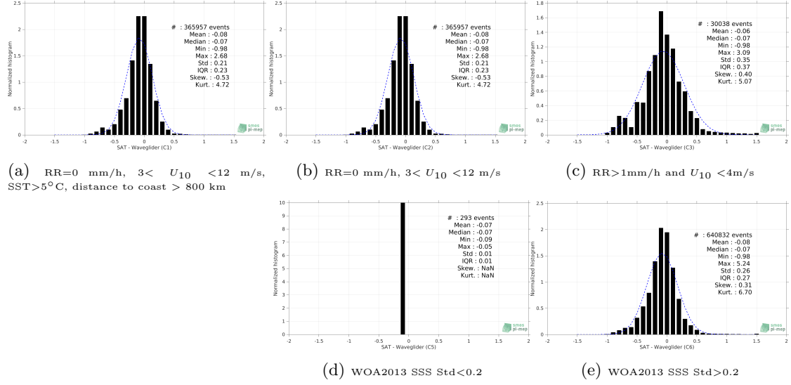
Figure 13: Normalized histogram of \Delta\text{SSS} (SMAP SSS L3 v4 - 8-Day running (RSS) - Waveglider) for 5 different subdatasets corresponding to: RR=0 mm/h, 3 < U_{10} < 12 m/s, SST > 5^\circ\text{C} , distance to coast > 800 km (a), RR=0 mm/h, 3 < U_{10} < 12 m/s (b), RR > 1\text{mm/h} and U_{10} < 4\text{m/s} (c), WOA2013 SSS Std < 0.2 (d), WOA2013 SSS Std > 0.2 (e).
