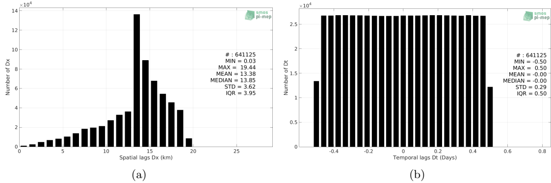
Figure 5: Histograms of the spatial (a) and temporal (b) lags between the time of the Waveglider measurements and the date of the corresponding SMAP SSS L3 v4 - 8-Day running (RSS) SSS product.
