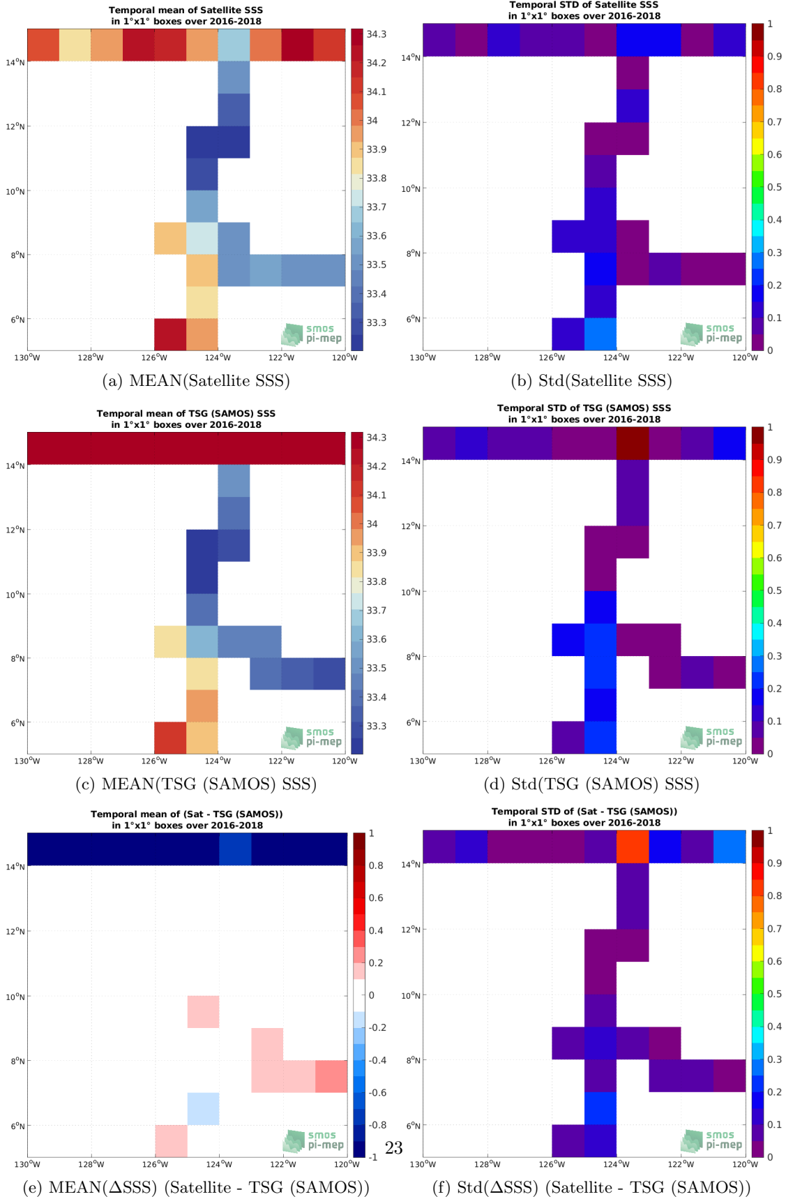
Figure 6: Temporal mean (left) and Std (right) of SSS from SMAP SSS L3 v4 - 8-Day running (RSS) (top), TSG (SAMOS) (middle), and of \Delta SSS (Satellite - TSG (SAMOS)). Only match-up pairs are used to generate these maps.
