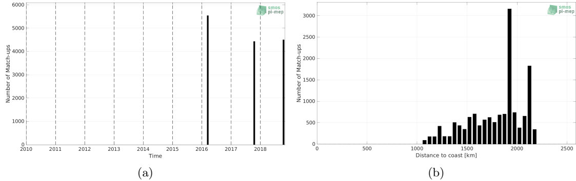
Figure 1: Number of match-ups between TSG (SAMOS) and SMAP SSS L3 v4 - 8-Day running (RSS) SSS as a function of time (a) and as function of the distance to coast (b) over the SPURS 2 Pi-MEP region and for the full satellite product period.
