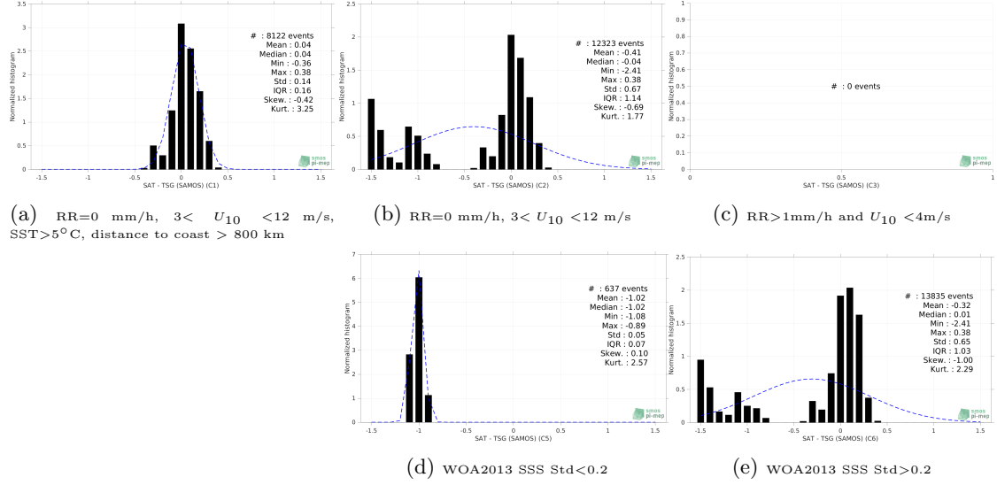
Figure 13: Normalized histogram of \Delta SSS (SMAP SSS L3 v4 - 8-Day running (RSS) - TSG (SAMOS)) for 5 different subdatasets corresponding to: RR=0 mm/h, 3 < U_{10} < 12 m/s, SST > 5°C, distance to coast > 800 km (a), RR=0 mm/h, 3 < U_{10} < 12 m/s (b), RR > 1mm/h and U_{10} < 4 m/s (c), WOA2013 SSS Std < 0.2 (d), WOA2013 SSS Std > 0.2 (e).
