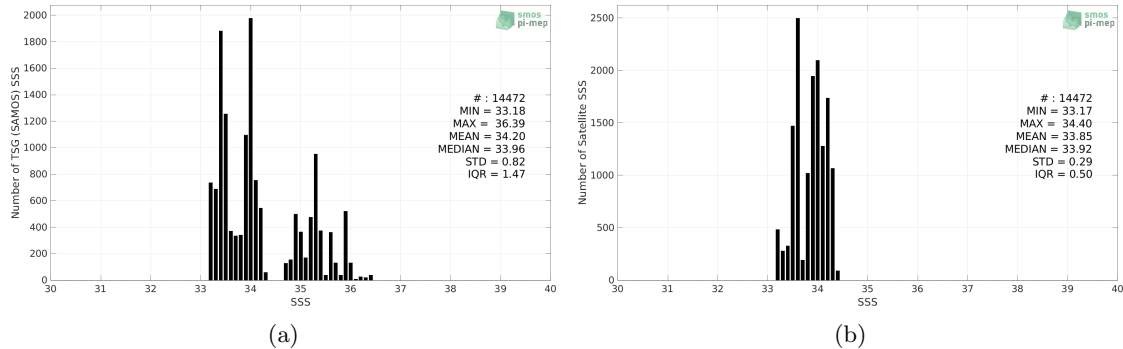
Figure 2: Histograms of SSS from TSG (SAMOS) (a) and SMAP SSS L3 v4 - 8-Day running (RSS) (b) considering all match-up pairs per bins of 0.1 over the SPURS 2 Pi-MEP region and for the full satellite product period.
