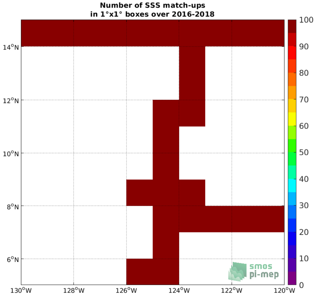
Figure 4: Number of SSS match-ups between TSG (SAMOS) SSS and the SMAP SSS L3 v4 - 8-Day running (RSS) SSS product for the SPURS 2 Pi-MEP region over 1°x1° boxes and for the full satellite product period.
