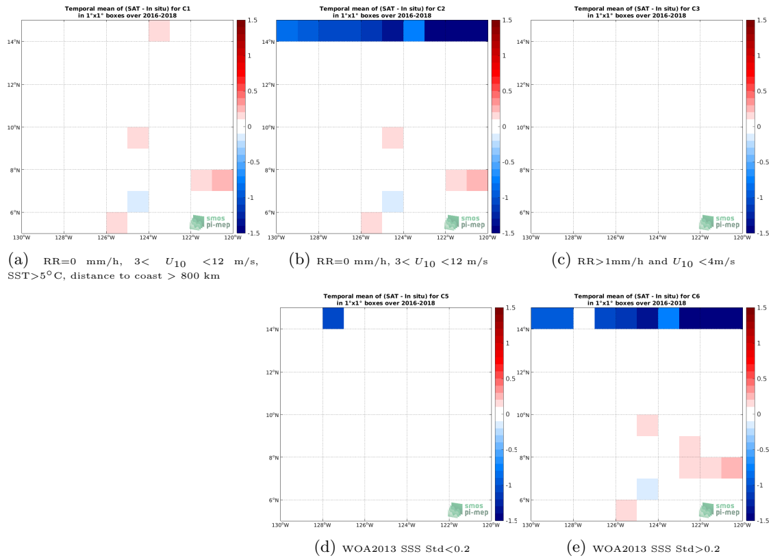
Figure 12: Temporal mean gridded over spatial boxes of size 1^\circ \times 1^\circ of \Delta SSS (SMAP SSS L3 v4 - 8-Day running (RSS) - TSG (SAMOS)) for 5 different subdatasets corresponding to:RR=0 mm/h, 3 < U_{10} < 12 m/s, SST >5^\circ\text{C} , distance to coast > 800 km (a), RR=0 mm/h, 3 < U_{10} < 12 m/s (b), RR >1 mm/h and U_{10} < 4 m/s (c), WOA2013 SSS Std <0.2 (d), WOA2013 SSS Std >0.2 (e).
