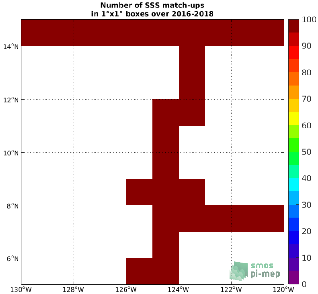
Figure 4: Number of SSS match-ups between TSG (SAMOS) SSS and the SMAP SSS L3 v4 - 8-Day running (RSS) SSS product for the SPURS 2 Pi-MEP region over 1°x1° boxes and for the full satellite product period.
