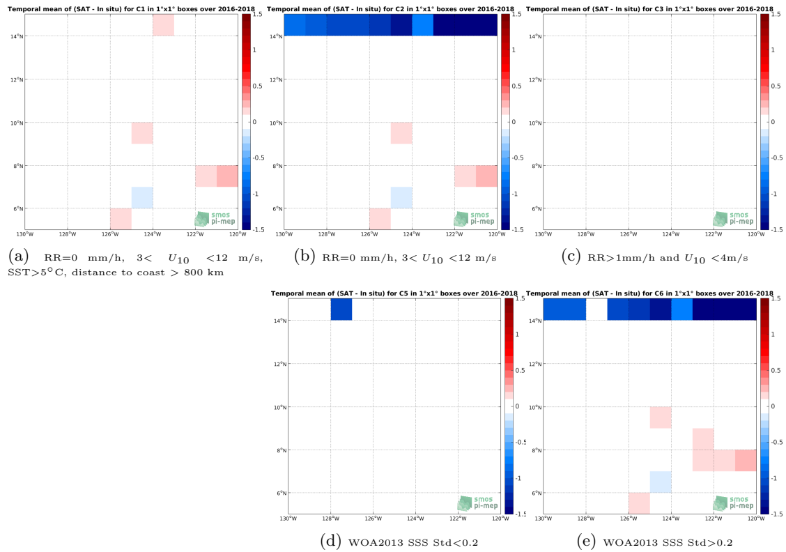
Figure 12: Temporal mean gridded over spatial boxes of size 1^\circ \times 1^\circ of \Delta SSS (SMAP-L3-RSS-V4-8DAY-RUNNING - TSG-SAMOS) for 5 different subdatasets corresponding to:RR=0 mm/h, 3 < U_{10} < 12 m/s, SST >5^\circ C, distance to coast > 800 km (a), RR=0 mm/h, 3 < U_{10} < 12 m/s (b), RR >1 mm/h and U_{10} < 4 m/s (c), WOA2013 SSS Std <0.2 (d), WOA2013 SSS Std >0.2 (e).
