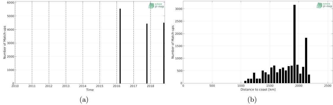
Figure 1: Number of match-ups between TSG-SAMOS and SMAP-L3-RSS-V4-8DAY-RUNNING SSS as a function of time (a) and as function of the distance to coast (b) over the SPURS 2 Pi-MEP region and for the full satellite product period.
