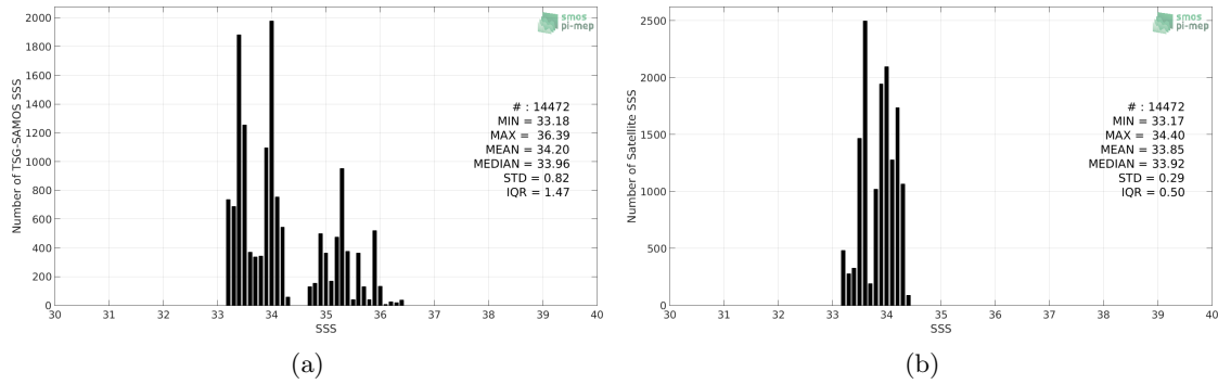
Figure 2: Histograms of SSS from TSG-SAMOS (a) and SMAP-L3-RSS-V4-8DAY-RUNNING (b) considering all match-up pairs per bins of 0.1 over the SPURS 2 Pi-MEP region and for the full satellite product period.
