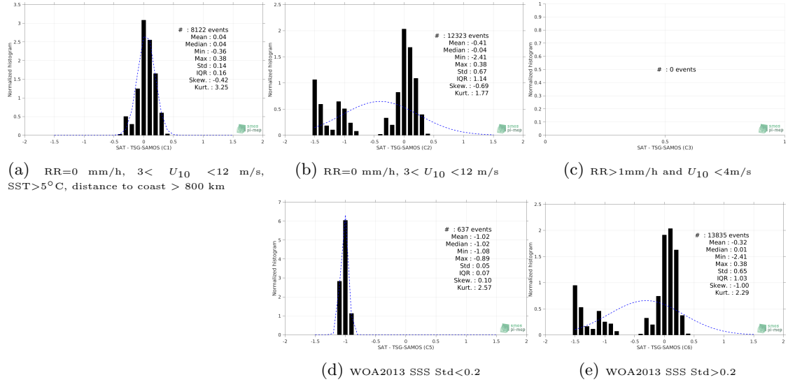
Figure 13: Normalized histogram of \Delta SSS (SMAP-L3-RSS-V4-8DAY-RUNNING - TSG-SAMOS) for 5 different subdatasets corresponding to: RR=0 mm/h, 3 < U_{10} < 12 m/s, SST>5°C, distance to coast > 800 km (a), RR=0 mm/h, 3 < U_{10} < 12 m/s (b), RR>1mm/h and U_{10} < 4 m/s (c), WOA2013 SSS Std<0.2 (d), WOA2013 SSS Std>0.2 (e).
