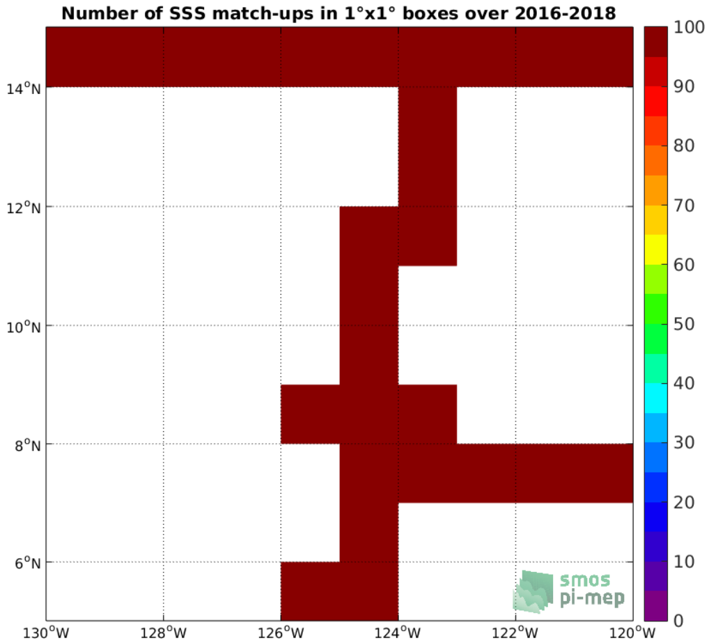
Figure 4: Number of SSS match-ups between TSG-SAMOS SSS and the SMAP-L3-RSS-V4-8DAY-RUNNING SSS product for the SPURS 2 Pi-MEP region over 1°x1° boxes and for the full satellite product period.
