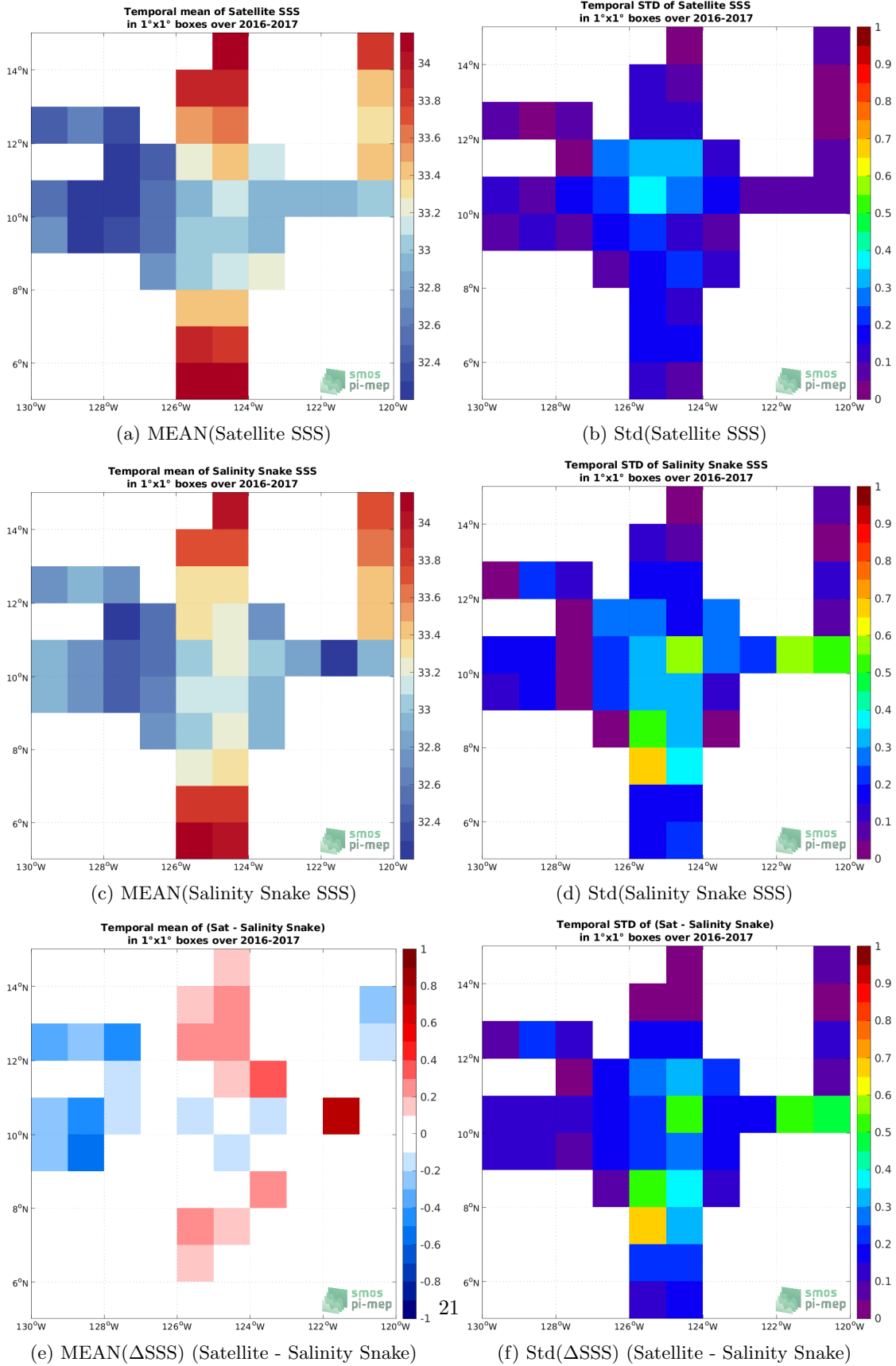
Figure 5: Temporal mean (left) and Std (right) of SSS from SMAP SSS L3 v4 - 8-Day running (RSS) (top), Salinity Snake (middle), and of \Delta SSS (Satellite - Salinity Snake). Only match-up pairs are used to generate these maps.
