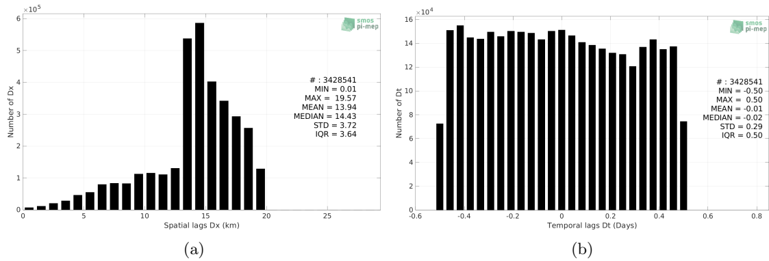
Figure 4: Histograms of the spatial (a) and temporal (b) lags between the location/time of the Salinity Snake measurement and the date of the corresponding SMAP SSS L3 v4 - 8-Day running (RSS) SSS pixel.
