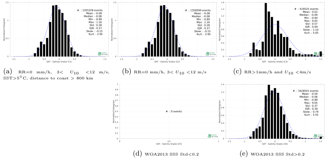
Figure 12: Normalized histogram of \Delta SSS (SMAP SSS L3 v4 - 8-Day running (RSS) - Salinity Snake) for 5 different subdatasets corresponding to: RR=0 mm/h, 3 < U_{10} < 12 m/s, SST > 5°C, distance to coast > 800 km (a), RR=0 mm/h, 3 < U_{10} < 12 m/s (b), RR > 1mm/h and U_{10} < 4 m/s (c), WOA2013 SSS Std < 0.2 (d), WOA2013 SSS Std > 0.2 (e).
