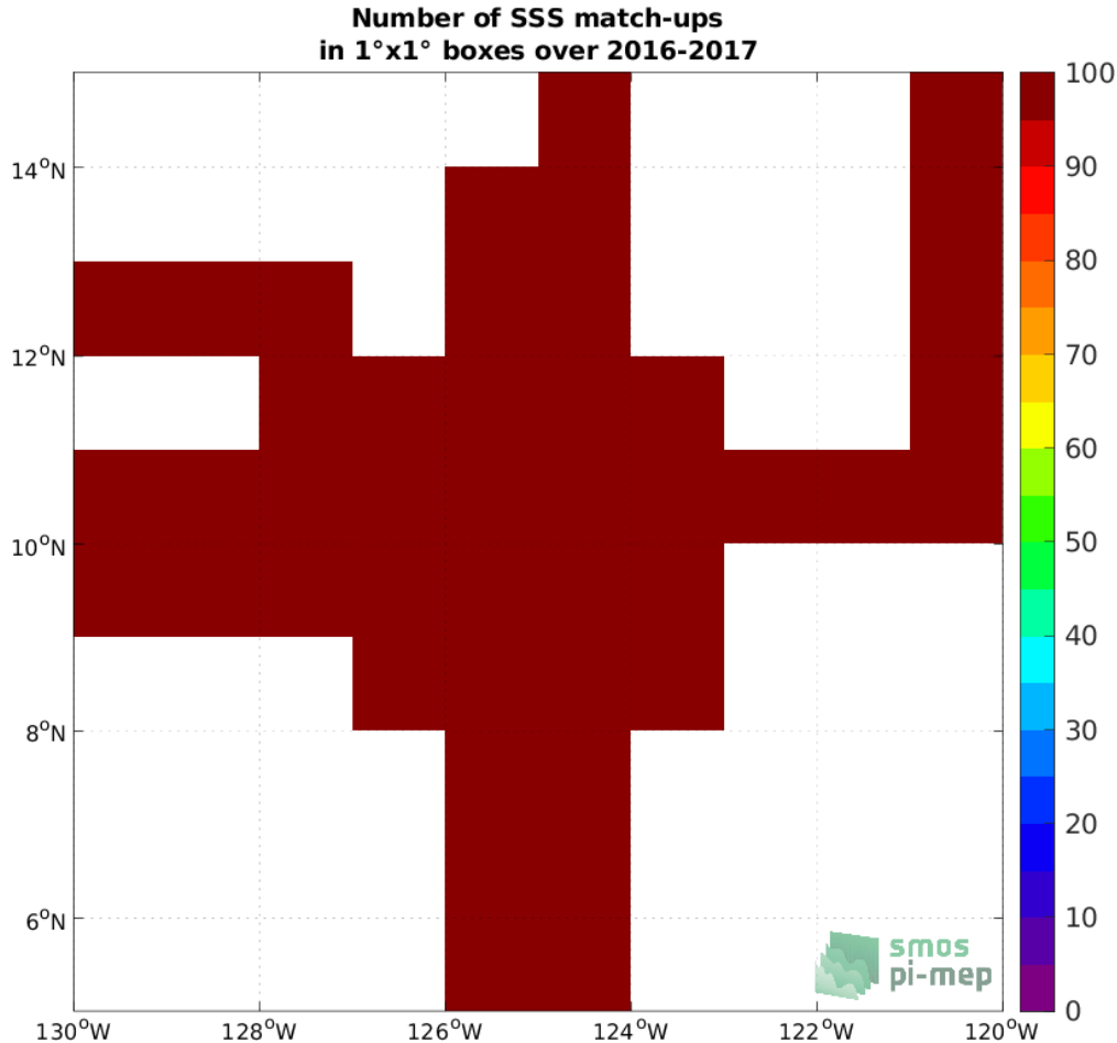
Figure 3: Number of SSS match-ups between Salinity Snake SSS and the SMAP SSS L3 v4 - 8-Day running (RSS) SSS product for the SPURS 2 Pi-MEP region over 1^\circ \times 1^\circ boxes and for the full satellite product period.
