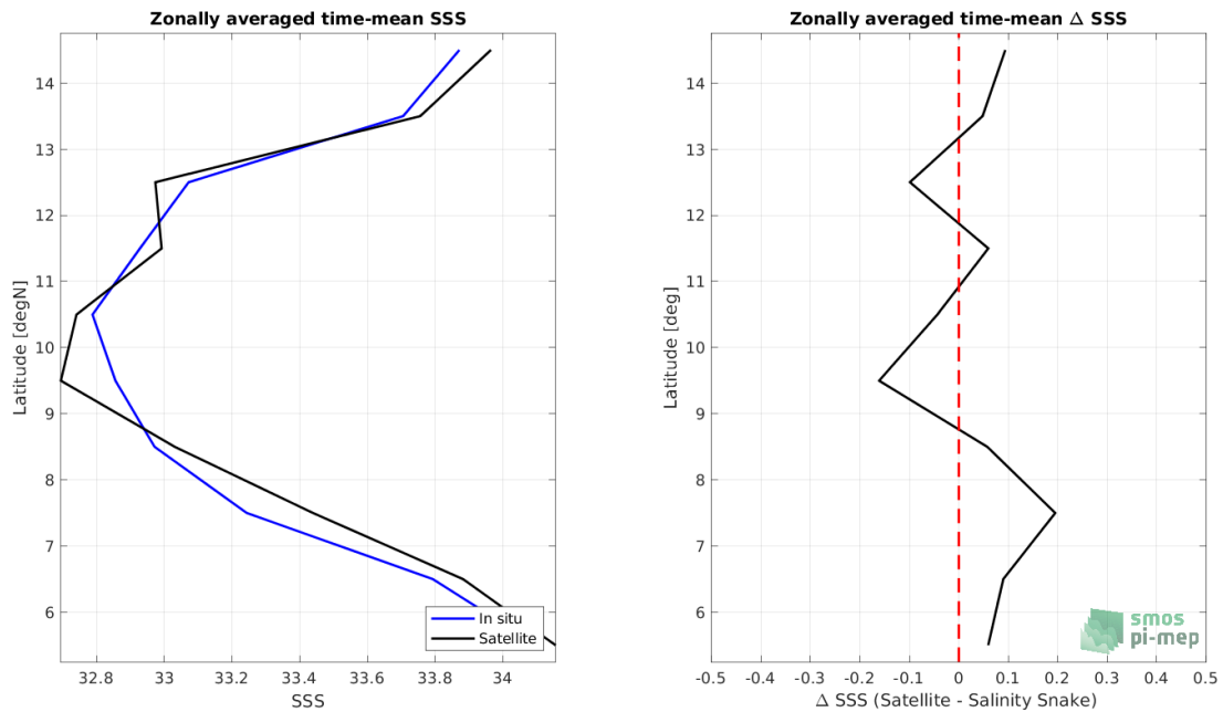
Figure 7: Left panel: Zonal mean SSS from SMAP SSS L3 v4 - 8-Day running (RSS) satellite product (black) and from Salinity Snake (blue). Right panel: Zonal mean of \Delta SSS (Satellite - Salinity Snake) for all the collected Pi-MEP match-up pairs estimated over the full satellite product period.
