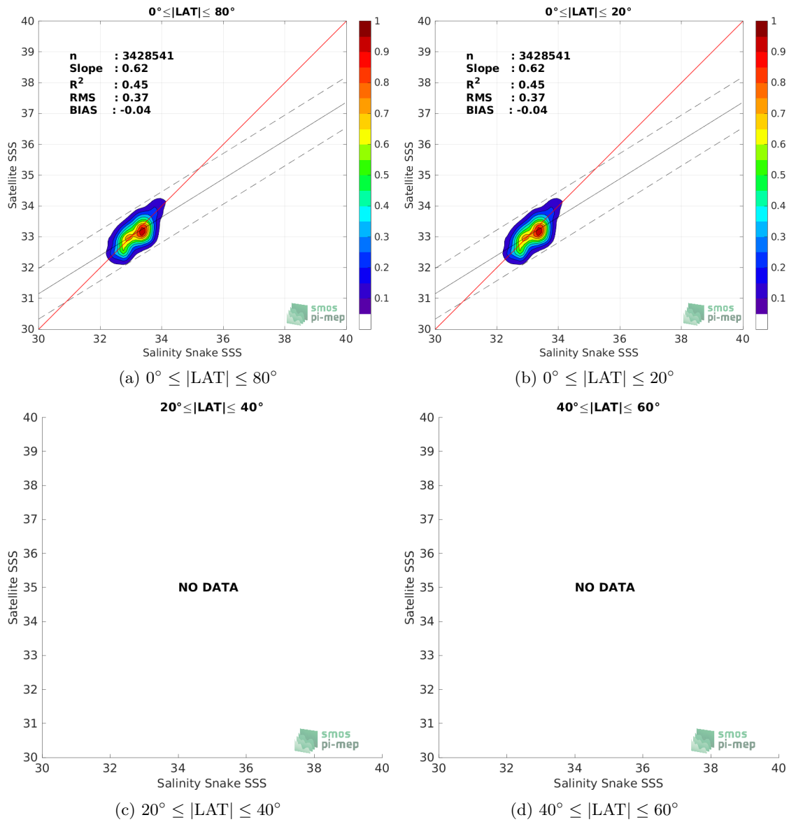
Figure 8: Contour maps of the concentration of SMAP SSS L3 v4 - 8-Day running (RSS) SSS (y-axis) versus Salinity Snake SSS (x-axis) at match-up pairs for different latitude bands. For each plot, the red line shows x=y . The black thin and dashed lines indicate a linear fit through the data cloud and the \pm 95\% confidence levels, respectively. The number match-up pairs n , the slope and R^2 coefficient of the linear fit, the root mean square (RMS) and the mean bias between satellite and in situ data are indicated for each latitude band in each plots.
