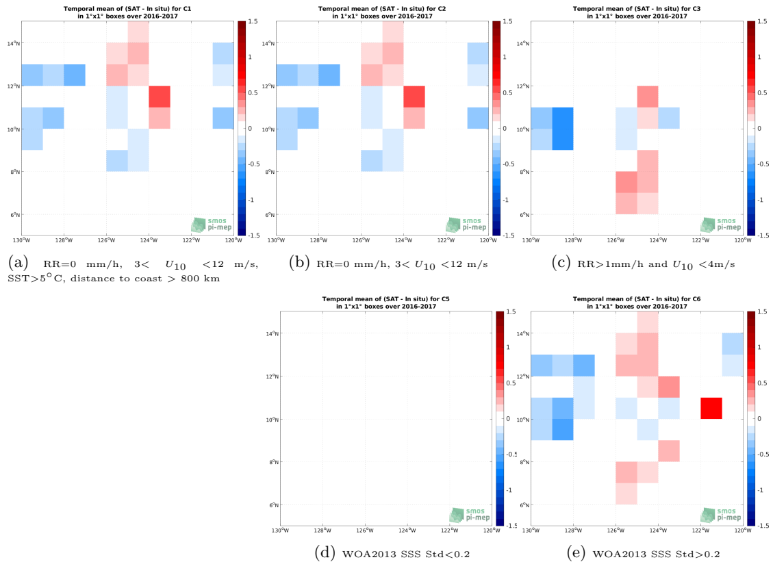
Figure 11: Temporal mean gridded over spatial boxes of size 1^\circ \times 1^\circ of \Delta SSS (SMAP SSS L3 v4 - 8-Day running (RSS) - Salinity Snake) for 5 different subdatasets corresponding to:RR=0 mm/h, 3 < U_{10} < 12 m/s, SST >5^\circ C, distance to coast > 800 km (a), RR=0 mm/h, 3 < U_{10} < 12 m/s (b), RR >1 mm/h and U_{10} < 4 m/s (c), WOA2013 SSS Std <0.2 (d), WOA2013 SSS Std >0.2 (e).
