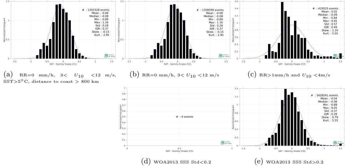
Figure 12: Normalized histogram of \Delta SSS (SMAP SSS L3 v4 - 8-Day running (RSS) - Salinity Snake) for 5 different subdatasets corresponding to: RR=0 mm/h, 3 < U_{10} < 12 m/s, SST>5°C, distance to coast > 800 km (a), RR=0 mm/h, 3 < U_{10} < 12 m/s (b), RR>1mm/h and U_{10} < 4 m/s (c), WOA2013 SSS Std<0.2 (d), WOA2013 SSS Std>0.2 (e).
