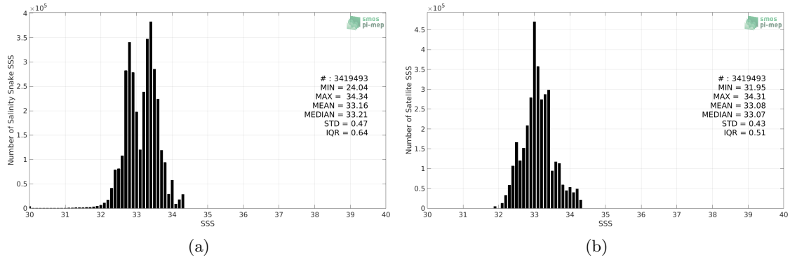
Figure 2: Histograms of SSS from Salinity Snake (a) and SMAP SSS L3 v4 - 8-Day running (RSS) (b) considering all match-up pairs per bins of 0.1 over the SPURS 2 Pi-MEP region and for the full satellite product period.
