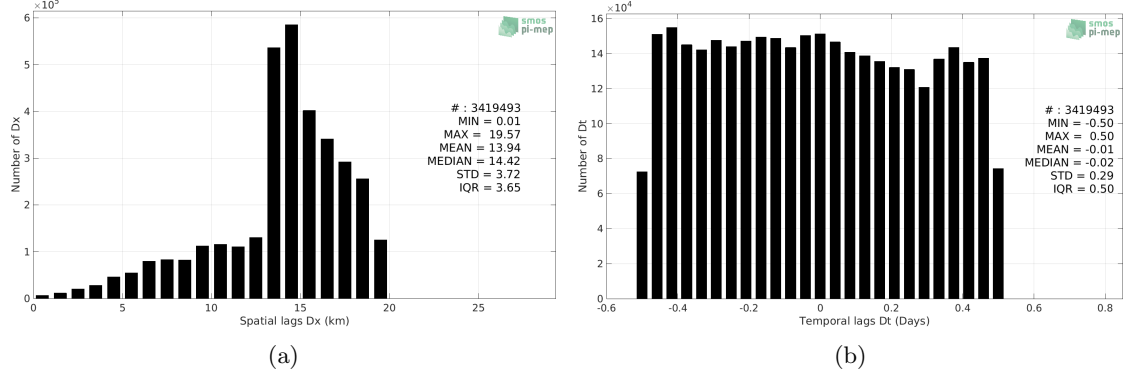
Figure 5: Histograms of the spatial (a) and temporal (b) lags between the time of the Salinity Snake measurements and the date of the corresponding SMAP SSS L3 v4 - 8-Day running (RSS) SSS product.
