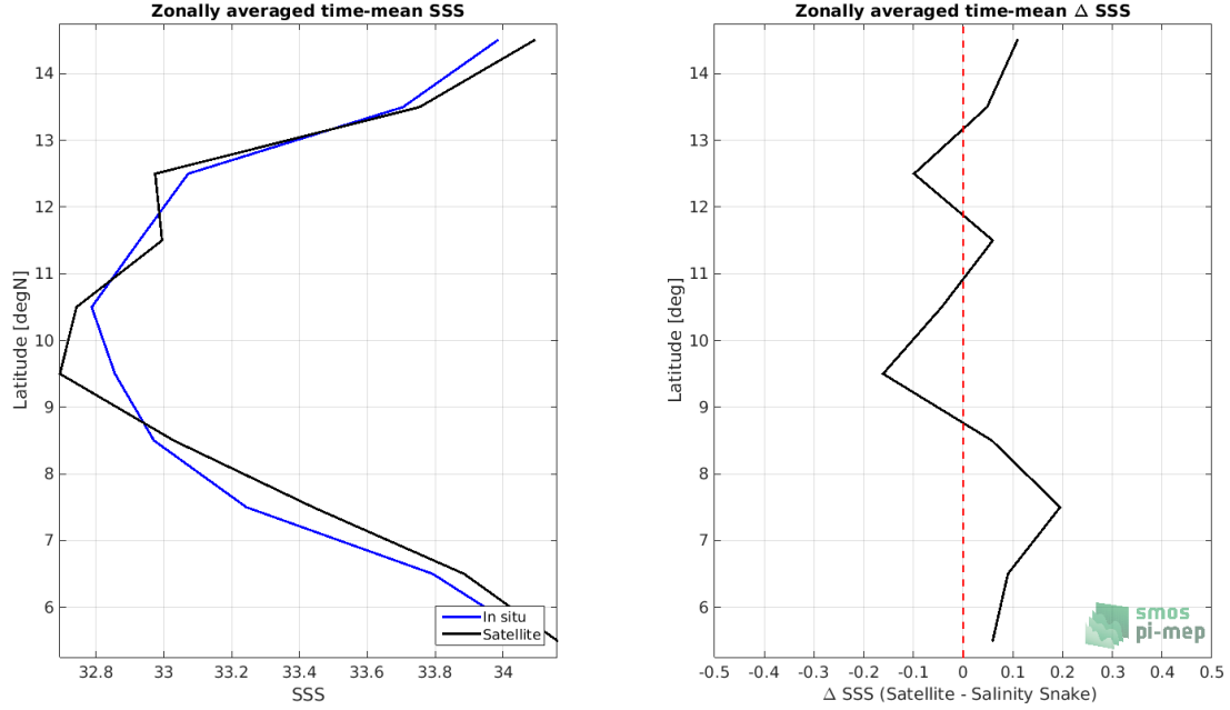
Figure 8: Left panel: Zonal mean SSS from SMAP SSS L3 v4 - 8-Day running (RSS) satellite product (black) and from Salinity Snake (blue). Right panel: Zonal mean of \Delta SSS (Satellite - Salinity Snake) for all the collected Pi-MEP match-up pairs estimated over the full satellite product period.
