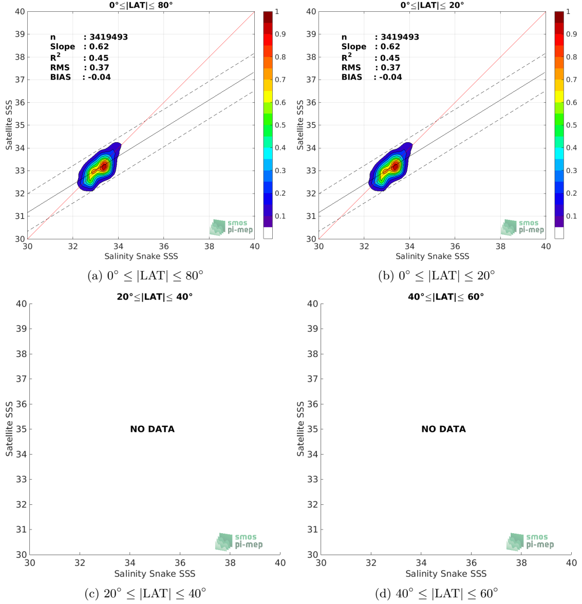
Figure 9: Contour maps of the concentration of SMAP SSS L3 v4 - 8-Day running (RSS) SSS (y-axis) versus Salinity Snake SSS (x-axis) at match-up pairs for different latitude bands. For each plot, the red line shows x=y . The black thin and dashed lines indicate a linear fit through the data cloud and the \pm 95\% confidence levels, respectively. The number match-up pairs n , the slope and R^2 coefficient of the linear fit, the root mean square (RMS) and the mean bias between satellite and in situ data are indicated for each latitude band in each plots.
