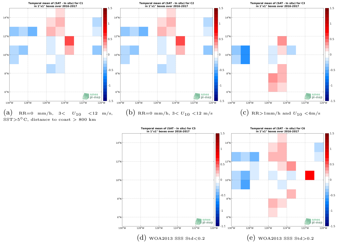
Figure 12: Temporal mean gridded over spatial boxes of size 1^\circ \times 1^\circ of \Delta SSS (SMAP SSS L3 v4 - 8-Day running (RSS) - Salinity Snake) for 5 different subdatasets corresponding to: RR=0 mm/h, 3 < U_{10} < 12 m/s, SST >5^\circ\text{C} , distance to coast > 800 km (a), RR=0 mm/h, 3 < U_{10} < 12 m/s (b), RR >1 mm/h and U_{10} < 4 m/s (c), WOA2013 SSS Std <0.2 (d), WOA2013 SSS Std >0.2 (e).
