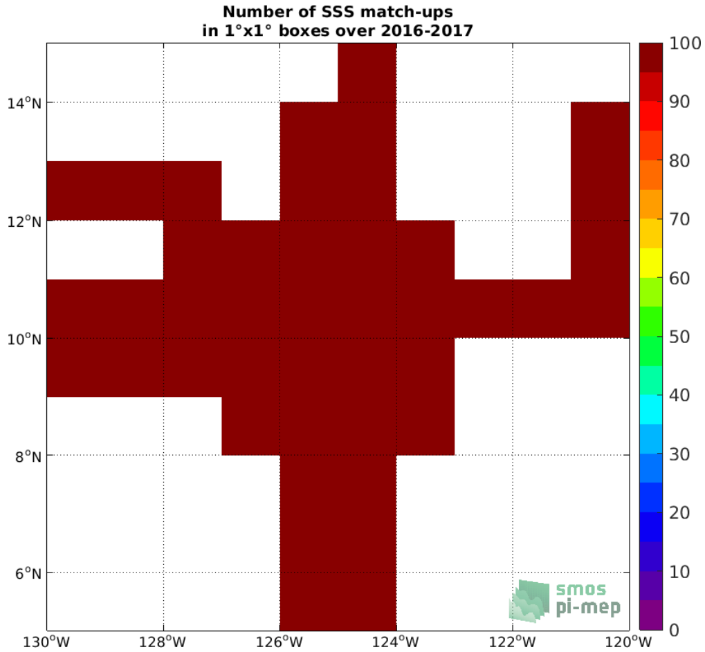
Figure 4: Number of SSS match-ups between Salinity Snake SSS and the SMAP SSS L3 v4 - 8-Day running (RSS) SSS product for the SPURS 2 Pi-MEP region over 1°x1° boxes and for the full satellite product period.
