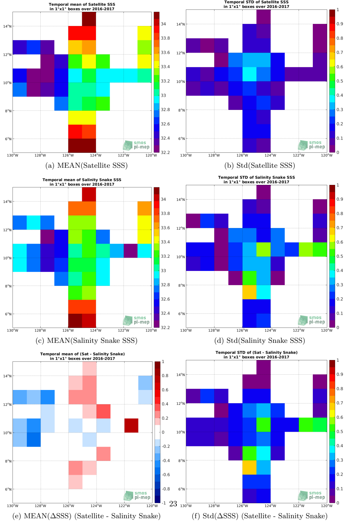
Figure 6: Temporal mean (left) and Std (right) of SSS from SMAP SSS L3 v4 - 8-Day running (RSS) (top), Salinity Snake (middle), and of \Delta SSS (Satellite - Salinity Snake). Only match-up pairs are used to generate these maps.
