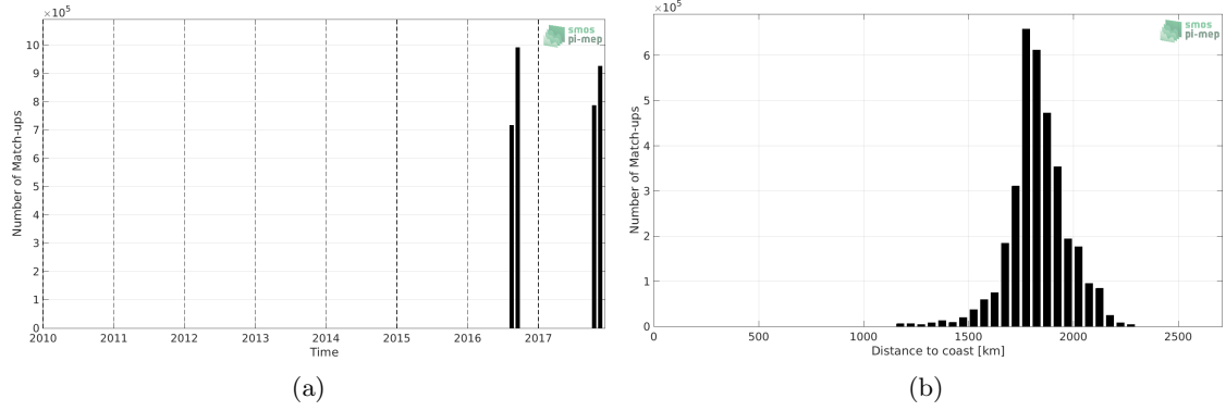
Figure 1: Number of match-ups between Salinity Snake and SMAP SSS L3 v4 - 8-Day running (RSS) SSS as a function of time (a) and as function of the distance to coast (b) over the SPURS 2 Pi-MEP region and for the full satellite product period.
