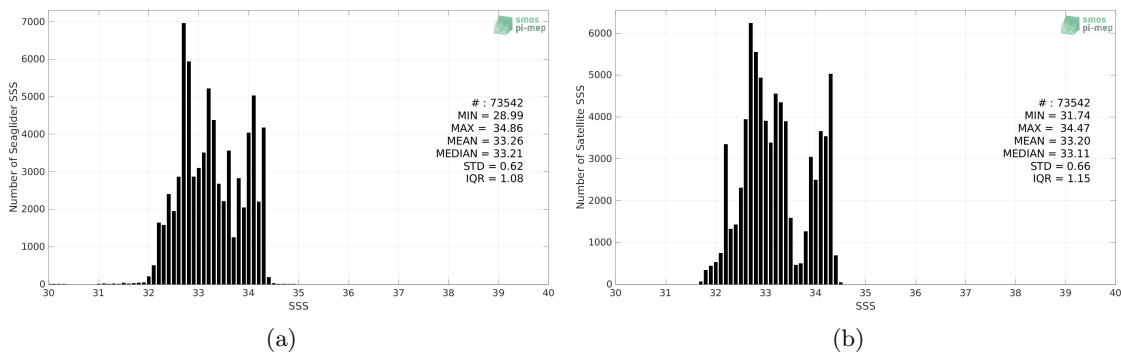
Figure 2: Histograms of SSS from Seagliders (a) and SMAP SSS L3 v4 - 8-Day running (RSS) (b) considering all match-up pairs per bins of 0.1 over the SPURS 2 Pi-MEP region and for the full satellite product period.
