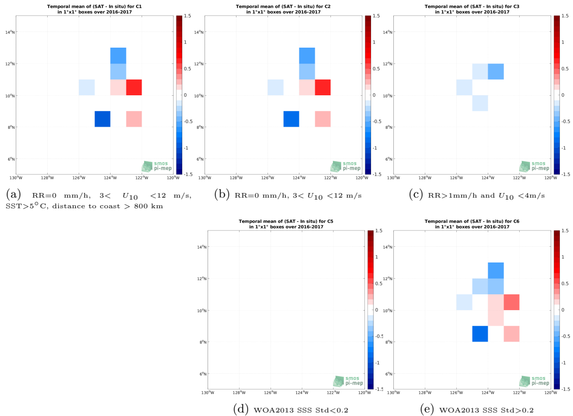
Figure 11: Temporal mean gridded over spatial boxes of size 1^\circ \times 1^\circ of \Delta\text{SSS} (SMAP SSS L3 v4 - 8-Day running (RSS) - Seaglider) for 5 different subdatasets corresponding to:RR=0 mm/h, 3 < U_{10} < 12 m/s, SST >5^\circ\text{C} , distance to coast > 800 km (a), RR=0 mm/h, 3 < U_{10} < 12 m/s (b), RR >1 mm/h and U_{10} < 4 m/s (c), WOA2013 SSS Std <0.2 (d), WOA2013 SSS Std >0.2 (e).
