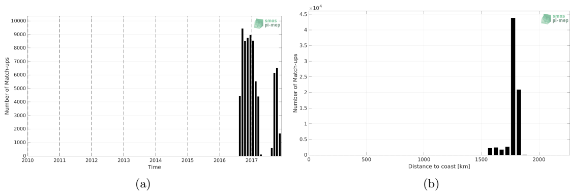
Figure 1: Number of match-ups between Seagliders and SMAP SSS L3 v4 - 8-Day running (RSS) SSS as a function of time (a) and as function of the distance to coast (b) over the SPURS 2 Pi-MEP region and for the full satellite product period.
