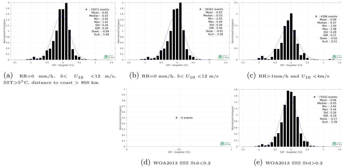
Figure 12: Normalized histogram of \Delta\text{SSS} (SMAP SSS L3 v4 - 8-Day running (RSS) - Seaglider) for 5 different subdatasets corresponding to: RR=0 mm/h, 3 < U_{10} < 12 m/s, SST > 5^\circ\text{C} , distance to coast > 800 km (a), RR=0 mm/h, 3 < U_{10} < 12 m/s (b), RR > 1\text{mm/h} and U_{10} < 4\text{m/s} (c), WOA2013 SSS \text{Std} < 0.2 (d), WOA2013 SSS \text{Std} > 0.2 (e).
