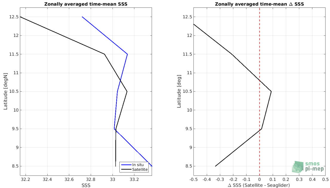
Figure 8: Left panel: Zonal mean SSS from SMAP SSS L3 v4 - 8-Day running (RSS) satellite product (black) and from Seaglider (blue). Right panel: Zonal mean of \Delta SSS (Satellite - Seaglider) for all the collected Pi-MEP match-up pairs estimated over the full satellite product period.
