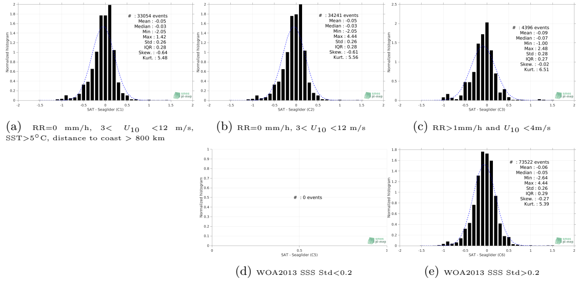
Figure 13: Normalized histogram of \Delta SSS (SMAP SSS L3 v4 - 8-Day running (RSS) - Seaglider) for 5 different subdatasets corresponding to: RR=0 mm/h, 3 < U_{10} < 12 m/s, SST > 5°C, distance to coast > 800 km (a), RR=0 mm/h, 3 < U_{10} < 12 m/s (b), RR > 1mm/h and U_{10} < 4 m/s (c), WOA2013 SSS Std < 0.2 (d), WOA2013 SSS Std > 0.2 (e).
