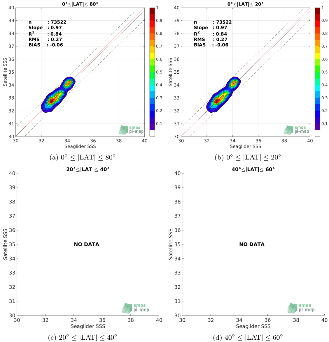
Figure 9: Contour maps of the concentration of SMAP SSS L3 v4 - 8-Day running (RSS) SSS (y-axis) versus Seaglider SSS (x-axis) at match-up pairs for different latitude bands. For each plot, the red line shows x=y . The black thin and dashed lines indicate a linear fit through the data cloud and the \pm 95\% confidence levels, respectively. The number match-up pairs n , the slope and R^2 coefficient of the linear fit, the root mean square (RMS) and the mean bias between satellite and in situ data are indicated for each latitude band in each plots.
