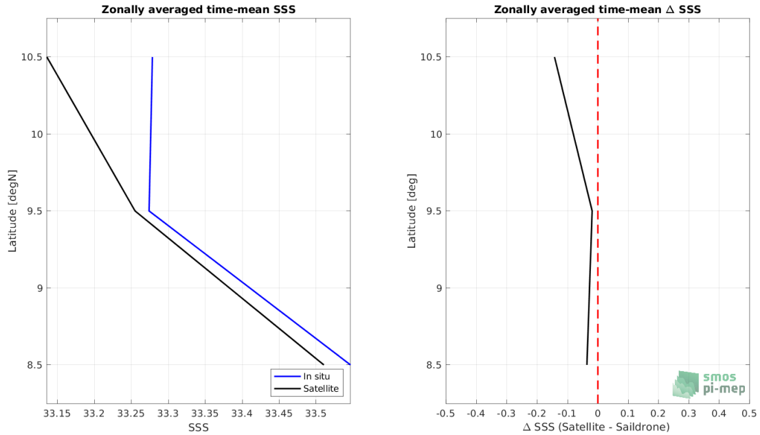
Figure 7: Left panel: Zonal mean SSS from SMAP SSS L3 v4 - 8-Day running (RSS) satellite product (black) and from Sairdrone (blue). Right panel: Zonal mean of \Delta SSS (Satellite - Sairdrone) for all the collected Pi-MEP match-up pairs estimated over the full satellite product period.
