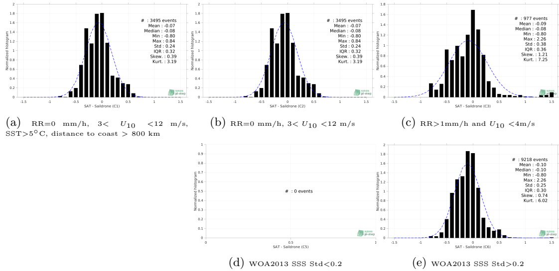
Figure 12: Normalized histogram of \Delta SSS (SMAP SSS L3 v4 - 8-Day running (RSS) - Sairdrone) for 5 different subdatasets corresponding to: RR=0 mm/h, 3 < U_{10} < 12 m/s, SST > 5°C, distance to coast > 800 km (a), RR=0 mm/h, 3 < U_{10} < 12 m/s (b), RR > 1mm/h and U_{10} < 4 m/s (c), WOA2013 SSS Std < 0.2 (d), WOA2013 SSS Std > 0.2 (e).
