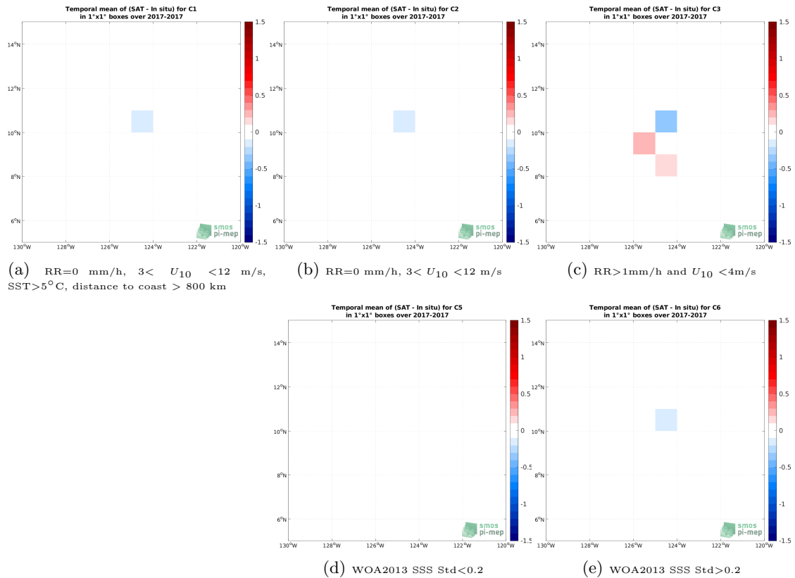
Figure 11: Temporal mean gridded over spatial boxes of size 1^\circ \times 1^\circ of \Delta SSS (SMAP SSS L3 v4 - 8-Day running (RSS) - Saildrone) for 5 different subdatasets corresponding to:RR=0 mm/h, 3 < U_{10} < 12 m/s, SST >5^\circ C, distance to coast > 800 km (a), RR=0 mm/h, 3 < U_{10} < 12 m/s (b), RR >1 mm/h and U_{10} < 4 m/s (c), WOA2013 SSS Std <0.2 (d), WOA2013 SSS Std >0.2 (e).
