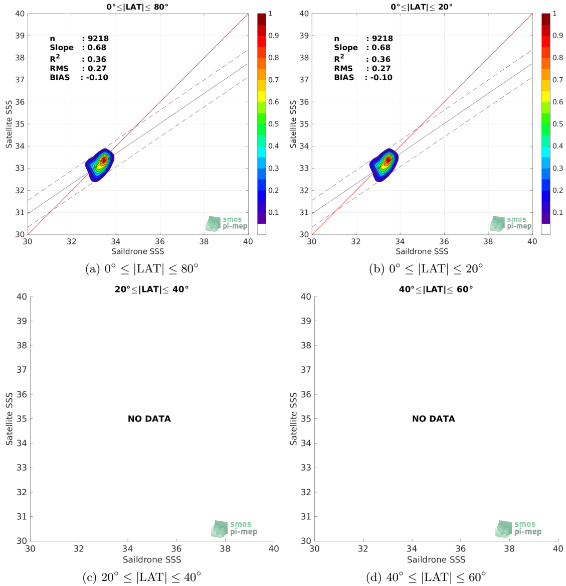
Figure 8: Contour maps of the concentration of SMAP SSS L3 v4 - 8-Day running (RSS) SSS (y-axis) versus Saildrone SSS (x-axis) at match-up pairs for different latitude bands. For each plot, the red line shows x=y . The black thin and dashed lines indicate a linear fit through the data cloud and the \pm 95\% confidence levels, respectively. The number match-up pairs n , the slope and R^2 coefficient of the linear fit, the root mean square (RMS) and the mean bias between satellite and in situ data are indicated for each latitude band in each plots.
