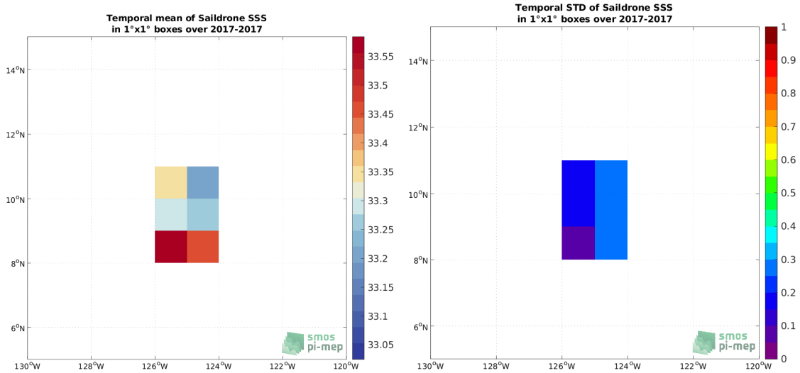
(c) MEAN(Saildrone SSS)
