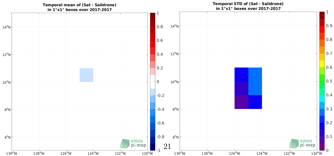
(e) MEAN( \Delta SSS) (Satellite - Saildrone)
