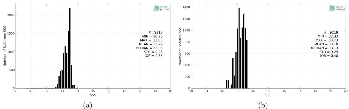
Figure 2: Histograms of SSS from Saildrone (a) and SMAP SSS L3 v4 - 8-Day running (RSS) (b) considering all match-up pairs per bins of 0.1 over the SPURS 2 Pi-MEP region and for the full satellite product period.
