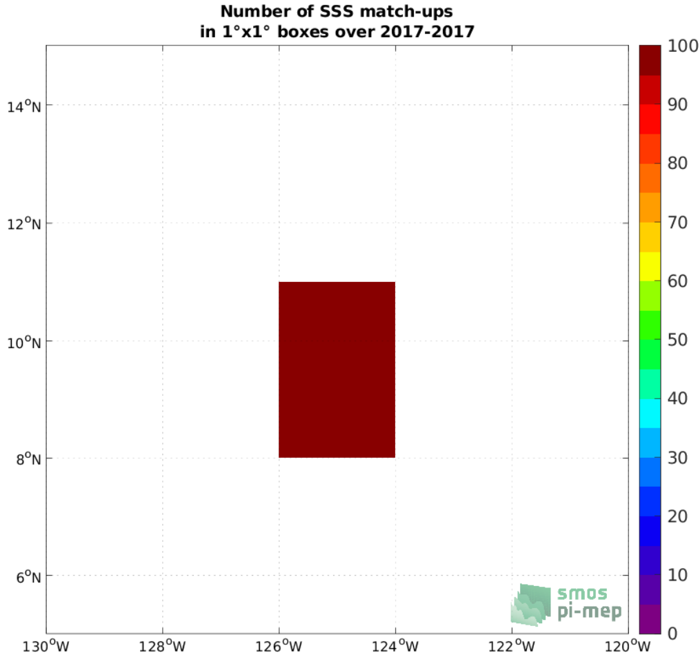
Figure 3: Number of SSS match-ups between Sairdrone SSS and the SMAP SSS L3 v4 - 8-Day running (RSS) SSS product for the SPURS 2 Pi-MEP region over 1^\circ \times 1^\circ boxes and for the full satellite product period.
