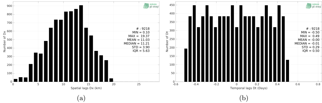
Figure 4: Histograms of the spatial (a) and temporal (b) lags between the location/time of the Smaildrone measurement and the date of the corresponding SMAP SSS L3 v4 - 8-Day running (RSS) SSS pixel.
