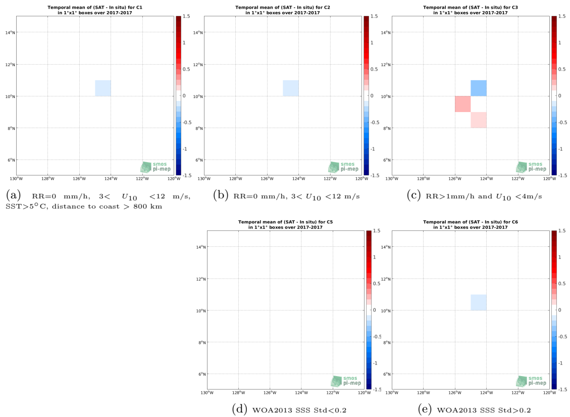
Figure 11: Temporal mean gridded over spatial boxes of size 1^\circ \times 1^\circ of \Delta SSS (SMAP SSS L3 v4 - 8-Day running (RSS) - Sailer) for 5 different subdatasets corresponding to: RR=0 mm/h, 3 < U_{10} < 12 m/s, SST > 5^\circ\text{C} , distance to coast > 800 km (a), RR=0 mm/h, 3 < U_{10} < 12 m/s (b), RR > 1 mm/h and U_{10} < 4 m/s (c), WOA2013 SSS Std < 0.2 (d), WOA2013 SSS Std > 0.2 (e).
