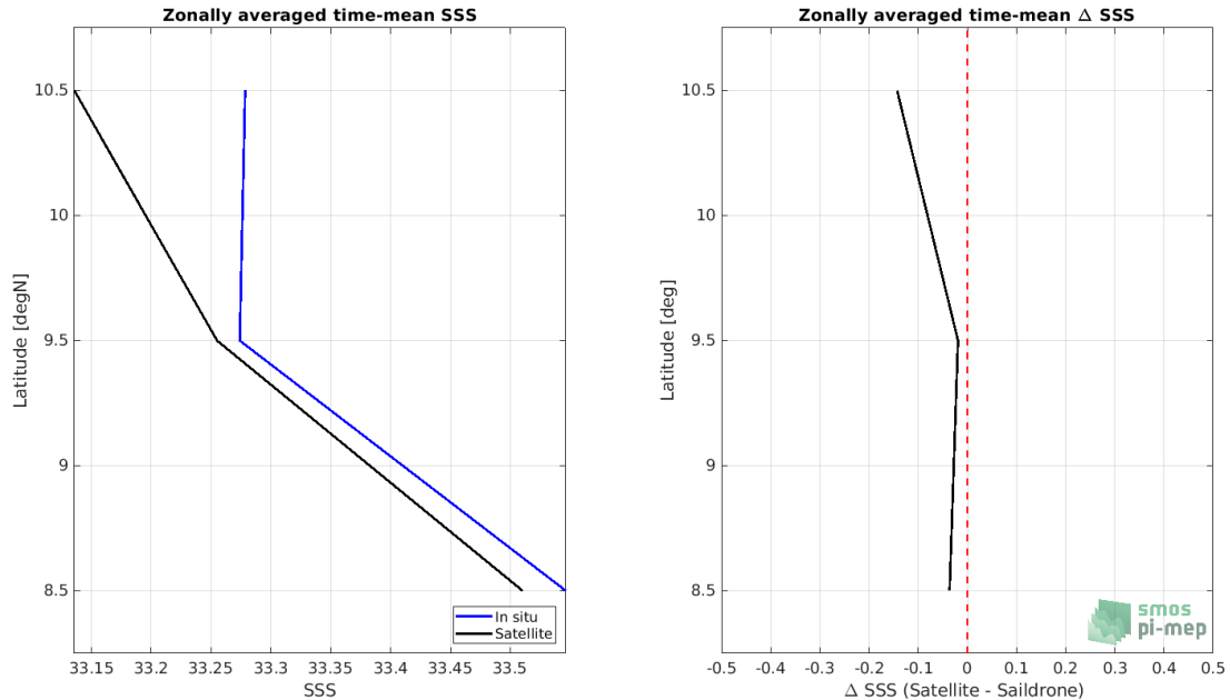
Figure 7: Left panel: Zonal mean SSS from SMAP SSS L3 v4 - 8-Day running (RSS) satellite product (black) and from Saildrone (blue). Right panel: Zonal mean of \Delta SSS (Satellite - Saildrone) for all the collected Pi-MEP match-up pairs estimated over the full satellite product period.
