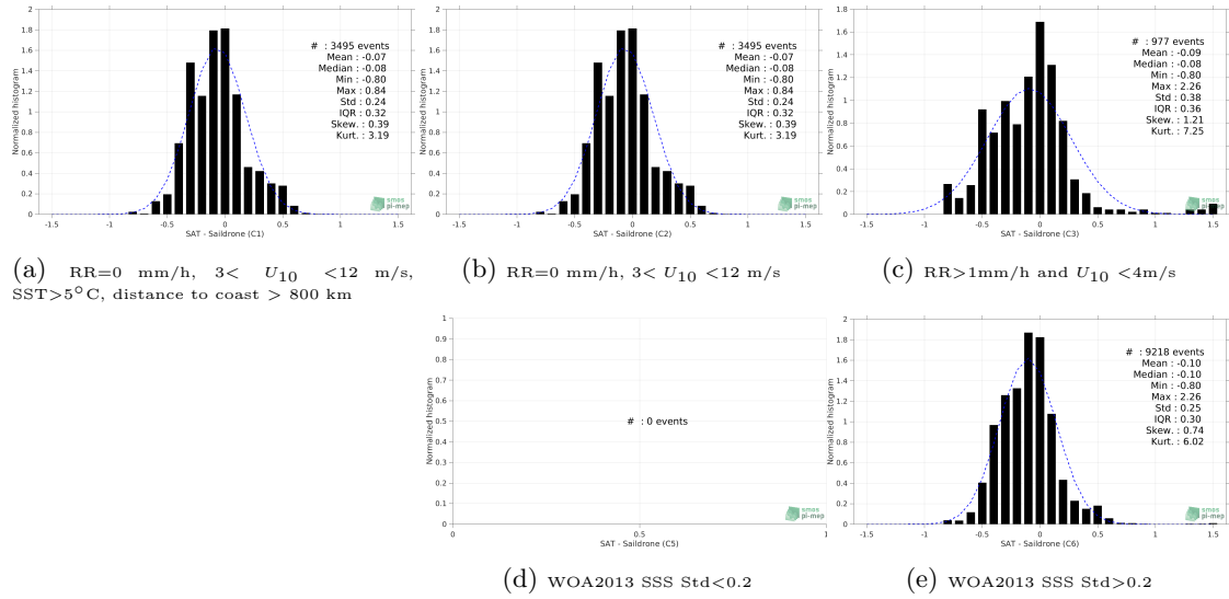
Figure 12: Normalized histogram of \Delta SSS (SMAP SSS L3 v4 - 8-Day running (RSS) - Saildrone) for 5 different subdatasets corresponding to: RR=0 mm/h, 3 < U_{10} < 12 m/s, SST>5°C, distance to coast > 800 km (a), RR=0 mm/h, 3 < U_{10} < 12 m/s (b), RR>1mm/h and U_{10} < 4 m/s (c), WOA2013 SSS Std<0.2 (d), WOA2013 SSS Std>0.2 (e).
