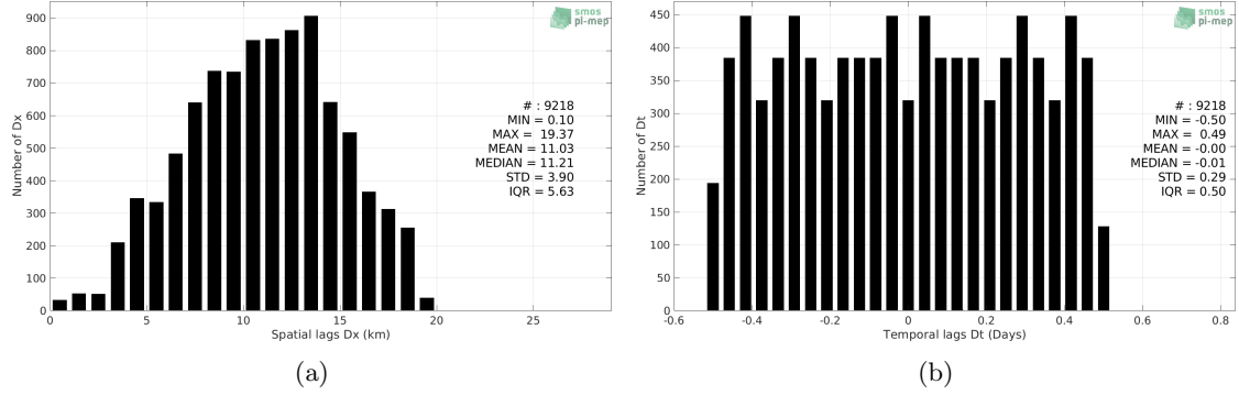
Figure 4: Histograms of the spatial (a) and temporal (b) lags between the location/time of the Saildrone measurement and the date of the corresponding SMAP SSS L3 v4 - 8-Day running (RSS) SSS pixel.
