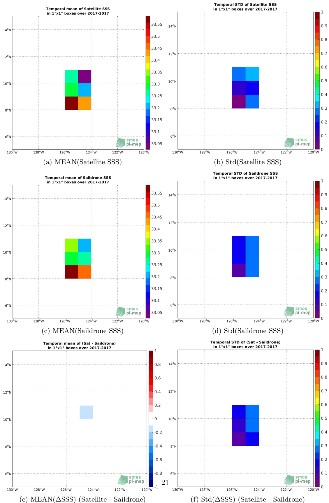
Figure 5: Temporal mean (left) and Std (right) of SSS from SMAP SSS L3 v4 - 8-Day running (RSS) (top), Saildrone (middle), and of \Delta SSS (Satellite - Saildrone). Only match-up pairs are used to generate these maps.
