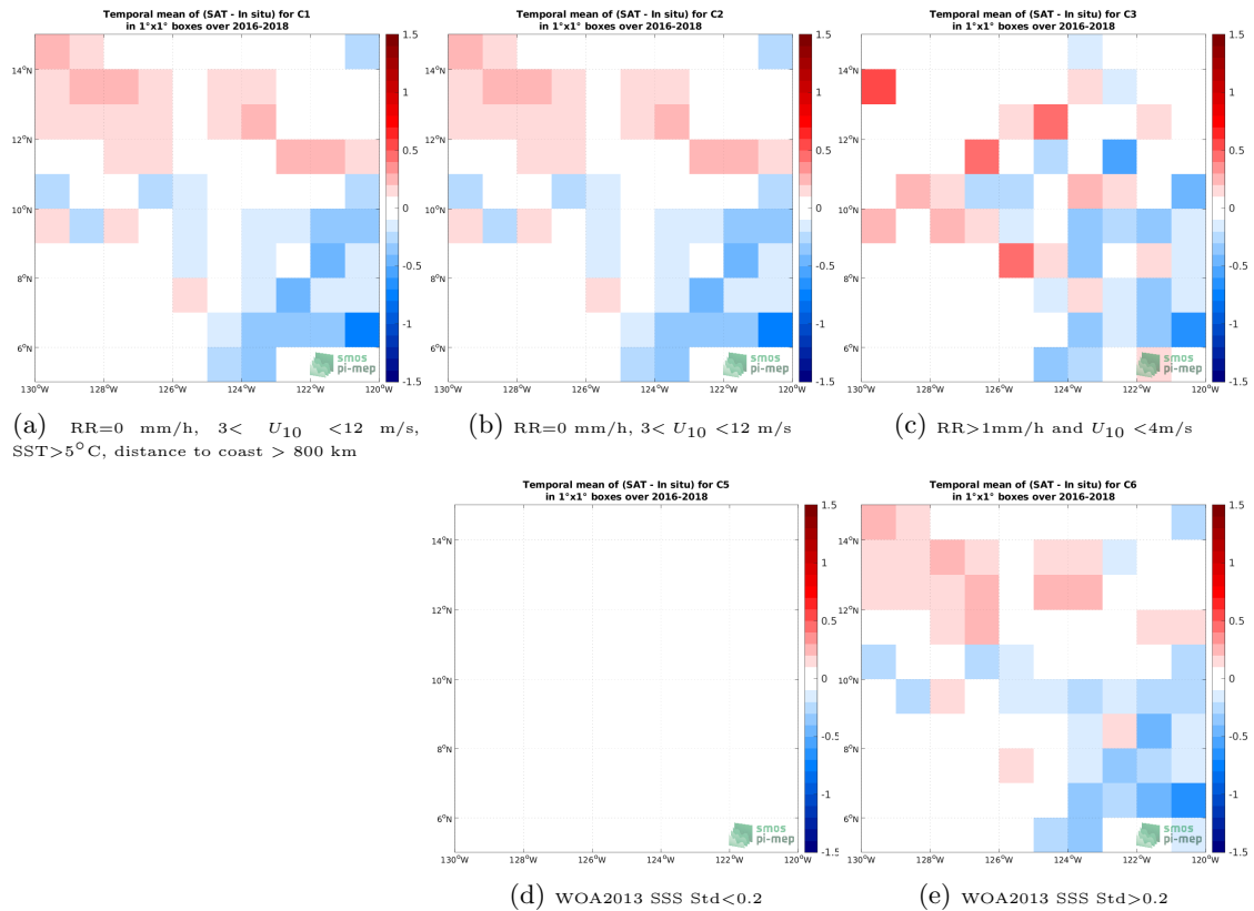
Figure 11: Temporal mean gridded over spatial boxes of size 1^\circ \times 1^\circ of \Delta SSS (SMAP SSS L3 v4 - 8-Day running (RSS) - Surface drifters) for 5 different subdatasets corresponding to:RR=0 mm/h, 3 < U_{10} < 12 m/s, SST > 5^\circ\text{C} , distance to coast > 800 km (a), RR=0 mm/h, 3 < U_{10} < 12 m/s (b), RR > 1 mm/h and U_{10} < 4 m/s (c), WOA2013 SSS Std < 0.2 (d), WOA2013 SSS Std > 0.2 (e).
