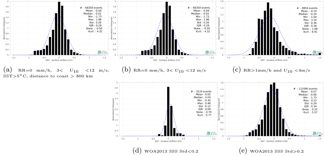
Figure 12: Normalized histogram of \Delta SSS (SMAP SSS L3 v4 - 8-Day running (RSS) - Surface drifters) for 5 different subdatasets corresponding to: RR=0 mm/h, 3 < U_{10} < 12 m/s, SST > 5°C, distance to coast > 800 km (a), RR=0 mm/h, 3 < U_{10} < 12 m/s (b), RR > 1mm/h and U_{10} < 4 m/s (c), WOA2013 SSS Std < 0.2 (d), WOA2013 SSS Std > 0.2 (e).
