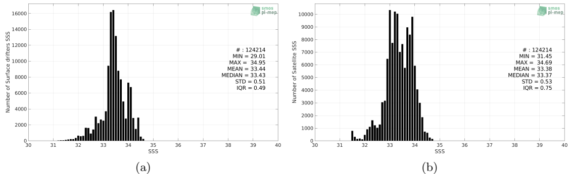
Figure 2: Histograms of SSS from Surface drifters (a) and SMAP SSS L3 v4 - 8-Day running (RSS) (b) considering all match-up pairs per bins of 0.1 over the SPURS 2 Pi-MEP region and for the full satellite product period.
