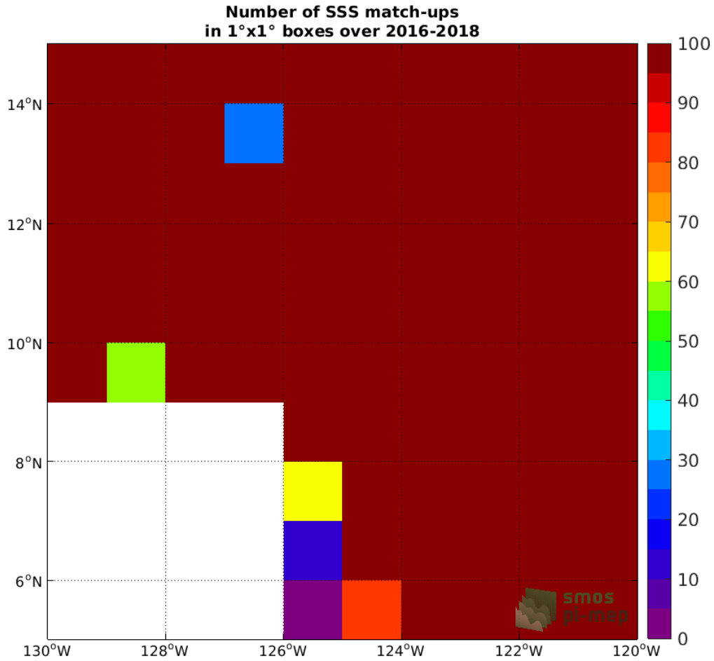
Figure 3: Number of SSS match-ups between Surface drifters SSS and the SMAP SSS L3 v4 - 8-Day running (RSS) SSS product for the SPURS 2 Pi-MEP region over 1°x1° boxes and for the full satellite product period.
