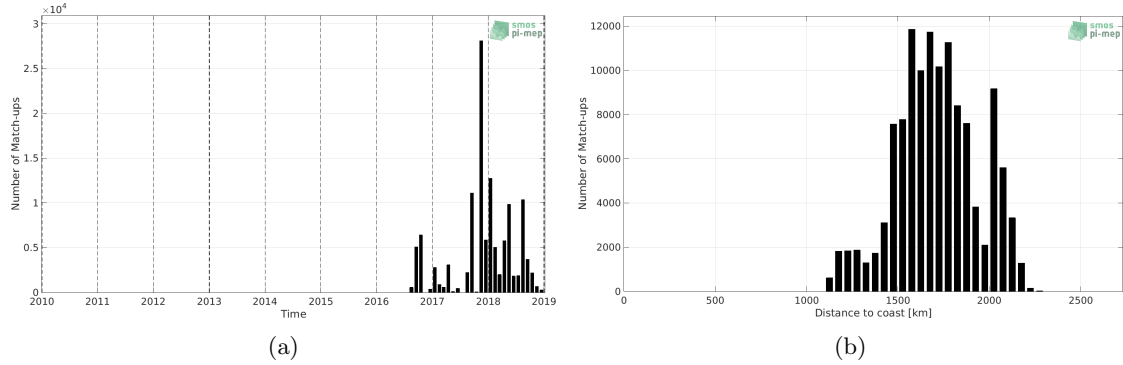
Figure 1: Number of match-ups between Surface drifters and SMAP SSS L3 v4 - 8-Day running (RSS) SSS as a function of time (a) and as function of the distance to coast (b) over the SPURS 2 Pi-MEP region and for the full satellite product period.
