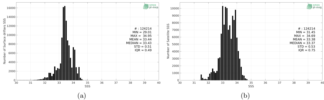
Figure 2: Histograms of SSS from Surface drifters (a) and SMAP SSS L3 v4 - 8-Day running (RSS) (b) considering all match-up pairs per bins of 0.1 over the SPURS 2 Pi-MEP region and for the full satellite product period.
