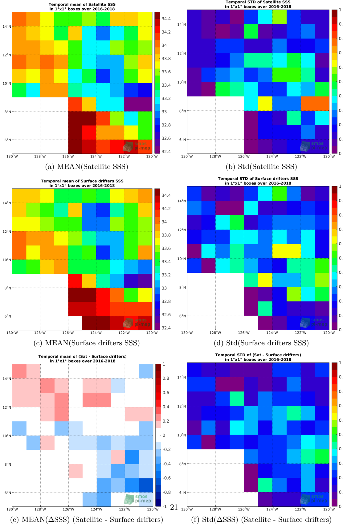
Figure 5: Temporal mean (left) and Std (right) of SSS from SMAP SSS L3 v4 - 8-Day running (RSS) (top), Surface drifters (middle), and of \Delta SSS (Satellite - Surface drifters). Only match-up pairs are used to generate these maps.
