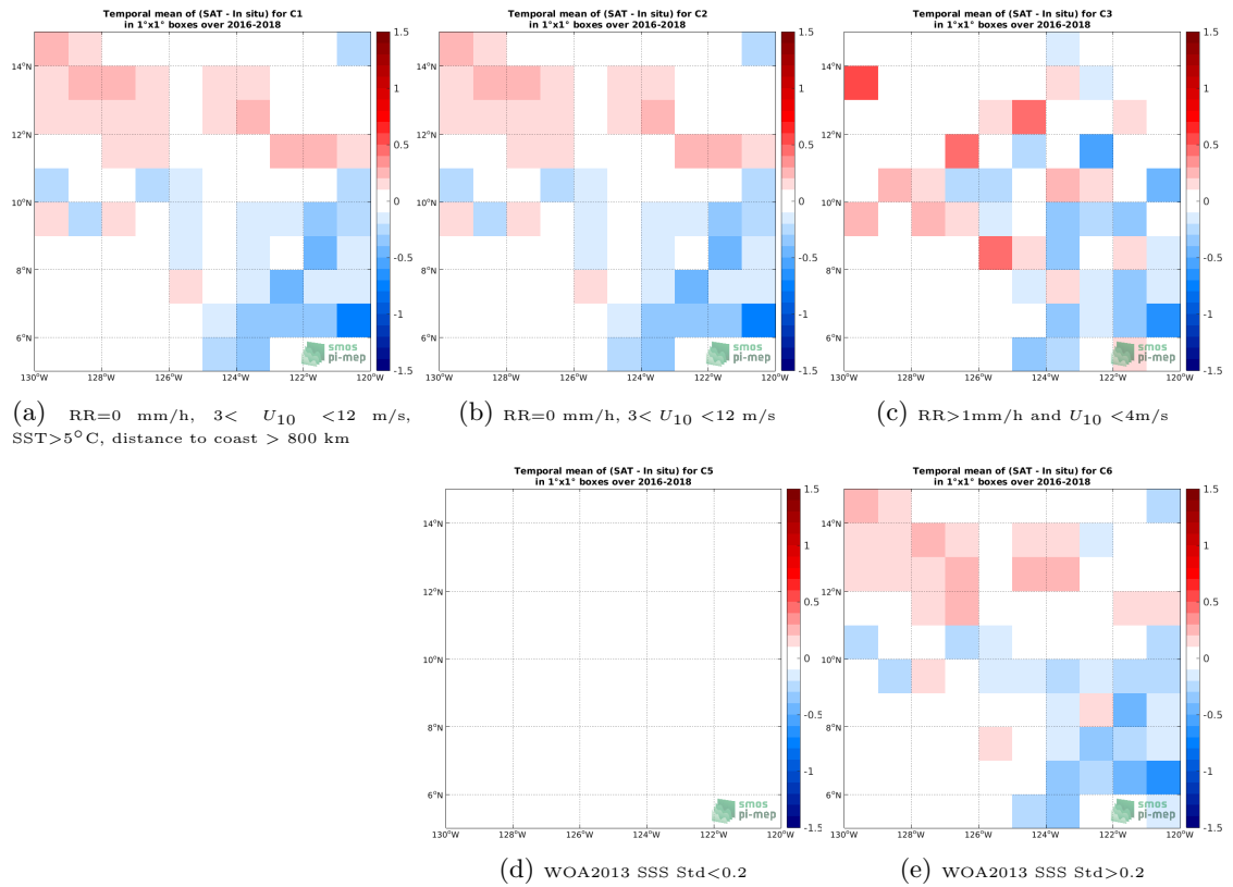
Figure 11: Temporal mean gridded over spatial boxes of size 1^\circ \times 1^\circ of \Delta SSS (SMAP SSS L3 v4 - 8-Day running (RSS) - Surface drifters) for 5 different subdatasets corresponding to:RR=0 mm/h, 3 < U_{10} < 12 m/s, SST >5^\circ\text{C} , distance to coast > 800 km (a), RR=0 mm/h, 3 < U_{10} < 12 m/s (b), RR >1 mm/h and U_{10} < 4 m/s (c), WOA2013 SSS Std <0.2 (d), WOA2013 SSS Std >0.2 (e).
