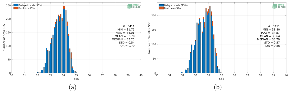
Figure 2: Histograms of SSS from Argo (a) and SMAP SSS L3 v4 - 8-Day running (RSS) (b) considering all match-up pairs per bins of 0.1 over the SPURS 2 Pi-MEP region and for the full satellite product period.
