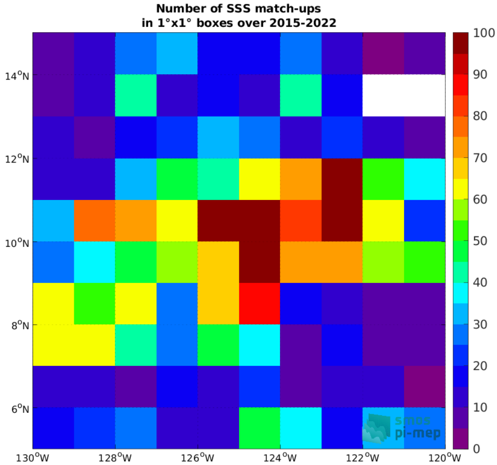
Figure 4: Number of SSS match-ups between Argo SSS and the SMAP SSS L3 v4 - 8-Day running (RSS) SSS product for the SPURS 2 Pi-MEP region over 1°x1° boxes and for the full satellite product period.
