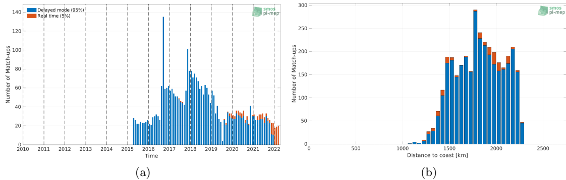
Figure 1: Number of match-ups between Argo and SMAP SSS L3 v4 - 8-Day running (RSS) SSS as a function of time (a) and as function of the distance to coast (b) over the SPURS 2 Pi-MEP region and for the full satellite product period.
