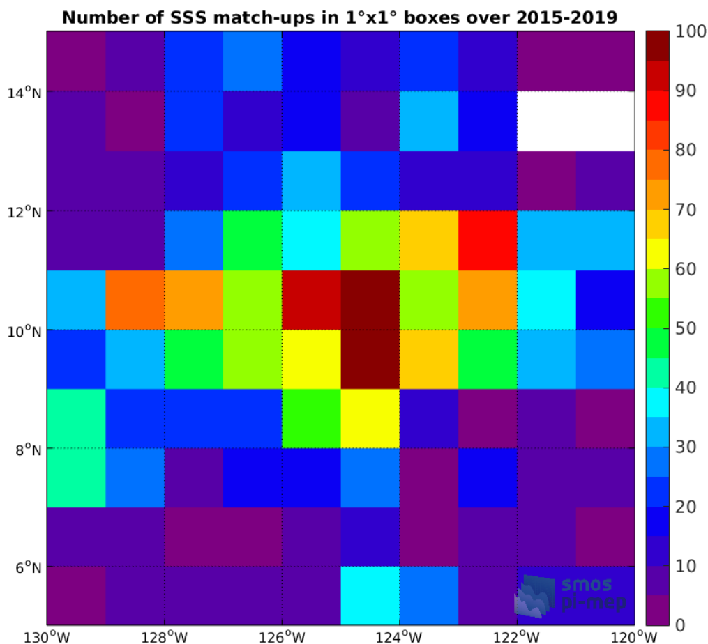
Figure 4: Number of SSS match-ups between Argo SSS and the SMAP-L3-RSS-V4-8DAY-RUNNING SSS product for the SPURS 2 Pi-MEP region over 1°x1° boxes and for the full satellite product period.
