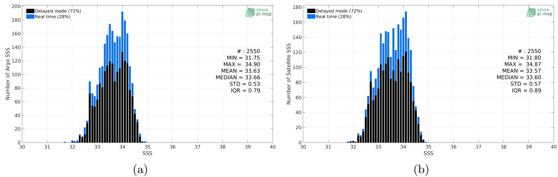
Figure 2: Histograms of SSS from Argo (a) and SMAP-L3-RSS-V4-8DAY-RUNNING (b) considering all match-up pairs per bins of 0.1 over the SPURS 2 Pi-MEP region and for the full satellite product period.
