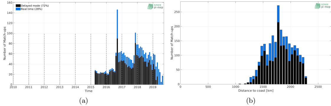
Figure 1: Number of match-ups between Argo and SMAP-L3-RSS-V4-8DAY-RUNNING SSS as a function of time (a) and as function of the distance to coast (b) over the SPURS 2 Pi-MEP region and for the full satellite product period.
