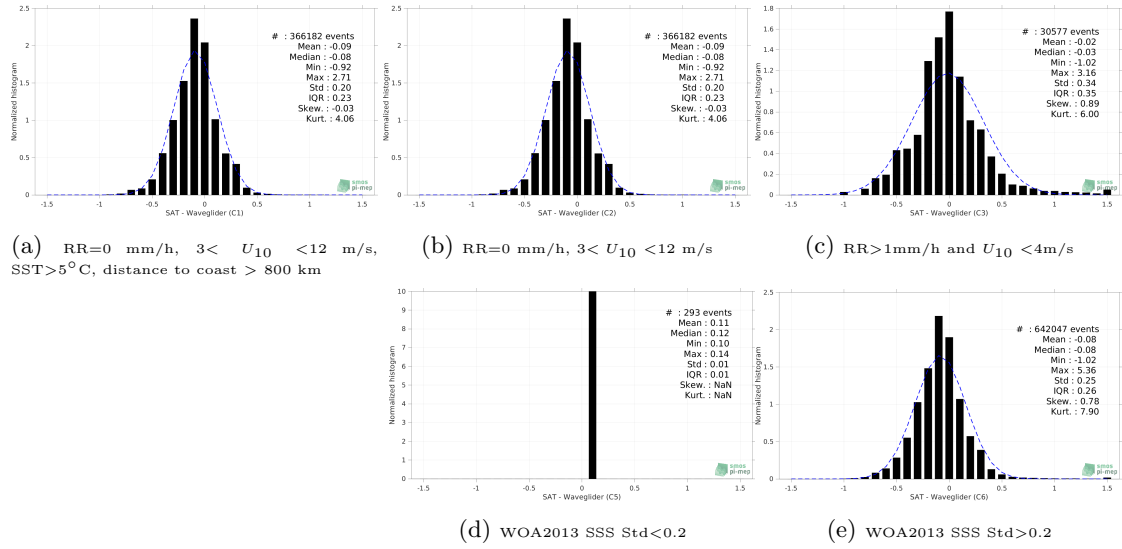
Figure 12: Normalized histogram of \Delta SSS (SMAP SSS L3 v4 - Monthly (RSS) - Waveglider) for 5 different subdatasets corresponding to: RR=0 mm/h, 3 < U_{10} < 12 m/s, SST > 5°C, distance to coast > 800 km (a), RR=0 mm/h, 3 < U_{10} < 12 m/s (b), RR > 1mm/h and U_{10} < 4 m/s (c), WOA2013 SSS Std < 0.2 (d), WOA2013 SSS Std > 0.2 (e).
