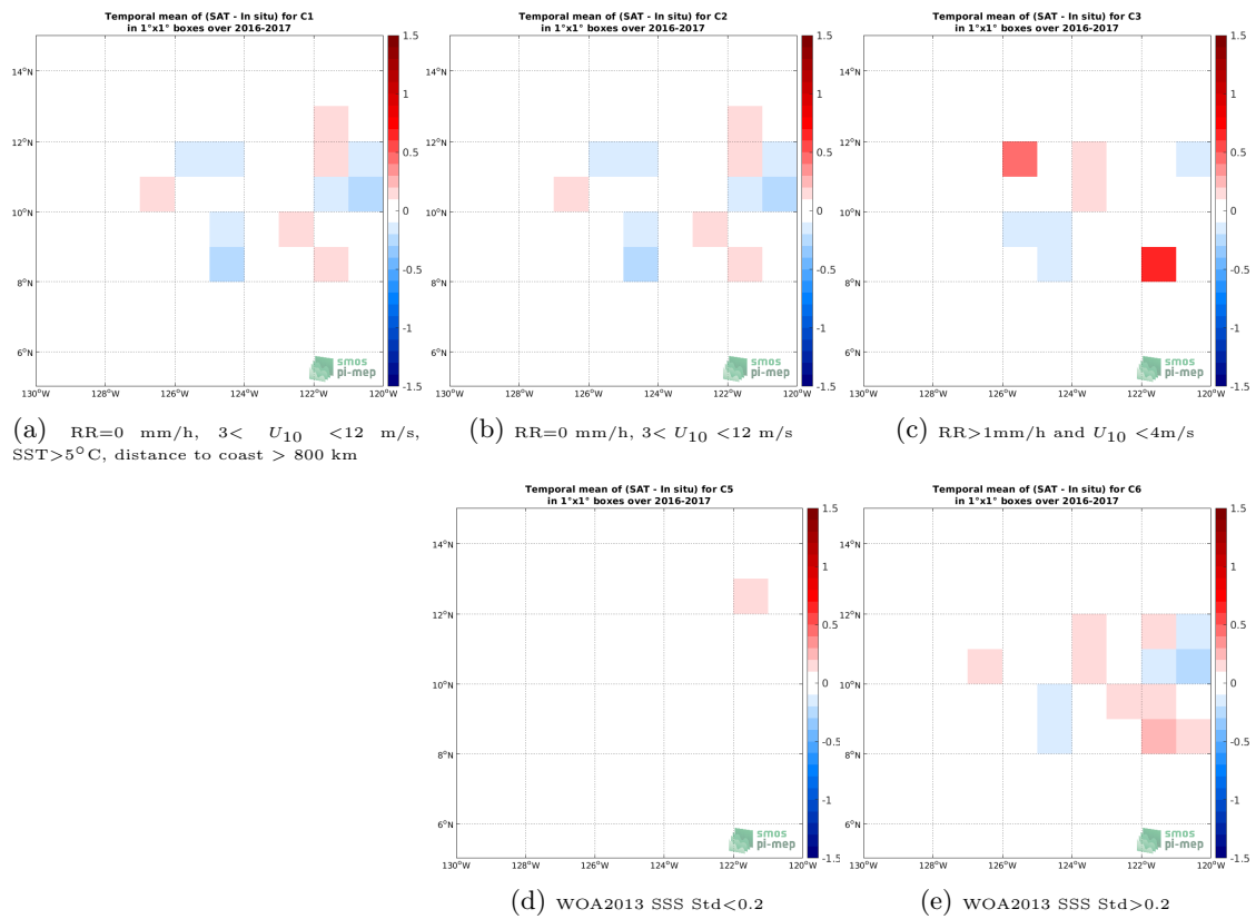
Figure 11: Temporal mean gridded over spatial boxes of size 1^\circ \times 1^\circ of \Delta SSS (SMAP SSS L3 v4 - Monthly (RSS) - Waveglider) for 5 different subdatasets corresponding to:RR=0 mm/h, 3 < U_{10} < 12 m/s, SST >5^\circ\text{C} , distance to coast > 800 km (a), RR=0 mm/h, 3 < U_{10} < 12 m/s (b), RR >1 mm/h and U_{10} < 4 m/s (c), WOA2013 SSS Std <0.2 (d), WOA2013 SSS Std >0.2 (e).
