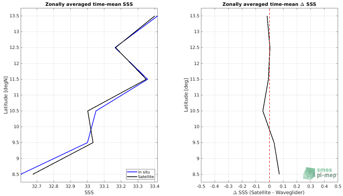
Figure 7: Left panel: Zonal mean SSS from SMAP SSS L3 v4 - Monthly (RSS) satellite product (black) and from Waveglider (blue). Right panel: Zonal mean of \Delta SSS (Satellite - Waveglider) for all the collected Pi-MEP match-up pairs estimated over the full satellite product period.
