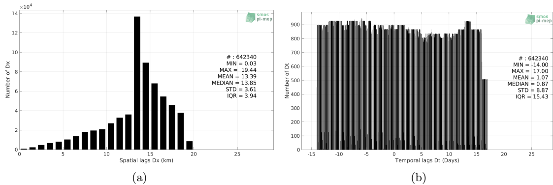
Figure 4: Histograms of the spatial (a) and temporal (b) lags between the location/time of the Waveglider measurement and the date of the corresponding SMAP SSS L3 v4 - Monthly (RSS) SSS pixel.
