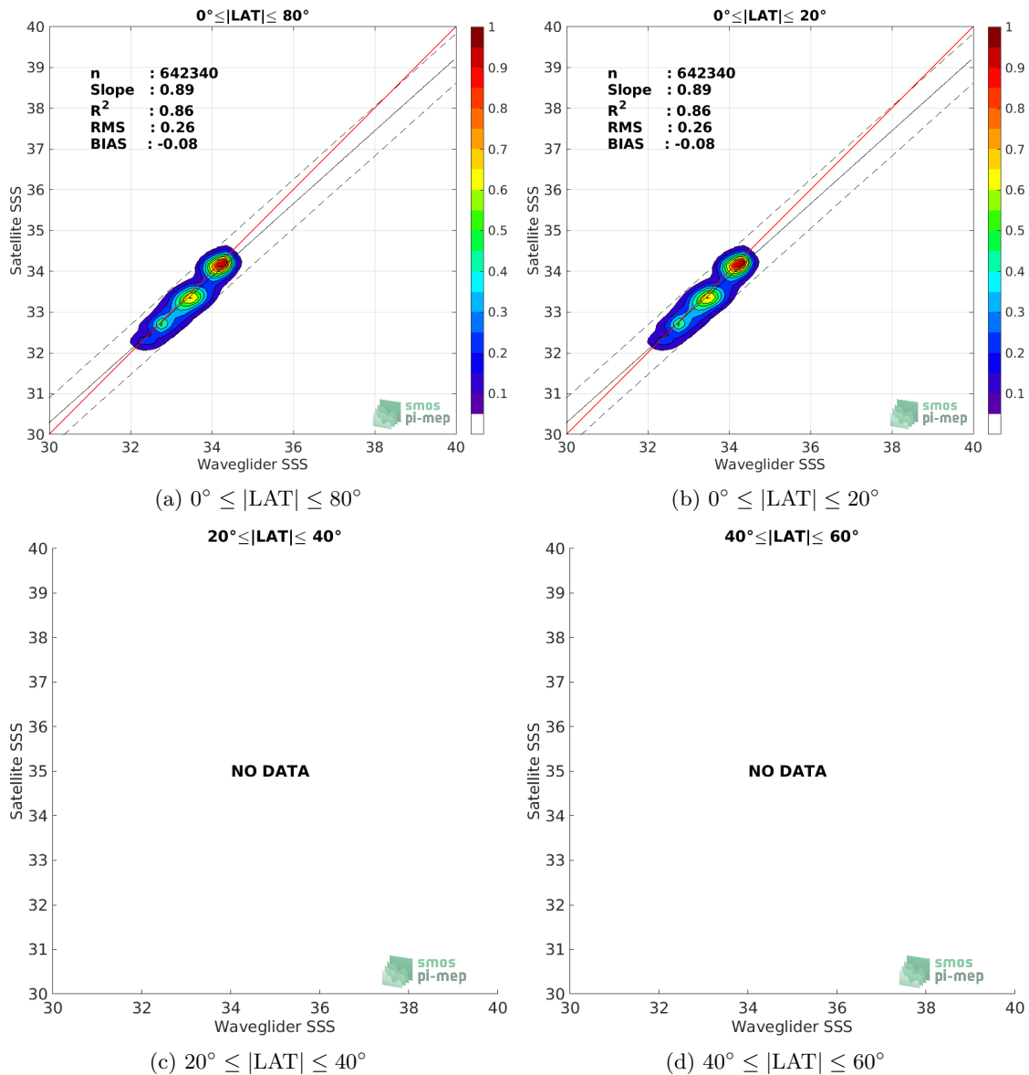
Figure 8: Contour maps of the concentration of SMAP SSS L3 v4 - Monthly (RSS) SSS (y-axis) versus Waveglider SSS (x-axis) at match-up pairs for different latitude bands. For each plot, the red line shows x=y . The black thin and dashed lines indicate a linear fit through the data cloud and the \pm 95\% confidence levels, respectively. The number match-up pairs n , the slope and R^2 coefficient of the linear fit, the root mean square (RMS) and the mean bias between satellite and in situ data are indicated for each latitude band in each plots.
