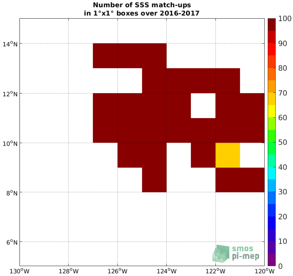
Figure 3: Number of SSS match-ups between Waveglider SSS and the SMAP SSS L3 v4 - Monthly (RSS) SSS product for the SPURS 2 Pi-MEP region over 1^\circ \times 1^\circ boxes and for the full satellite product period.
