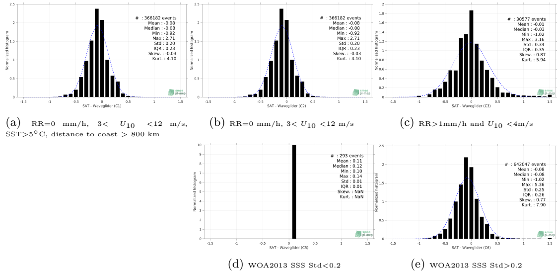
Figure 12: Normalized histogram of \Delta\text{SSS} (SMAP SSS L3 v4 - Monthly (RSS) - Waveglider) for 5 different subdatasets corresponding to: RR=0 mm/h, 3 < U_{10} < 12 m/s, SST > 5^\circ\text{C} , distance to coast > 800 km (a), RR=0 mm/h, 3 < U_{10} < 12 m/s (b), RR > 1\text{mm/h} and U_{10} < 4\text{m/s} (c), WOA2013 SSS Std < 0.2 (d), WOA2013 SSS Std > 0.2 (e).
