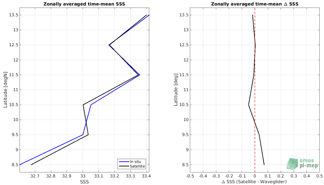
Figure 8: Left panel: Zonal mean SSS from SMAP SSS L3 v4 - Monthly (RSS) satellite product (black) and from Waveglider (blue). Right panel: Zonal mean of \Delta SSS (Satellite - Waveglider) for all the collected Pi-MEP match-up pairs estimated over the full satellite product period.
