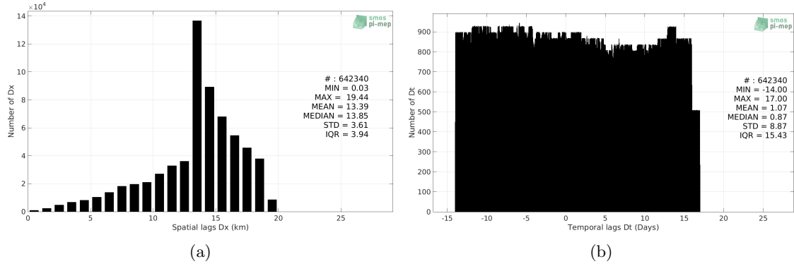
Figure 5: Histograms of the spatial (a) and temporal (b) lags between the time of the Waveglider measurements and the date of the corresponding SMAP SSS L3 v4 - Monthly (RSS) SSS product.
