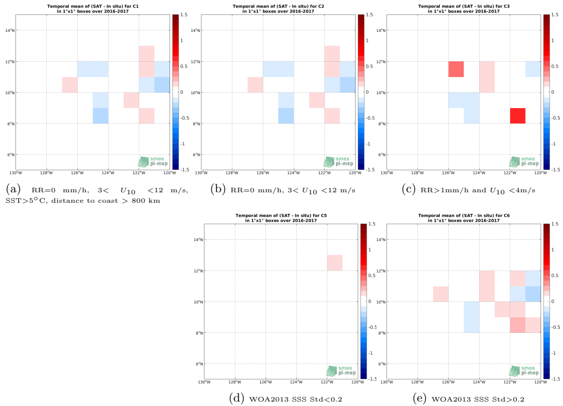
Figure 12: Temporal mean gridded over spatial boxes of size 1^\circ \times 1^\circ of \Delta SSS (SMAP SSS L3 v4 - Monthly (RSS) - Waveglider) for 5 different subdatasets corresponding to: RR=0 mm/h, 3 < U_{10} < 12 m/s, SST > 5^\circ C , distance to coast > 800 km (a), RR=0 mm/h, 3 < U_{10} < 12 m/s (b), RR > 1 mm/h and U_{10} < 4 m/s (c), WOA2013 SSS Std < 0.2 (d), WOA2013 SSS Std > 0.2 (e).
