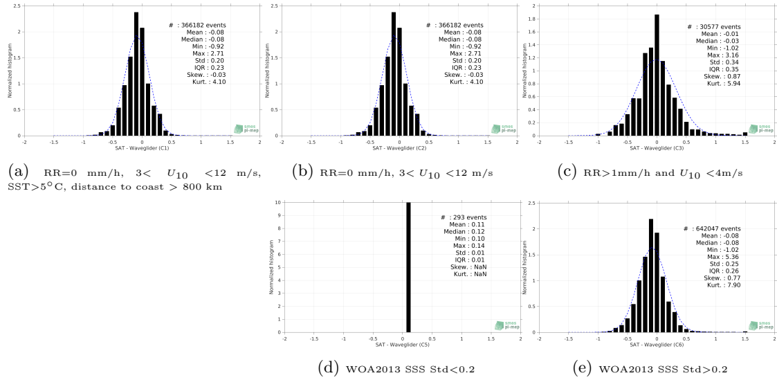
Figure 13: Normalized histogram of \Delta SSS (SMAP SSS L3 v4 - Monthly (RSS) - Waveglider) for 5 different subdatasets corresponding to: RR=0 mm/h, 3 < U_{10} < 12 m/s, SST>5°C, distance to coast > 800 km (a), RR=0 mm/h, 3 < U_{10} < 12 m/s (b), RR>1mm/h and U_{10} < 4 m/s (c), WOA2013 SSS Std<0.2 (d), WOA2013 SSS Std>0.2 (e).
