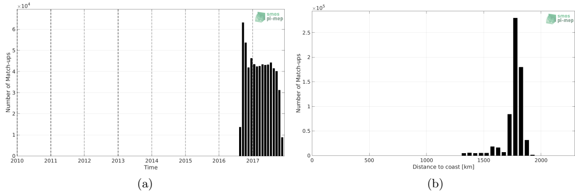
Figure 1: Number of match-ups between Waveglider and SMAP SSS L3 v4 - Monthly (RSS) SSS as a function of time (a) and as function of the distance to coast (b) over the SPURS 2 Pi-MEP region and for the full satellite product period.
