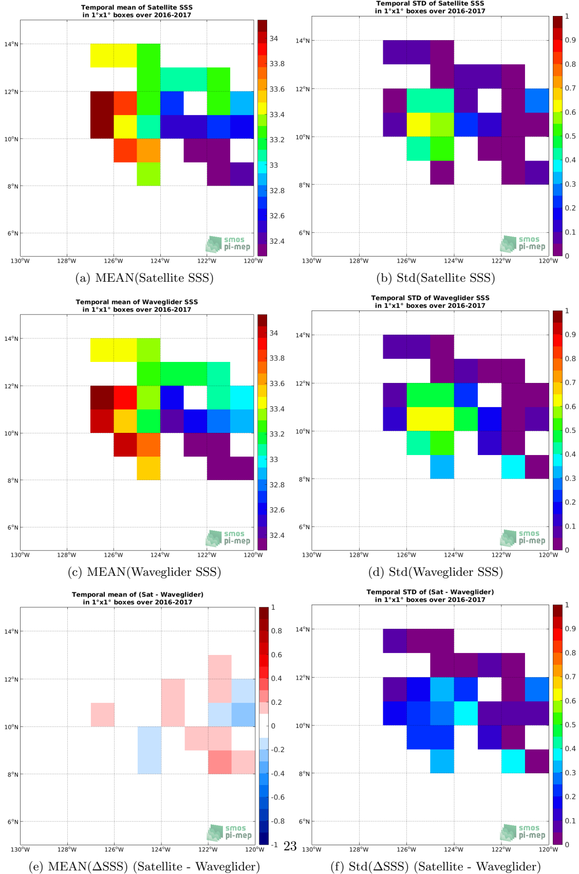
Figure 6: Temporal mean (left) and Std (right) of SSS from SMAP SSS L3 v4 - Monthly (RSS) (top), Waveglider (middle), and of \Delta SSS (Satellite - Waveglider). Only match-up pairs are used to generate these maps.
