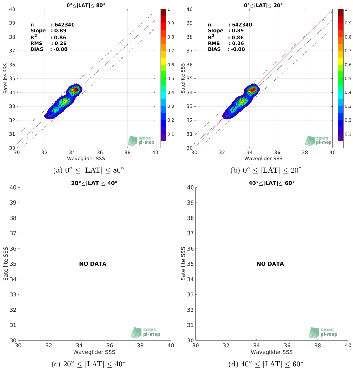
Figure 9: Contour maps of the concentration of SMAP SSS L3 v4 - Monthly (RSS) SSS (y-axis) versus Waveglider SSS (x-axis) at match-up pairs for different latitude bands. For each plot, the red line shows x=y . The black thin and dashed lines indicate a linear fit through the data cloud and the \pm 95\% confidence levels, respectively. The number match-up pairs n , the slope and R^2 coefficient of the linear fit, the root mean square (RMS) and the mean bias between satellite and in situ data are indicated for each latitude band in each plots.
