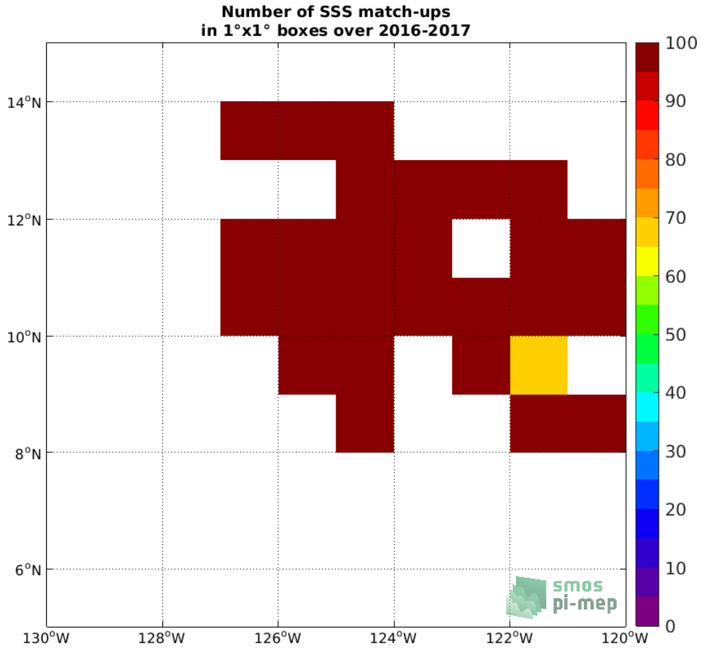
Figure 4: Number of SSS match-ups between Waveglider SSS and the SMAP SSS L3 v4 - Monthly (RSS) SSS product for the SPURS 2 Pi-MEP region over 1°x1° boxes and for the full satellite product period.
