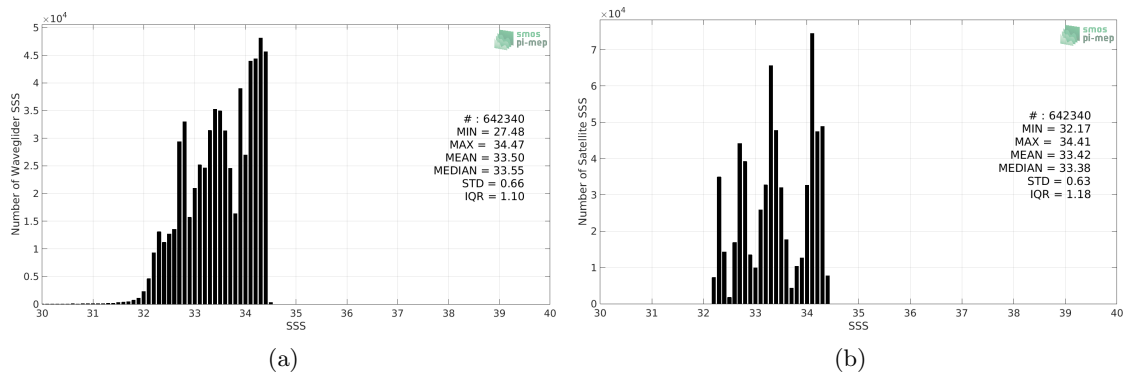
Figure 2: Histograms of SSS from Waveglider (a) and SMAP SSS L3 v4 - Monthly (RSS) (b) considering all match-up pairs per bins of 0.1 over the SPURS 2 Pi-MEP region and for the full satellite product period.
