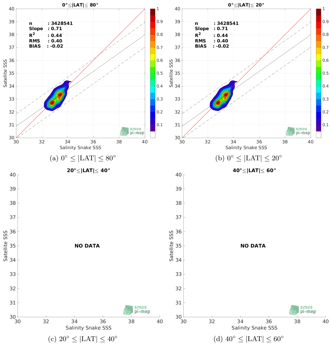
Figure 8: Contour maps of the concentration of SMAP SSS L3 v4 - Monthly (RSS) SSS (y-axis) versus Salinity Snake SSS (x-axis) at match-up pairs for different latitude bands. For each plot, the red line shows x=y . The black thin and dashed lines indicate a linear fit through the data cloud and the \pm 95\% confidence levels, respectively. The number match-up pairs n , the slope and R^2 coefficient of the linear fit, the root mean square (RMS) and the mean bias between satellite and in situ data are indicated for each latitude band in each plots.
