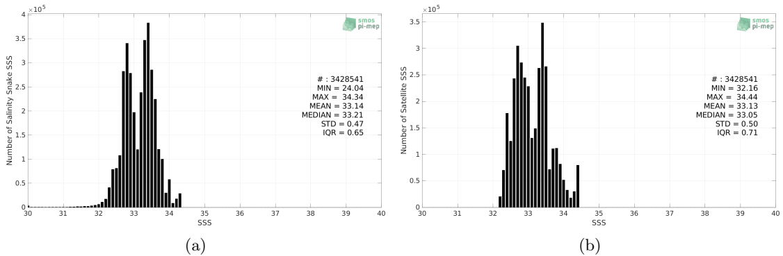
Figure 2: Histograms of SSS from Salinity Snake (a) and SMAP SSS L3 v4 - Monthly (RSS) (b) considering all match-up pairs per bins of 0.1 over the SPURS 2 Pi-MEP region and for the full satellite product period.
