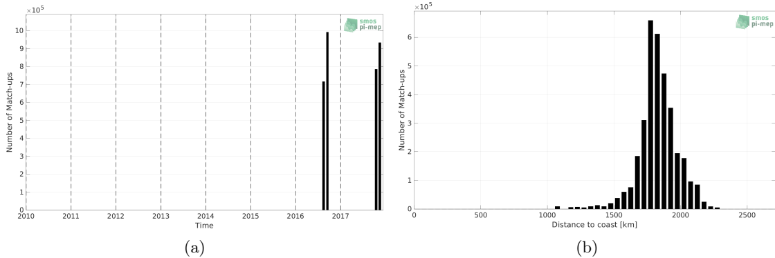
Figure 1: Number of match-ups between Salinity Snake and SMAP SSS L3 v4 - Monthly (RSS) SSS as a function of time (a) and as function of the distance to coast (b) over the SPURS 2 Pi-MEP region and for the full satellite product period.
