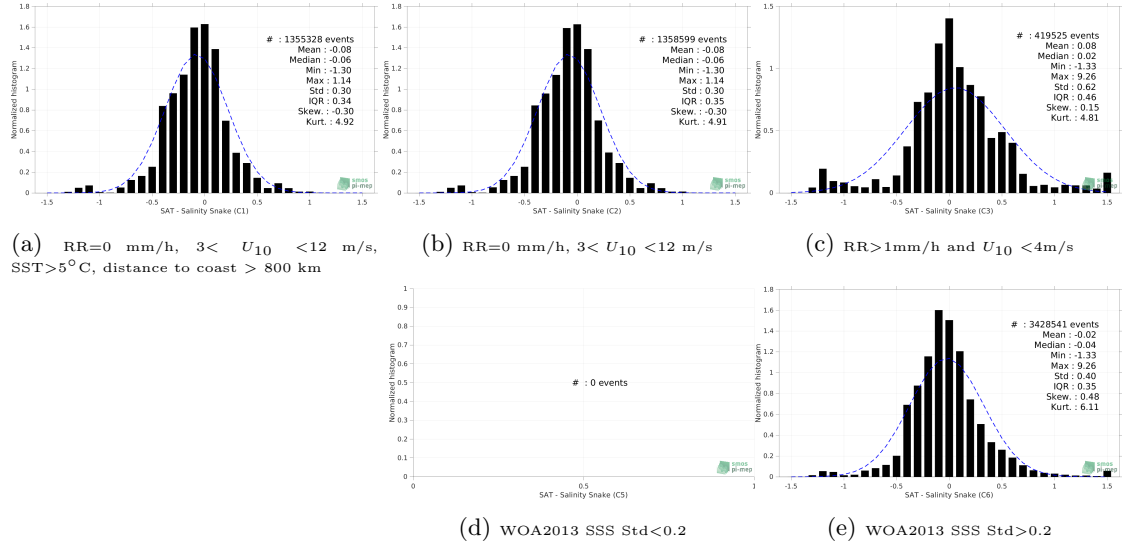
Figure 12: Normalized histogram of \Delta SSS (SMAP SSS L3 v4 - Monthly (RSS) - Salinity Snake) for 5 different subdatasets corresponding to: RR=0 mm/h, 3 < U_{10} < 12 m/s, SST > 5°C, distance to coast > 800 km (a), RR=0 mm/h, 3 < U_{10} < 12 m/s (b), RR > 1mm/h and U_{10} < 4 m/s (c), WOA2013 SSS Std < 0.2 (d), WOA2013 SSS Std > 0.2 (e).
