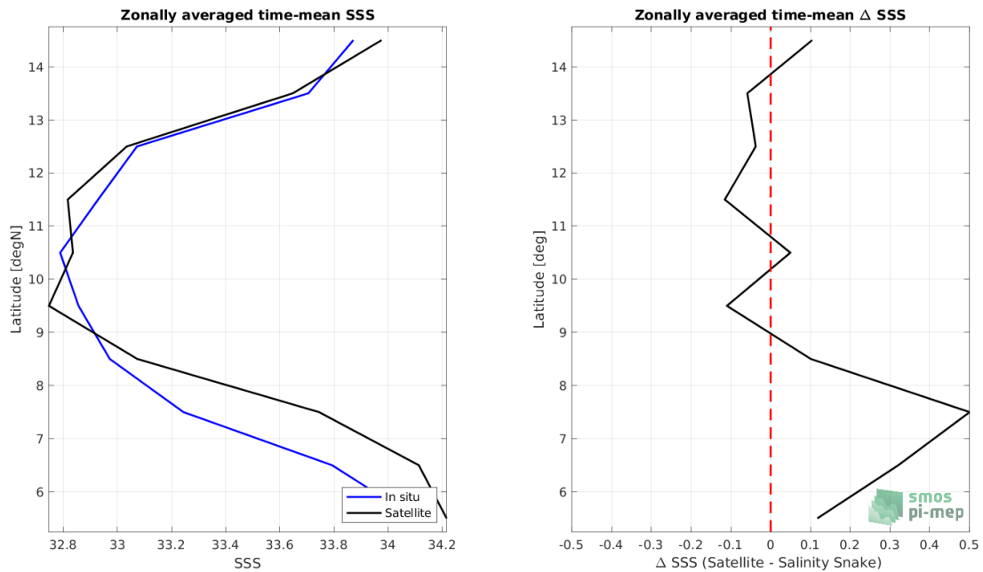
Figure 7: Left panel: Zonal mean SSS from SMAP SSS L3 v4 - Monthly (RSS) satellite product (black) and from Salinity Snake (blue). Right panel: Zonal mean of \Delta SSS (Satellite - Salinity Snake) for all the collected Pi-MEP match-up pairs estimated over the full satellite product period.
