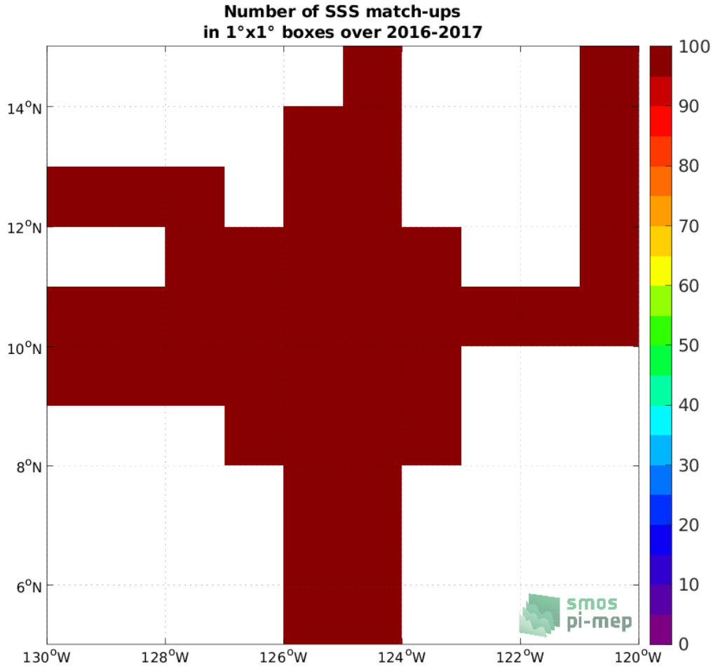
Figure 3: Number of SSS match-ups between Salinity Snake SSS and the SMAP SSS L3 v4 - Monthly (RSS) SSS product for the SPURS 2 Pi-MEP region over 1^\circ \times 1^\circ boxes and for the full satellite product period.
