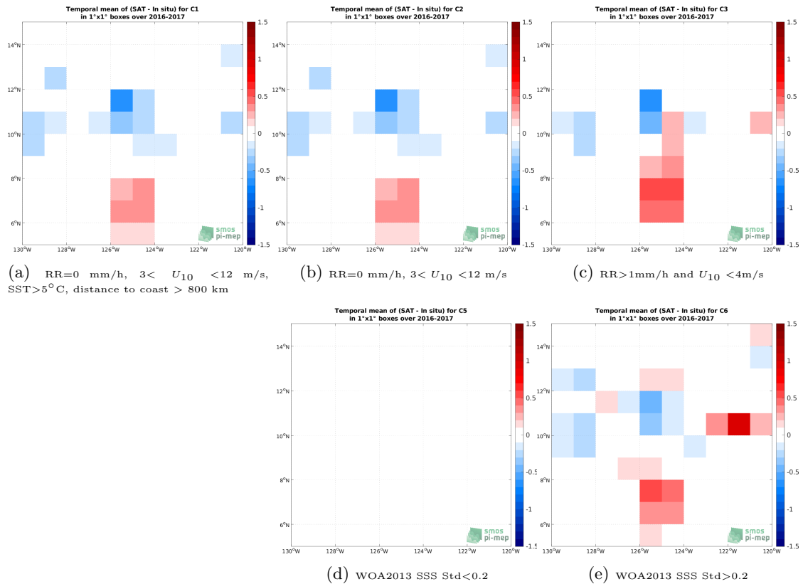
Figure 11: Temporal mean gridded over spatial boxes of size 1^\circ \times 1^\circ of \Delta SSS (SMAP SSS L3 v4 - Monthly (RSS) - Salinity Snake) for 5 different subdatasets corresponding to:RR=0 mm/h, 3 < U_{10} < 12 m/s, SST >5^\circ\text{C} , distance to coast > 800 km (a), RR=0 mm/h, 3 < U_{10} < 12 m/s (b), RR >1 mm/h and U_{10} < 4 m/s (c), WOA2013 SSS Std <0.2 (d), WOA2013 SSS Std >0.2 (e).
