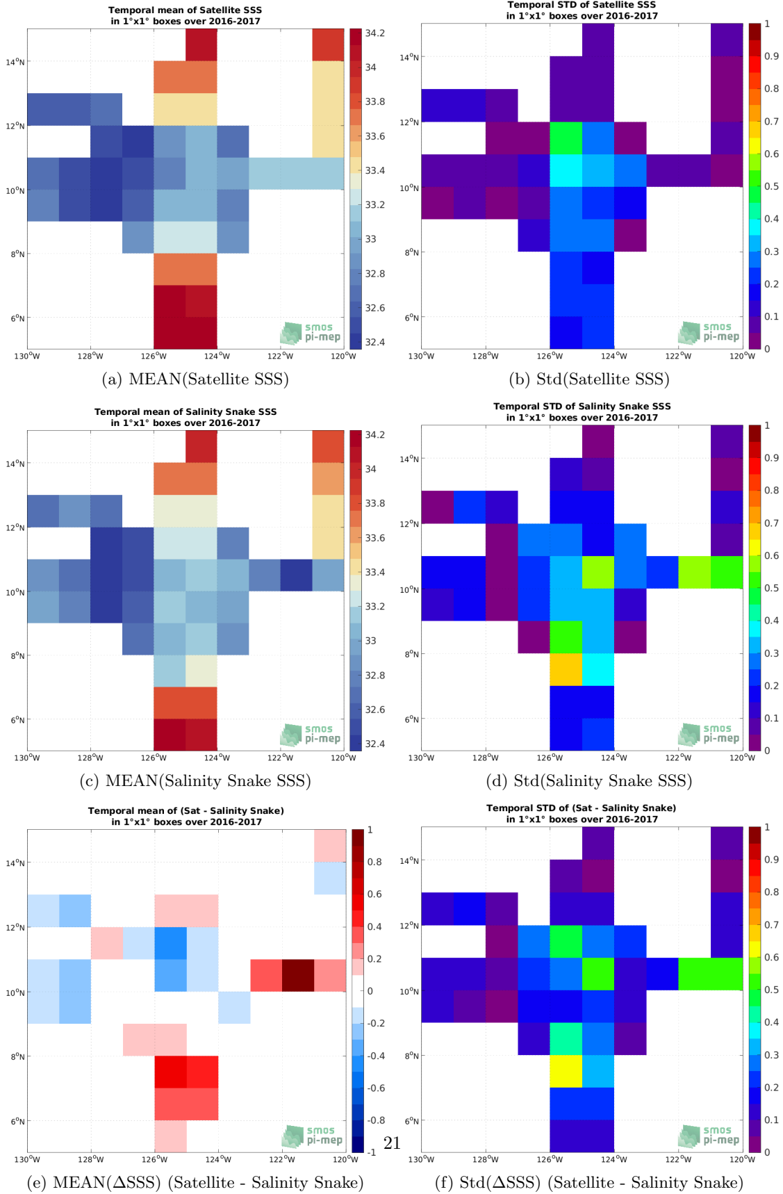
Figure 5: Temporal mean (left) and Std (right) of SSS from SMAP SSS L3 v4 - Monthly (RSS) (top), Salinity Snake (middle), and of \Delta SSS (Satellite - Salinity Snake). Only match-up pairs are used to generate these maps.
