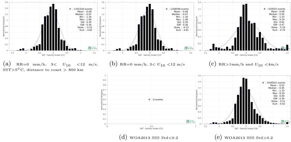
Figure 12: Normalized histogram of \Delta SSS (SMAP SSS L3 v4 - Monthly (RSS) - Salinity Snake) for 5 different subdatasets corresponding to: RR=0 mm/h, 3 < U_{10} < 12 m/s, SST>5°C, distance to coast > 800 km (a), RR=0 mm/h, 3 < U_{10} < 12 m/s (b), RR>1mm/h and U_{10} < 4 m/s (c), WOA2013 SSS Std<0.2 (d), WOA2013 SSS Std>0.2 (e).
