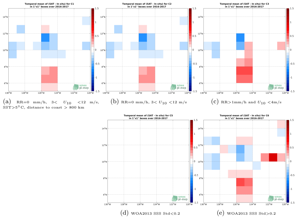
Figure 11: Temporal mean gridded over spatial boxes of size 1°x1° of \Delta SSS (SMAP SSS L3 v4 - Monthly (RSS) - Salinity Snake) for 5 different subdatasets corresponding to:RR=0 mm/h, 3 < U_{10} < 12 m/s, SST>5°C, distance to coast > 800 km (a), RR=0 mm/h, 3 < U_{10} < 12 m/s (b), RR>1mm/h and U_{10} < 4 m/s (c), WOA2013 SSS Std<0.2 (d), WOA2013 SSS Std>0.2 (e).
