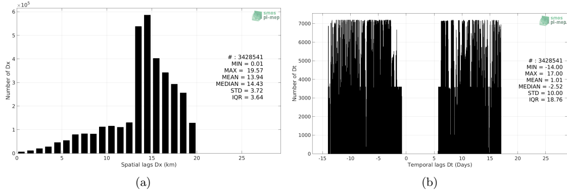
Figure 5: Histograms of the spatial (a) and temporal (b) lags between the time of the Salinity Snake measurements and the date of the corresponding SMAP SSS L3 v4 - Monthly (RSS) SSS product.
