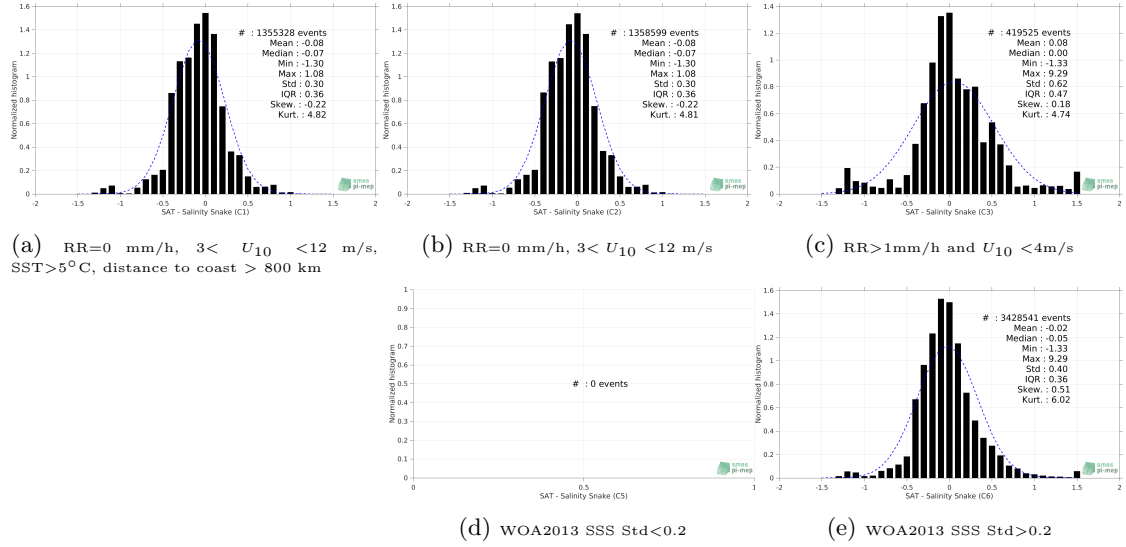
Figure 13: Normalized histogram of \Delta SSS (SMAP SSS L3 v4 - Monthly (RSS) - Salinity Snake) for 5 different subdatasets corresponding to: RR=0 mm/h, 3 < U_{10} < 12 m/s, SST>5°C, distance to coast > 800 km (a), RR=0 mm/h, 3 < U_{10} < 12 m/s (b), RR>1mm/h and U_{10} < 4 m/s (c), WOA2013 SSS Std<0.2 (d), WOA2013 SSS Std>0.2 (e).
