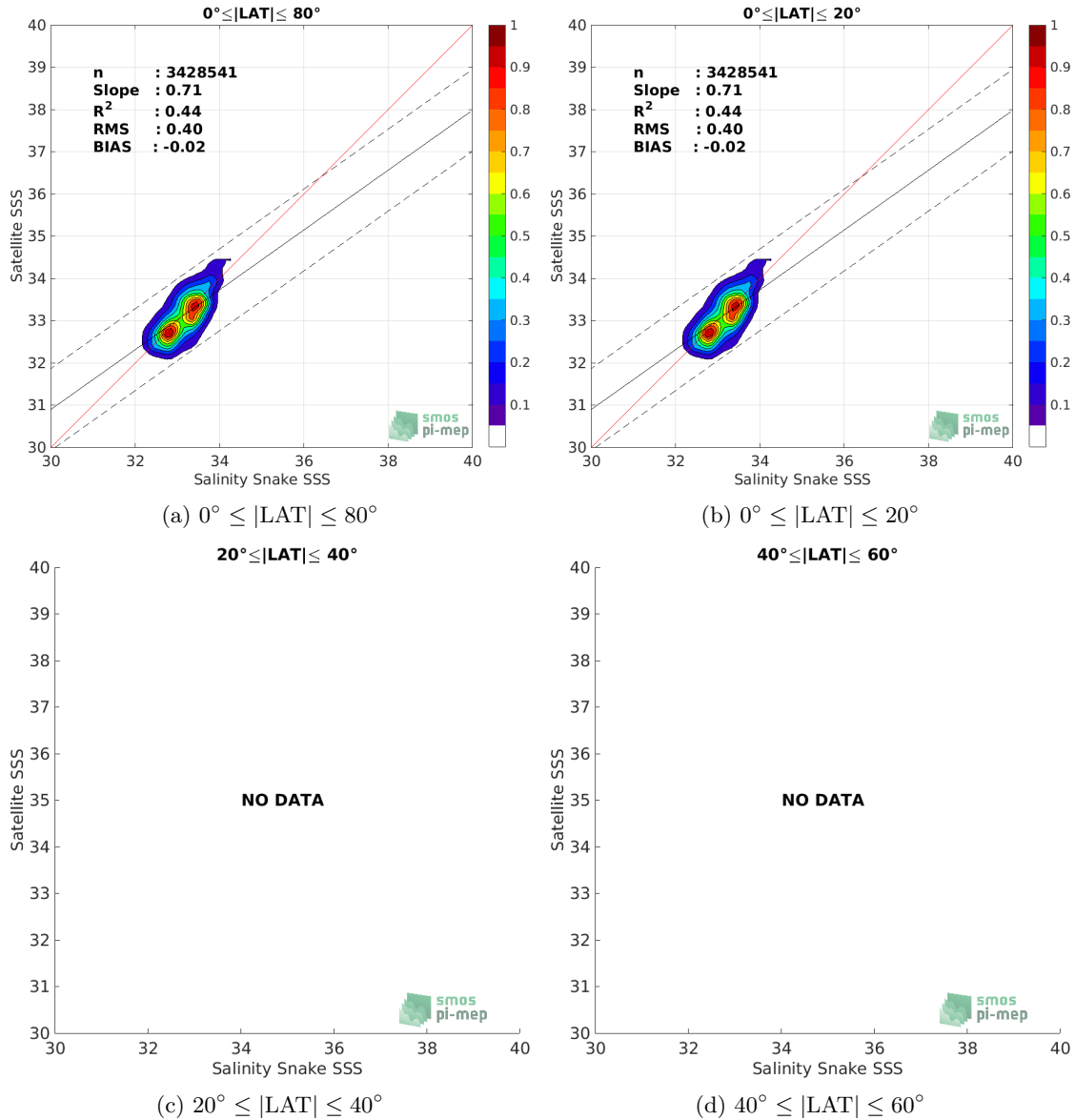
Figure 9: Contour maps of the concentration of SMAP SSS L3 v4 - Monthly (RSS) SSS (y-axis) versus Salinity Snake SSS (x-axis) at match-up pairs for different latitude bands. For each plot, the red line shows x=y . The black thin and dashed lines indicate a linear fit through the data cloud and the \pm 95\% confidence levels, respectively. The number match-up pairs n , the slope and R^2 coefficient of the linear fit, the root mean square (RMS) and the mean bias between satellite and in situ data are indicated for each latitude band in each plots.
