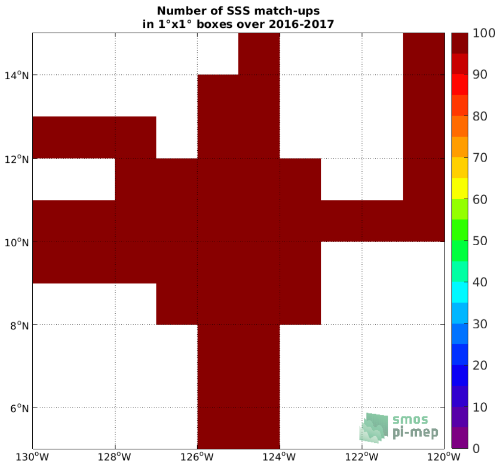
Figure 4: Number of SSS match-ups between Salinity Snake SSS and the SMAP SSS L3 v4 - Monthly (RSS) SSS product for the SPURS 2 Pi-MEP region over 1°x1° boxes and for the full satellite product period.
