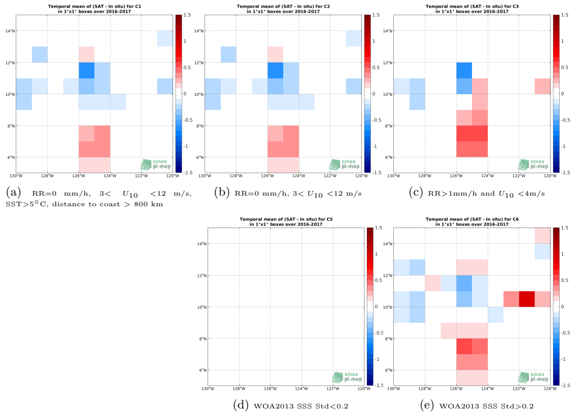
Figure 12: Temporal mean gridded over spatial boxes of size 1°x1° of \Delta SSS (SMAP SSS L3 v4 - Monthly (RSS) - Salinity Snake) for 5 different subdatasets corresponding to:RR=0 mm/h, 3 < U_{10} < 12 m/s, SST>5°C, distance to coast > 800 km (a), RR=0 mm/h, 3 < U_{10} < 12 m/s (b), RR>1mm/h and U_{10} < 4 m/s (c), WOA2013 SSS Std<0.2 (d), WOA2013 SSS Std>0.2 (e).
