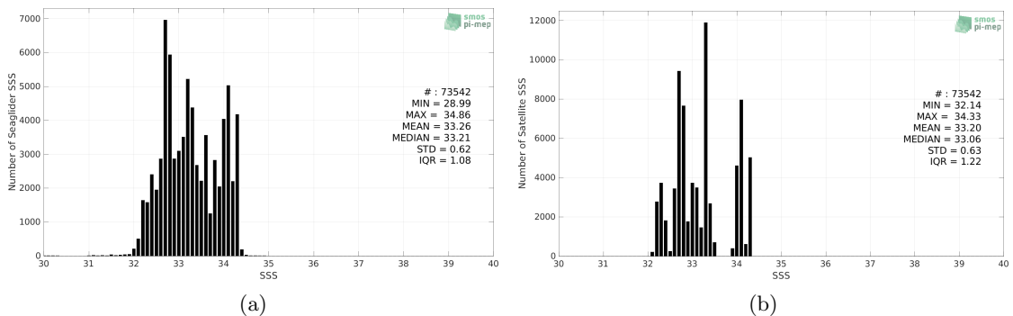
Figure 2: Histograms of SSS from Seagliders (a) and SMAP SSS L3 v4 - Monthly (RSS) (b) considering all match-up pairs per bins of 0.1 over the SPURS 2 Pi-MEP region and for the full satellite product period.
