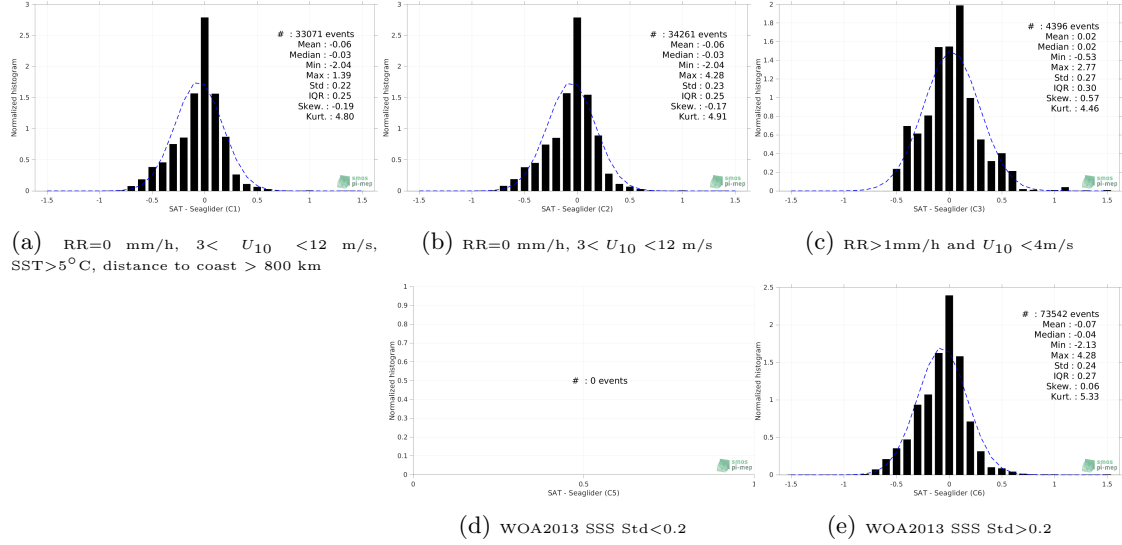
Figure 12: Normalized histogram of \Delta SSS (SMAP SSS L3 v4 - Monthly (RSS) - Seaglider) for 5 different subdatasets corresponding to: RR=0 mm/h, 3 < U_{10} < 12 m/s, SST > 5°C, distance to coast > 800 km (a), RR=0 mm/h, 3 < U_{10} < 12 m/s (b), RR > 1mm/h and U_{10} < 4 m/s (c), WOA2013 SSS Std < 0.2 (d), WOA2013 SSS Std > 0.2 (e).
