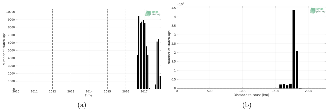
Figure 1: Number of match-ups between Seagliders and SMAP SSS L3 v4 - Monthly (RSS) SSS as a function of time (a) and as function of the distance to coast (b) over the SPURS 2 Pi-MEP region and for the full satellite product period.
