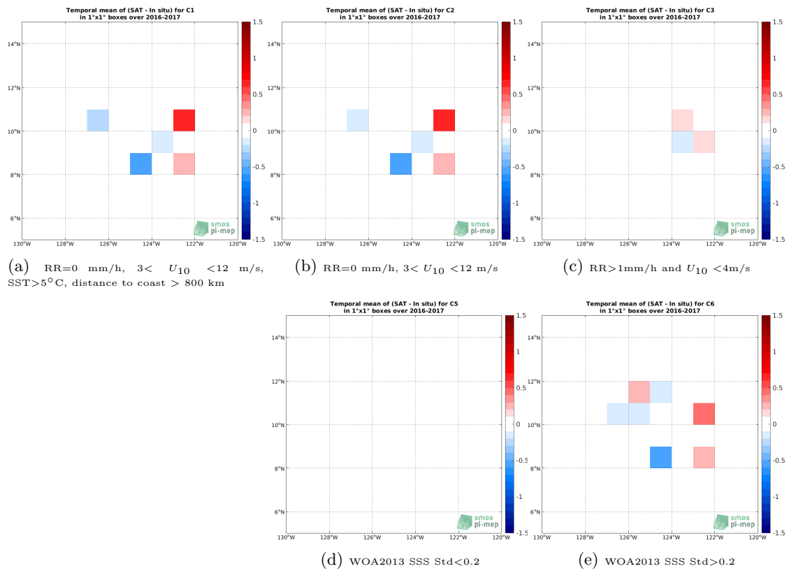
Figure 12: Temporal mean gridded over spatial boxes of size 1^\circ \times 1^\circ of \Delta SSS (SMAP SSS L3 v4 - Monthly (RSS) - Seaglider) for 5 different subdatasets corresponding to: RR=0 mm/h, 3 < U_{10} < 12 m/s, SST > 5^\circ C , distance to coast > 800 km (a), RR=0 mm/h, 3 < U_{10} < 12 m/s (b), RR > 1 mm/h and U_{10} < 4 m/s (c), WOA2013 SSS Std < 0.2 (d), WOA2013 SSS Std > 0.2 (e).
