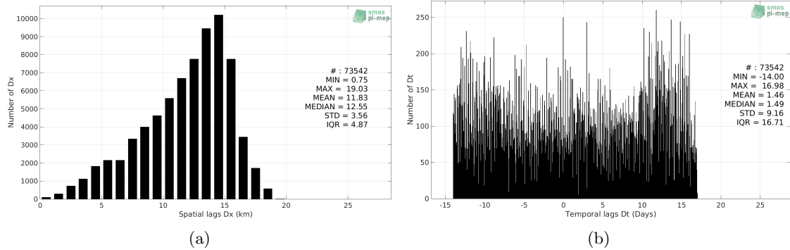
Figure 5: Histograms of the spatial (a) and temporal (b) lags between the time of the Seaglider measurements and the date of the corresponding SMAP SSS L3 v4 - Monthly (RSS) SSS product.
