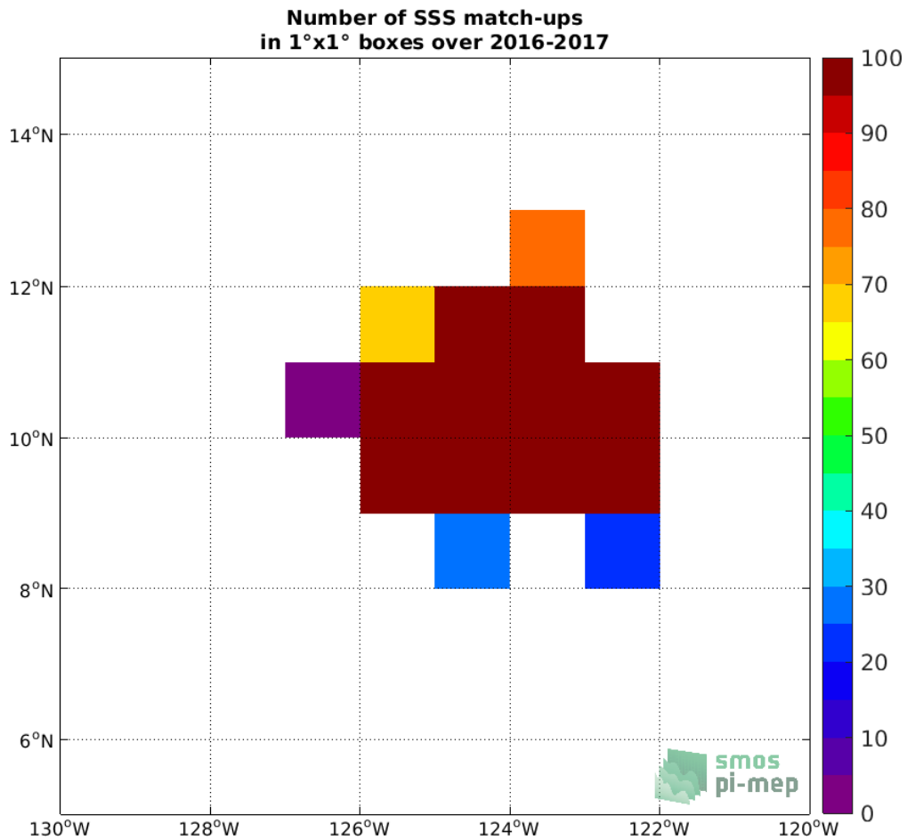
Figure 4: Number of SSS match-ups between Seagliders SSS and the SMAP SSS L3 v4 - Monthly (RSS) SSS product for the SPURS 2 Pi-MEP region over 1°x1° boxes and for the full satellite product period.
