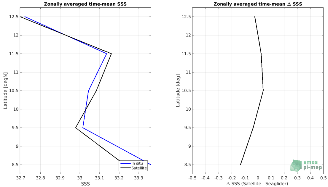
Figure 8: Left panel: Zonal mean SSS from SMAP SSS L3 v4 - Monthly (RSS) satellite product (black) and from Seaglider (blue). Right panel: Zonal mean of \Delta SSS (Satellite - Seaglider) for all the collected Pi-MEP match-up pairs estimated over the full satellite product period.
