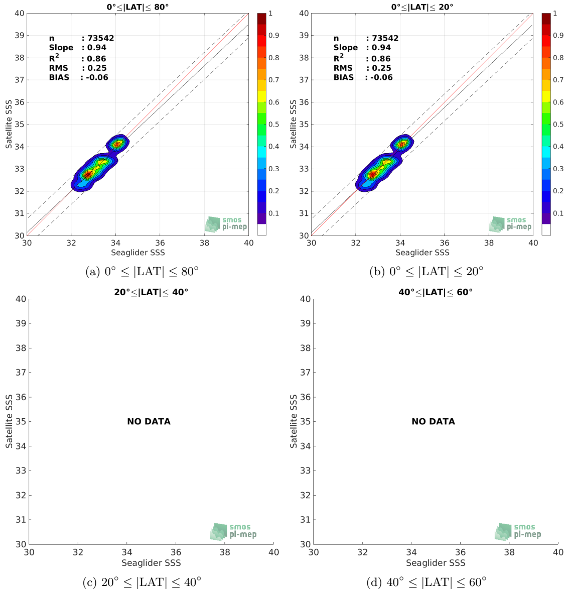
Figure 9: Contour maps of the concentration of SMAP SSS L3 v4 - Monthly (RSS) SSS (y-axis) versus Seaglider SSS (x-axis) at match-up pairs for different latitude bands. For each plot, the red line shows x=y . The black thin and dashed lines indicate a linear fit through the data cloud and the \pm 95\% confidence levels, respectively. The number match-up pairs n , the slope and R^2 coefficient of the linear fit, the root mean square (RMS) and the mean bias between satellite and in situ data are indicated for each latitude band in each plots.
