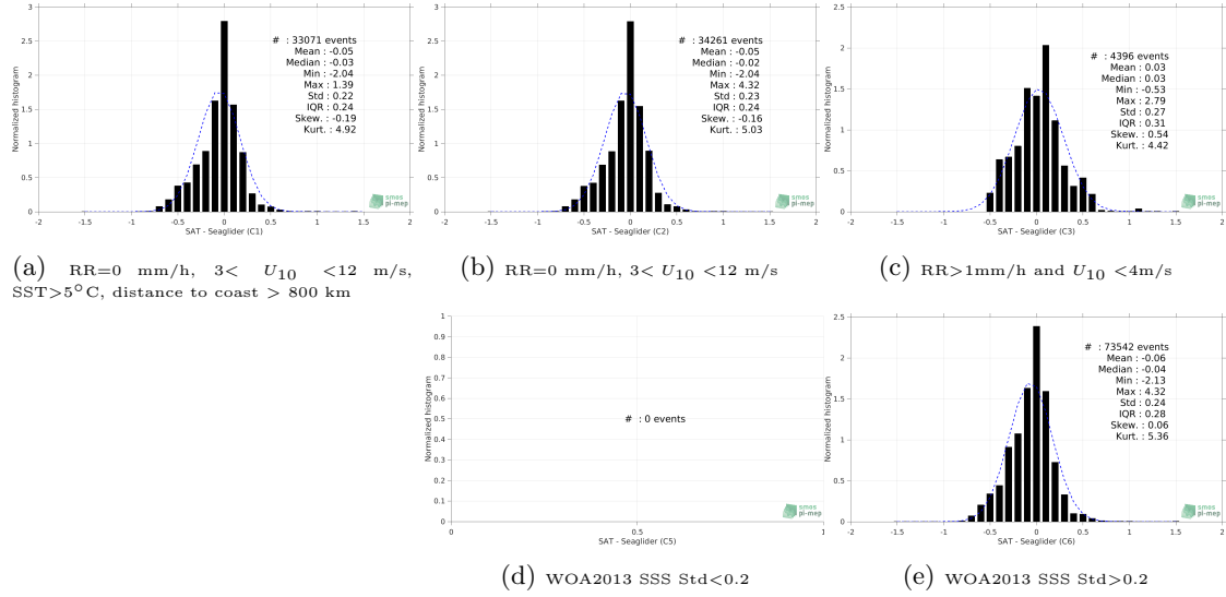
Figure 13: Normalized histogram of \Delta SSS (SMAP SSS L3 v4 - Monthly (RSS) - Seaglider) for 5 different subdatasets corresponding to: RR=0 mm/h, 3 < U_{10} < 12 m/s, SST>5°C, distance to coast > 800 km (a), RR=0 mm/h, 3 < U_{10} < 12 m/s (b), RR>1mm/h and U_{10} < 4 m/s (c), WOA2013 SSS Std<0.2 (d), WOA2013 SSS Std>0.2 (e).
