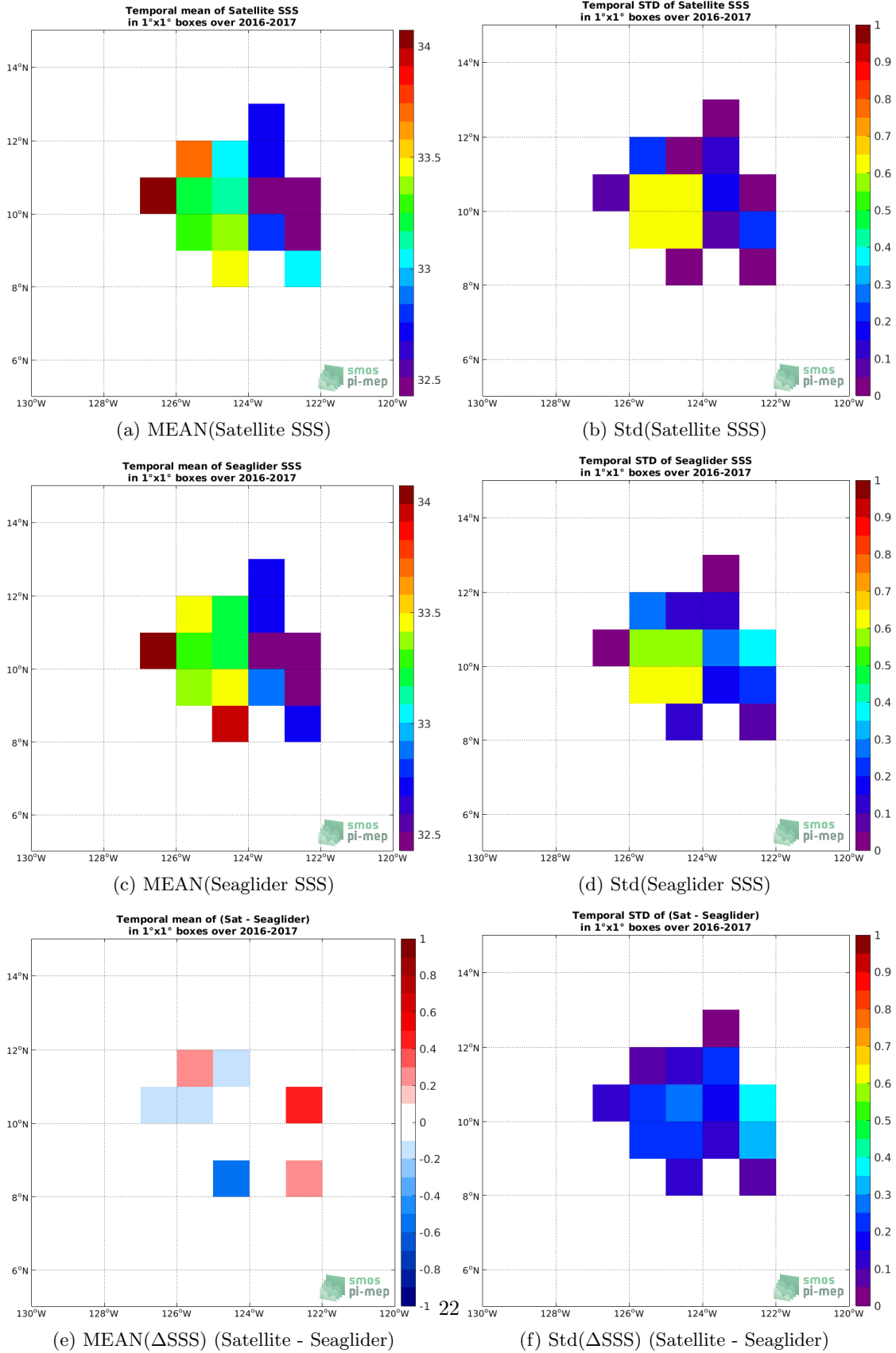
Figure 6: Temporal mean (left) and Std (right) of SSS from SMAP SSS L3 v4 - Monthly (RSS) (top), Seaglider (middle), and of \Delta SSS (Satellite - Seaglider). Only match-up pairs are used to generate these maps.
