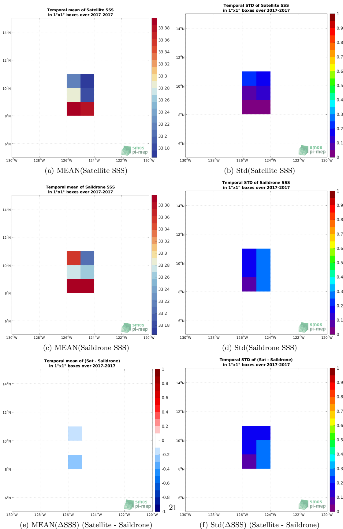
Figure 5: Temporal mean (left) and Std (right) of SSS from SMAP SSS L3 v4 - Monthly (RSS) (top), Saildrone (middle), and of \Delta SSS (Satellite - Saildrone). Only match-up pairs are used to generate these maps.
