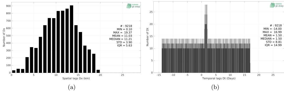
Figure 4: Histograms of the spatial (a) and temporal (b) lags between the location/time of the Sailldrone measurement and the date of the corresponding SMAP SSS L3 v4 - Monthly (RSS) SSS pixel.
