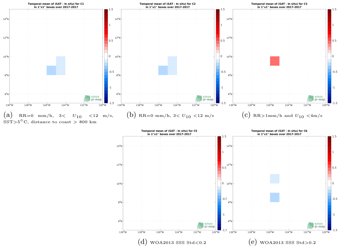
Figure 11: Temporal mean gridded over spatial boxes of size 1^\circ \times 1^\circ of \Delta SSS (SMAP SSS L3 v4 - Monthly (RSS) - Sairdrone) for 5 different subdatasets corresponding to:RR=0 mm/h, 3 < U_{10} < 12 m/s, SST >5^\circ C, distance to coast > 800 km (a), RR=0 mm/h, 3 < U_{10} < 12 m/s (b), RR >1 mm/h and U_{10} < 4 m/s (c), WOA2013 SSS Std <0.2 (d), WOA2013 SSS Std >0.2 (e).
