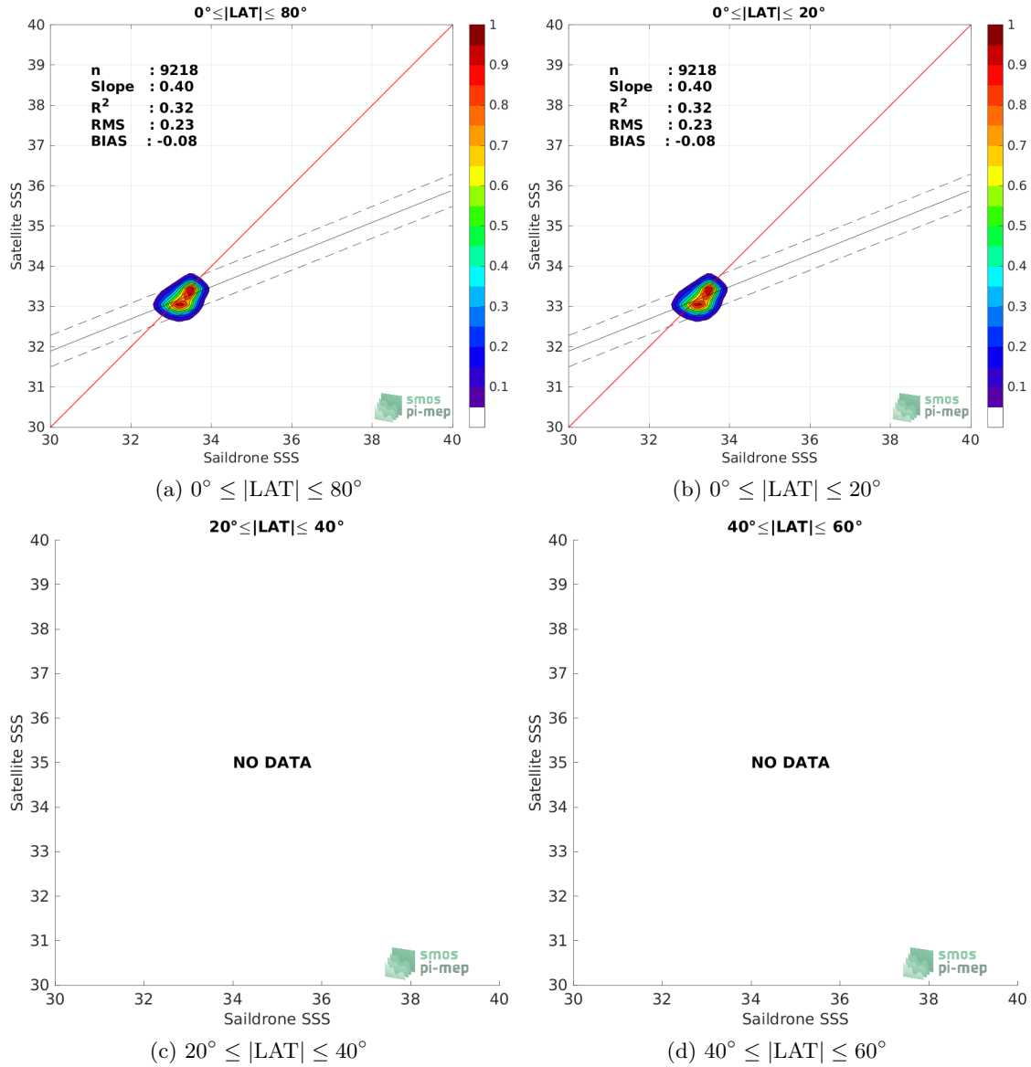
Figure 8: Contour maps of the concentration of SMAP SSS L3 v4 - Monthly (RSS) SSS (y-axis) versus Sailability SSS (x-axis) at match-up pairs for different latitude bands. For each plot, the red line shows x=y . The black thin and dashed lines indicate a linear fit through the data cloud and the \pm 95\% confidence levels, respectively. The number match-up pairs n , the slope and R^2 coefficient of the linear fit, the root mean square (RMS) and the mean bias between satellite and in situ data are indicated for each latitude band in each plots.
